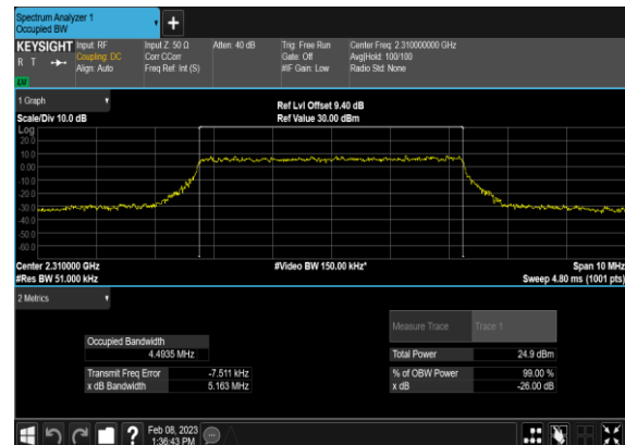
N30(5M)_CP-OFDM_16 QAM_Outer_Full_Mid_CH
