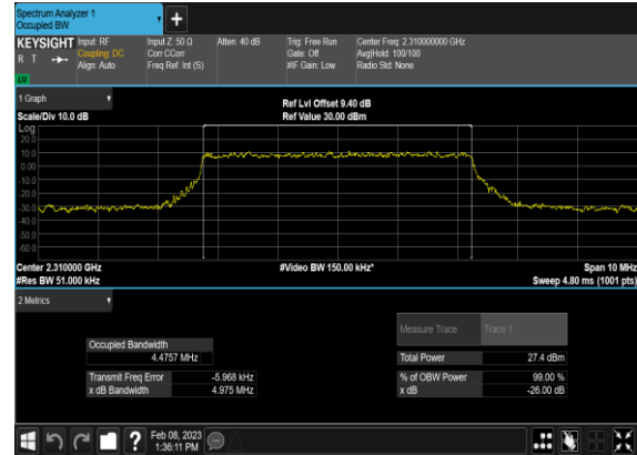
N30(5M)_DFT-s-OFDM_QPSK_Outer_Full_ Mid_CH
