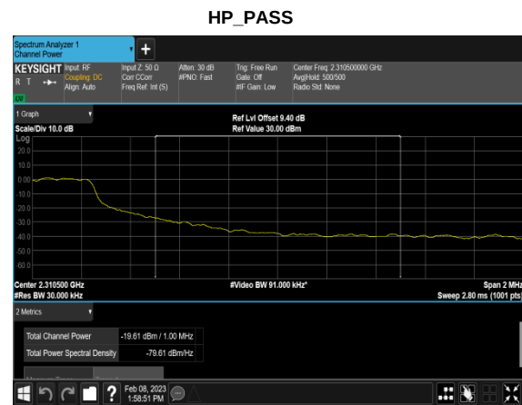
N30(5M)_DFT-s-OFDM_QPSK_Outer_Full_Low_CH_c
