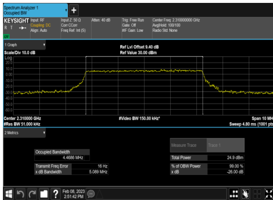
N30(5M)_CP-OFDM_QPSK_Outer_Full_Mid_CH
