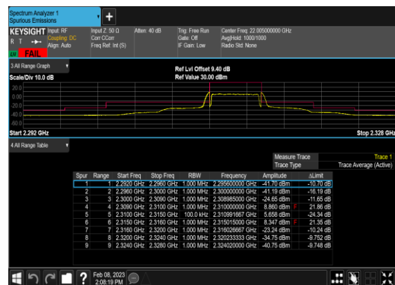
N30(5M)_DFT-s-OFDM_QPSK_Outer_Full_High_CH
