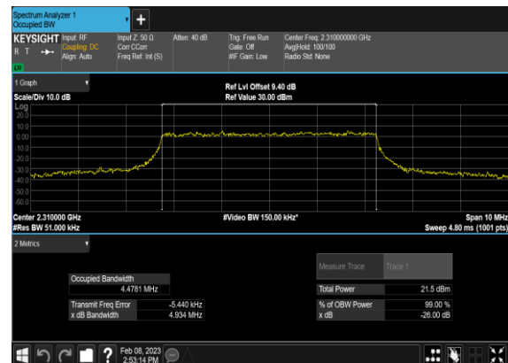
N30(5M)_CP-OFDM_256 QAM_Outer_Full_Mid_CH
