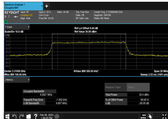
N30(10M)_CP-OFDM_16 QAM_Outer_Full_Low_CH
