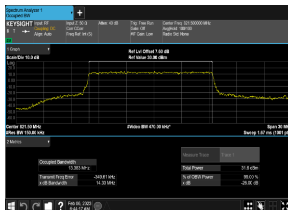
N26(15M)_DFT-s-OFDM_QPSK_Outer_Full_Mid_CH
