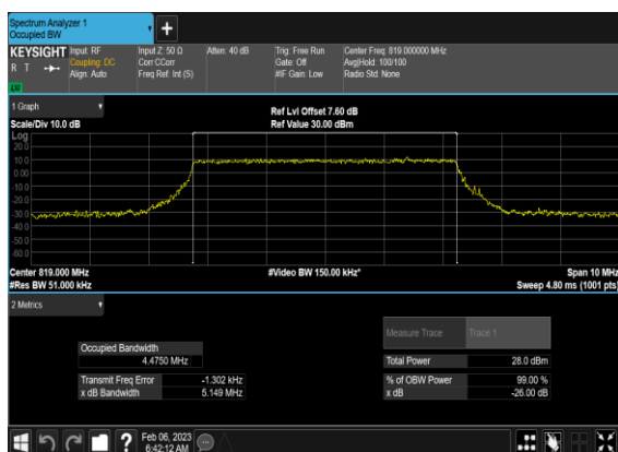
N26(5M)_CP-OFDM_QPSK_Outer_Full_Mid_CH
