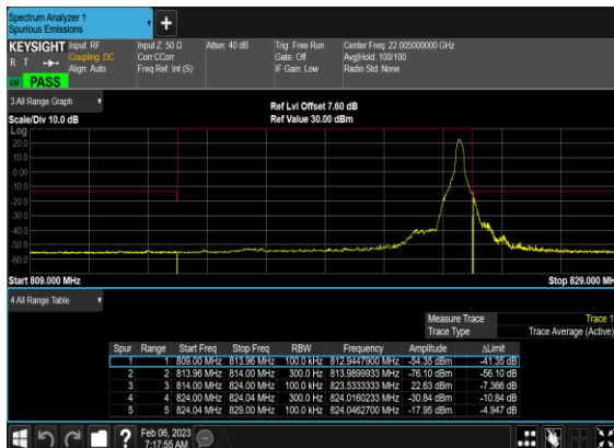
N26(10M)_DFT-s-OFDM_BPSK_Edge_1RB_Right_Mid_CH
