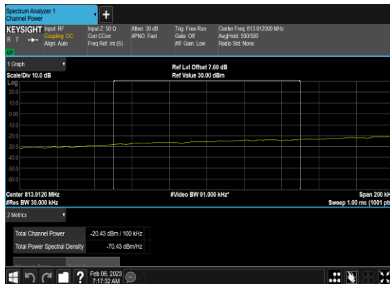
N26(10M)_DFT-s-OFDM_QPSK_Edge_1RB_Left_Mid_CH_CHP_PASS
