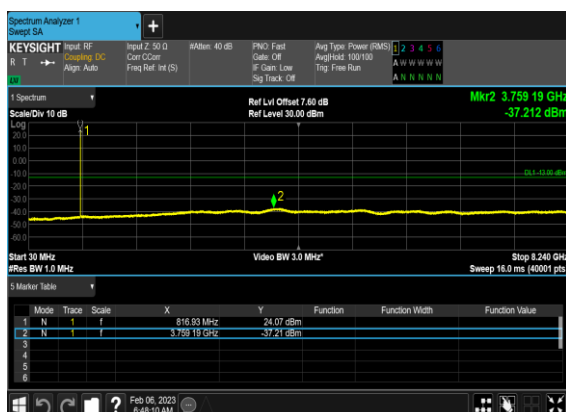
N26(5M)_DFT-s-OFDM_BPSK_Edge_1RB_Left_Mid_CH
