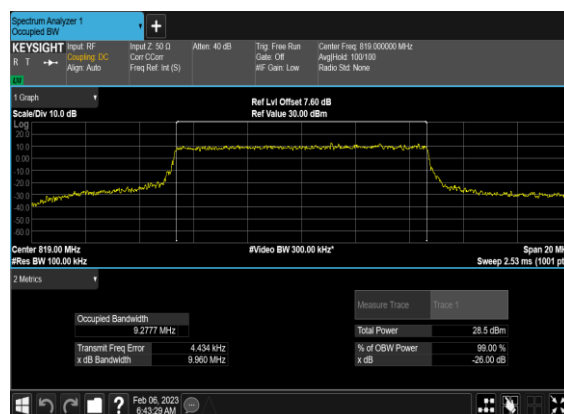
N26(10M)_CP-OFDM_16 QAM_Outer_Full_Mid_CH
