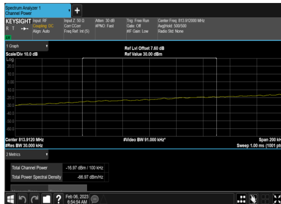
N26(5M)_DFT-s-OFDM_BPSK_Edge_1RB_Left_Low_CH_CHP_PASS
