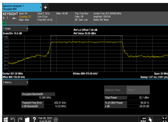
N26(15M)_DFT-s-OFDM_PI_2-BPSK_Outer_Full_Mid_CH
