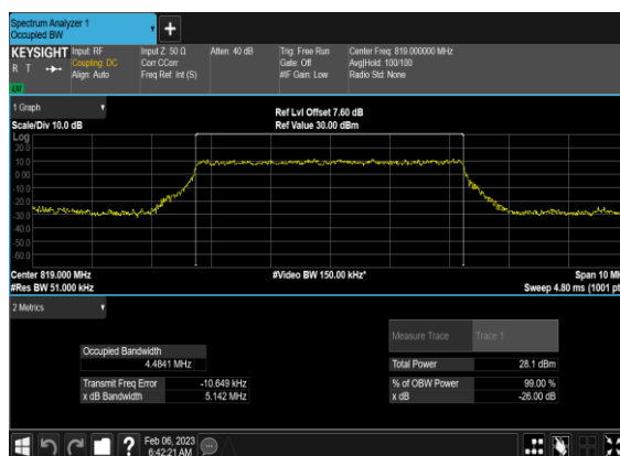
N26(5M)_CP-OFDM_16QAM_Outer_Full_Mid_CH
