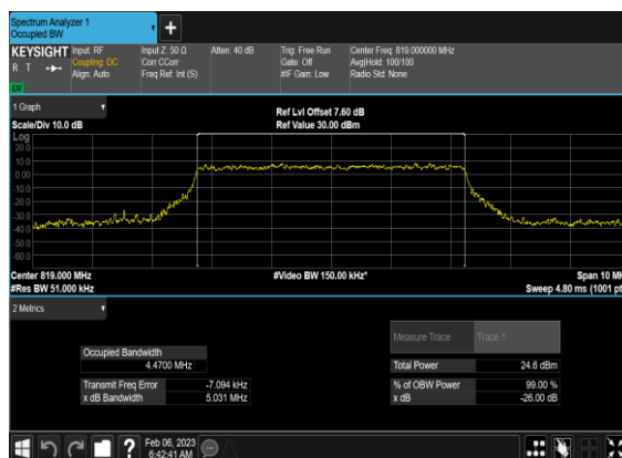
N26(5M)_CP-OFDM_256 QAM_Outer_Full_Mid_CH
