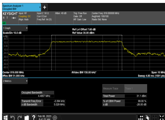
N26(5M)_DFT-s-OFDM_PI_2-BPSK_Outer_Full_Mid_CH
