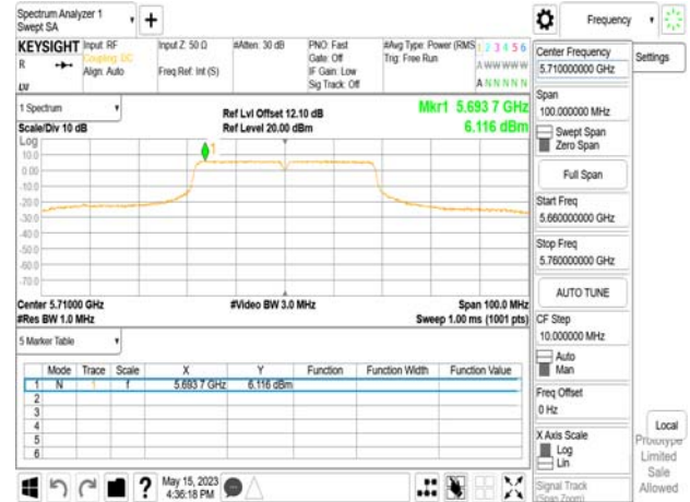
802.11n_40MHz_Chain0_5710MHz_UNII 3
