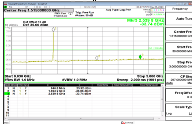
HSDPA_B5_HighCH4233-846.6
