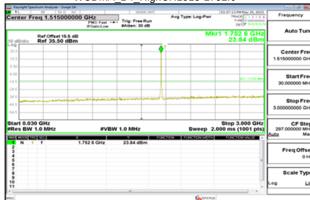
WCDMA B4_HighCH1513-1752.6
