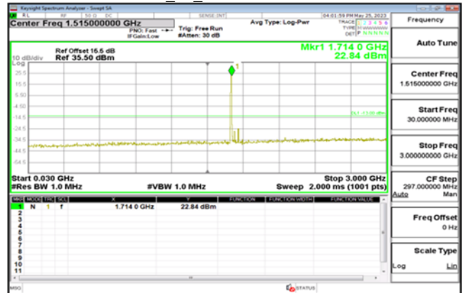
HSUPA B4 MidCH1413-1732.6
