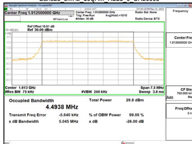
Band25 5MHz 16QAM RB25 0 CH26665
