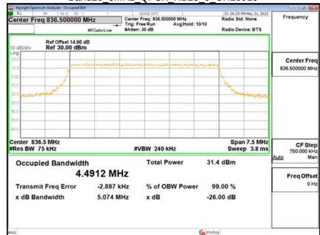
Band26 5MHz QPSK RB25 0 CH26915
