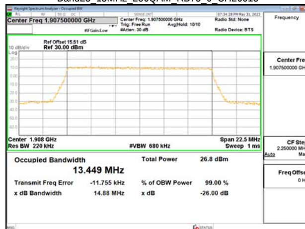
Band25 15MHz 256QAM RB75 0 CH26615
