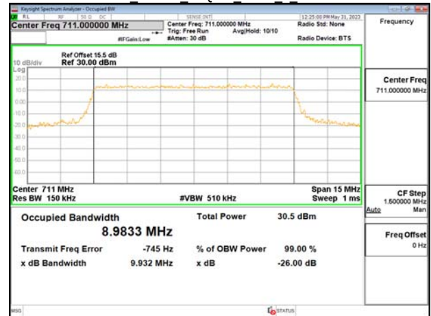
Band17 10MHz 16QAM RB50 0 CH23800
