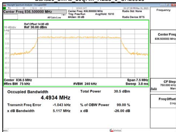
Band26 5MHz 16QAM RB25 0 CH26915
