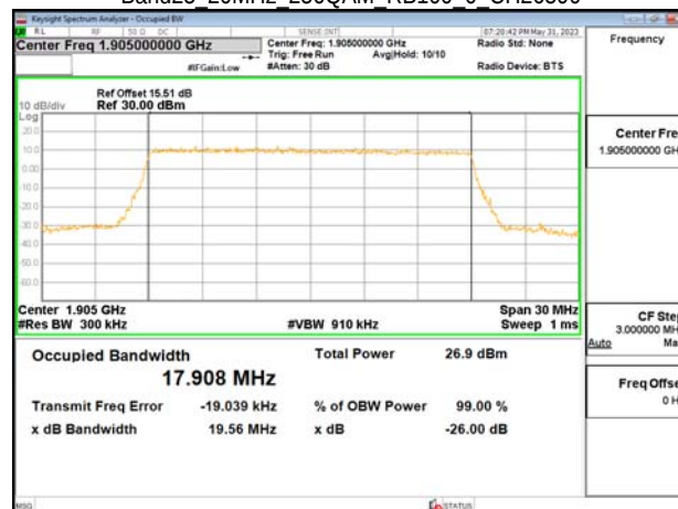
Band25 20MHz 256QAM RB100 0 CH26590
