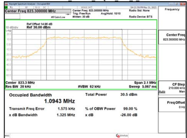
Band26-Part90s 1.4MHz 16QAM RB6 0 CH26783
