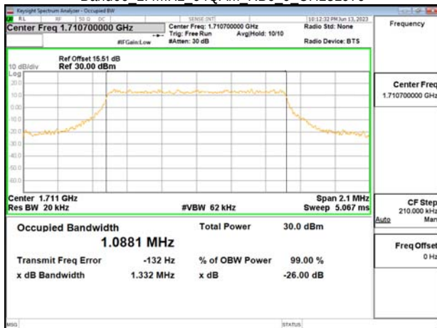
Band66 1.4MHz 64QAM RB6 0 CH131979
