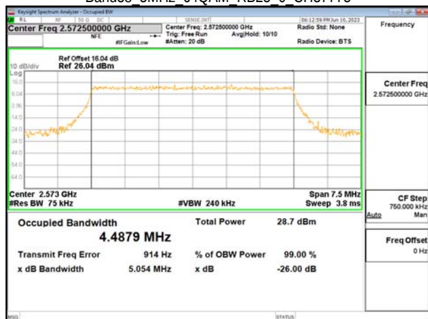
Band38 5MHz 64QAM RB25 0 CH37775
