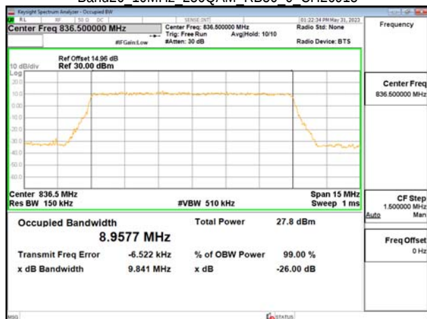
Band26 10MHz 256QAM RB50 0 CH26915
