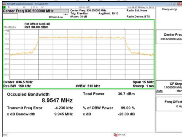
Band26 10MHz 16QAM RB50 0 CH26915
