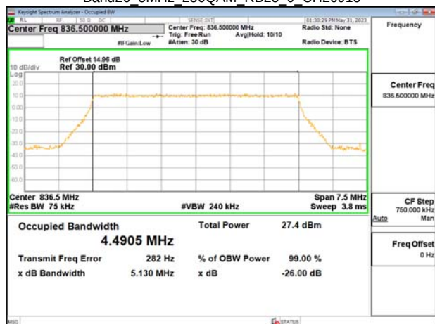
Band26 5MHz 256QAM RB25 0 CH26915
