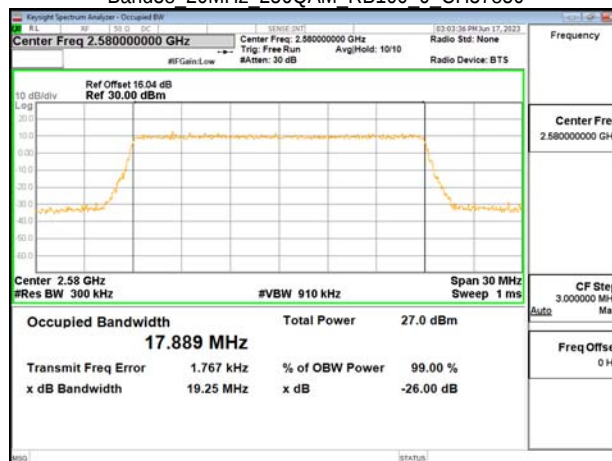
Band38 20MHz 256QAM RB100 0 CH37850
