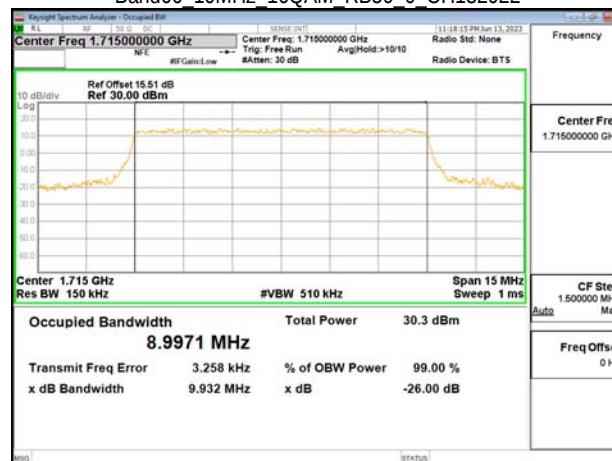
Band66 10MHz 16QAM RB50 0 CH132022
