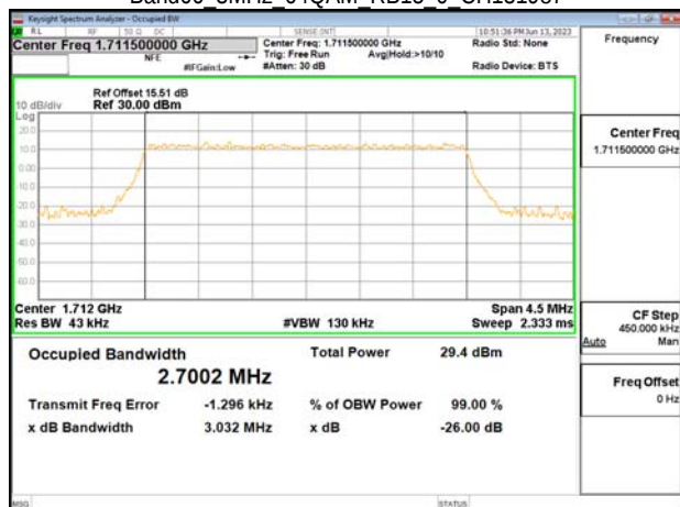
Band66 3MHz 64QAM RB15 0 CH131987
