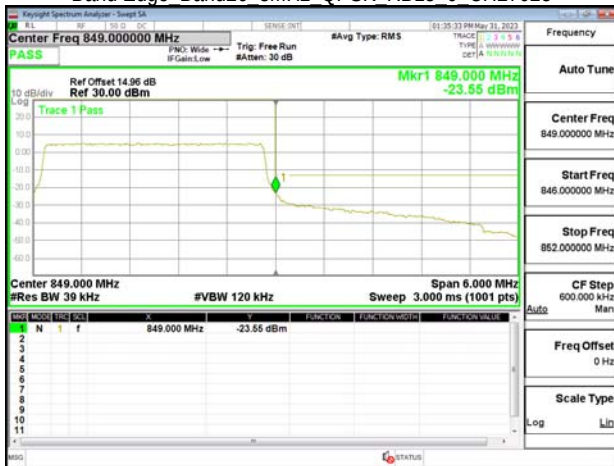
Band Edge Band26 5MHz QPSK RB1 0 CH26815
