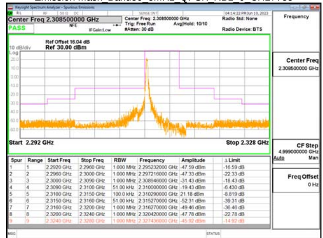
Emission Mask Band30 5MHz QPSK RB1 24 CH27685
