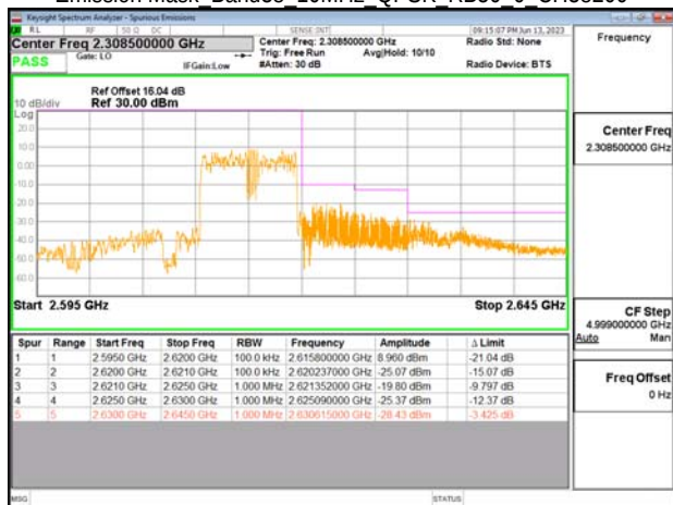
Emission Mask Band38 10MHz QPSK RB50 0 CH38200
