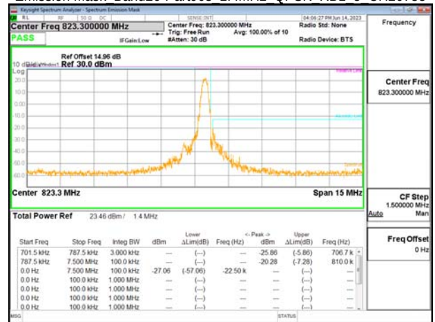
Emission Mask Band26-Part90s 1.4MHz QPSK RB6 0 CH26697
