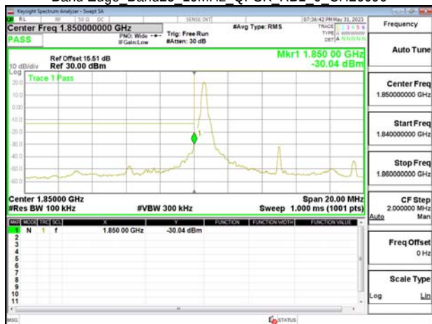
Band Edge Band25 10MHz QPSK RB1 0 CH26090
