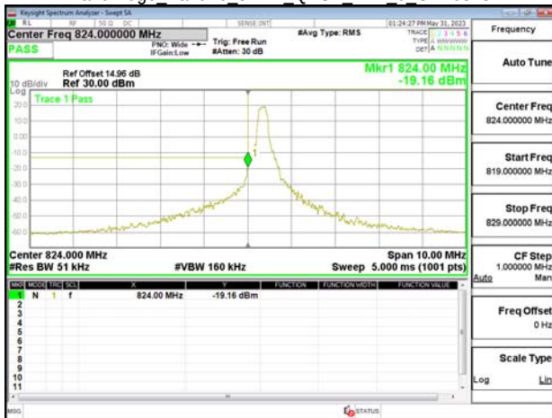
Band Edge Band26 5MHz QPSK RB1 24 CH27015
