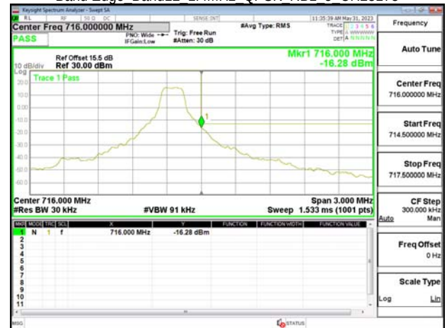
Band Edge Band12 1.4MHz QPSK RB6 0 CH23017
