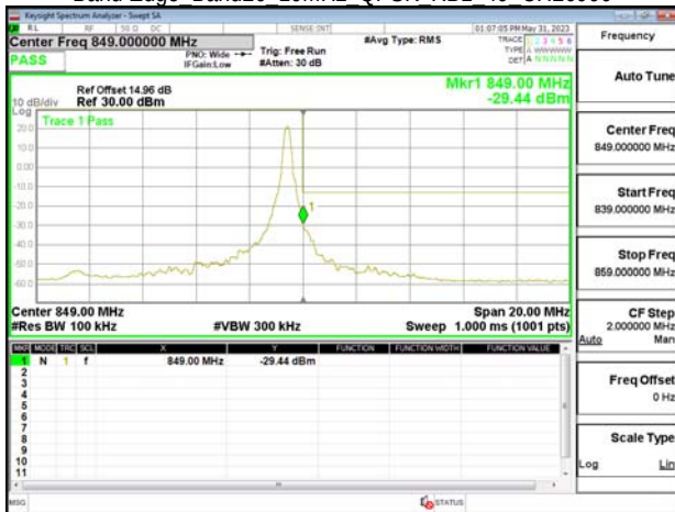
Band Edge Band26 10MHz QPSK RB50 0 CH26840
