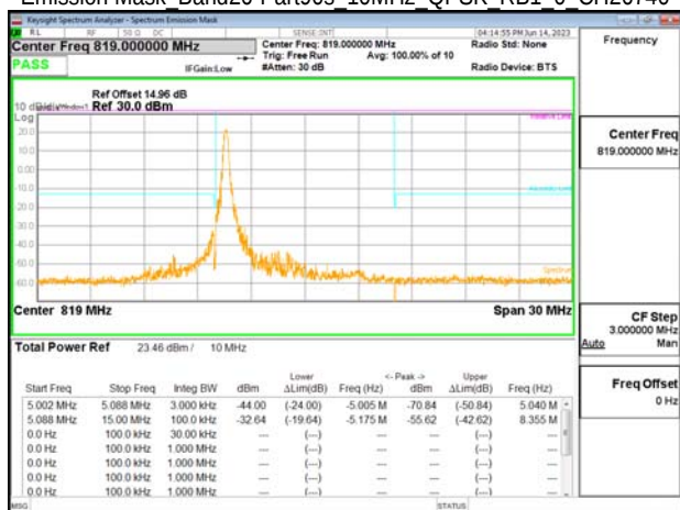
Emission Mask Band26-Part90s 10MHz QPSK RB1 0 CH26740
