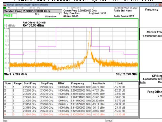
Emission Mask Band30 10MHz QPSK RB1 49 CH27710
