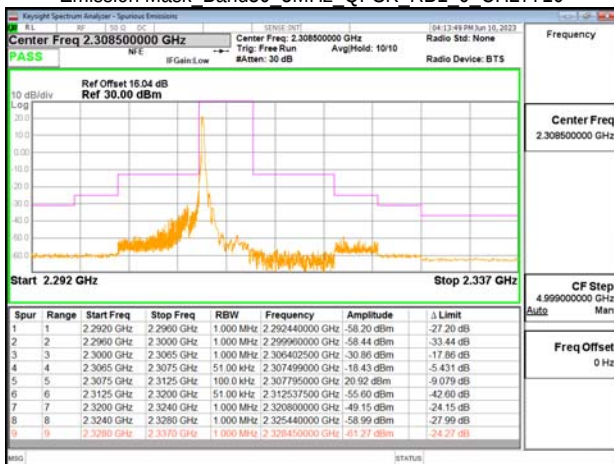
Emission Mask Band30 5MHz QPSK RB1 0 CH27710
