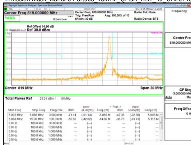
Emission Mask Band26-Part90s 10MHz QPSK RB50 0 CH26740
