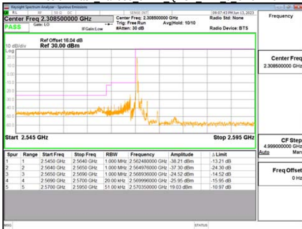
Emission Mask Band38 5MHz QPSK RB1 24 CH38225
