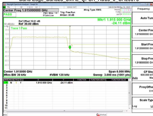
Band Edge Band25 5MHz QPSK RB1 0 CH26065
