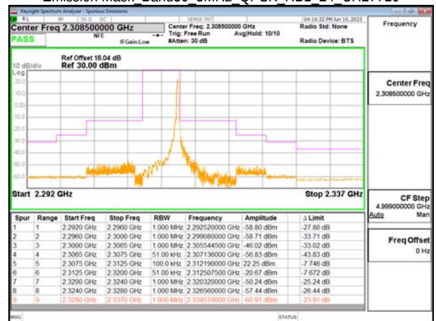
Emission Mask Band30 5MHz QPSK RB1 24 CH27710
