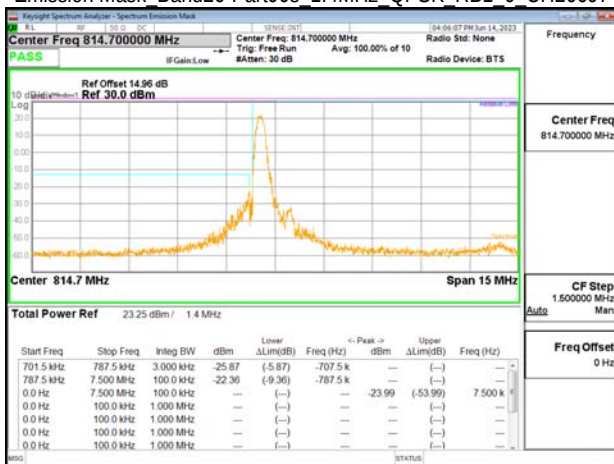
Emission Mask Band26-Part90s 1.4MHz QPSK RB1 0 CH26697
