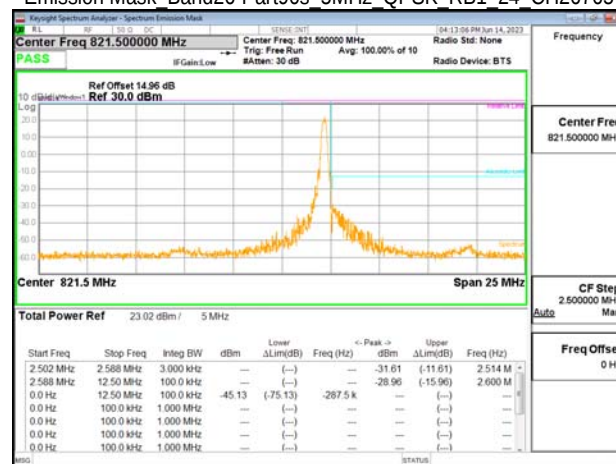
Emission Mask Band26-Part90s 5MHz QPSK RB1 24 CH26765
