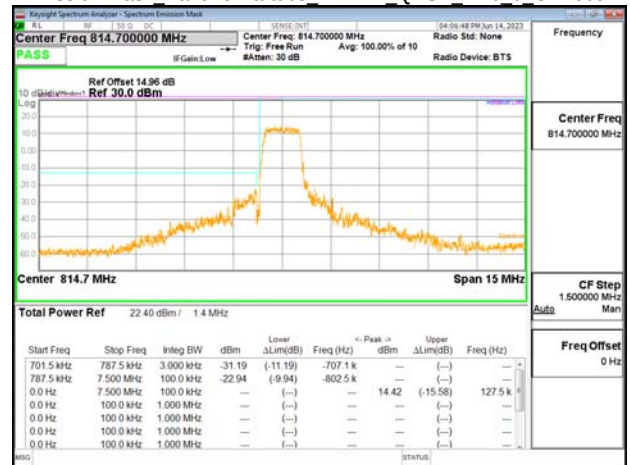
Emission Mask Band26-Part90s 1.4MHz QPSK RB6 0 CH26783
