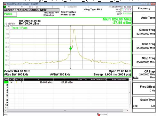
Band Edge Band26 10MHz QPSK RB1 0 CH26840
