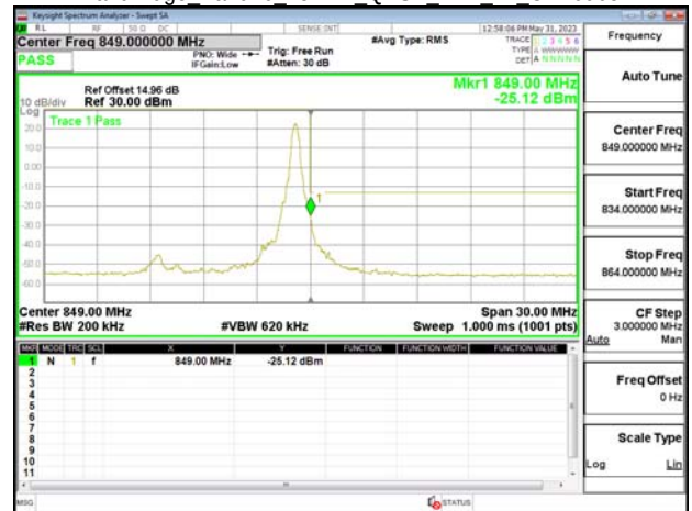
Band Edge Band26 15MHz QPSK RB75 0 CH26865
