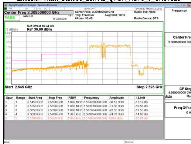
Emission Mask Band38 15MHz QPSK RB75 0 CH37825
