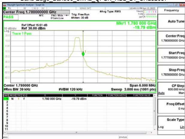
Band Edge Band66 3MHz QPSK RB1 14 CH132657
