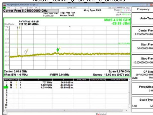
Band17 10MHz QPSK RB1 0 CH23800
