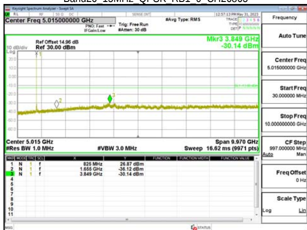
Band26 15MHz QPSK RB1 0 CH26915
