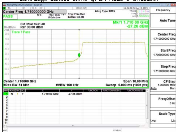
Band Edge Band66 5MHz QPSK RB25 0 CH132647
