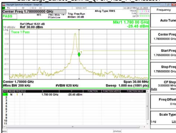
Band Edge Band66 15MHz QPSK RB1 74 CH132597
