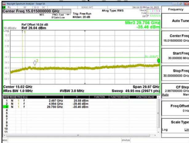
Band41 20MHz QPSK RB1 0 CH40620
