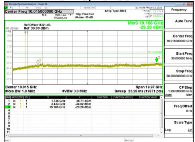
Band66 20MHz QPSK RB1 0 CH132322
