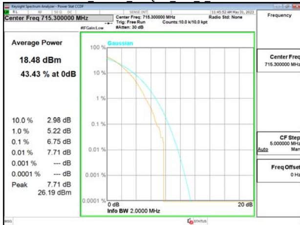
Band12 1.4MHz 256QAM RB6 0 CH23173
