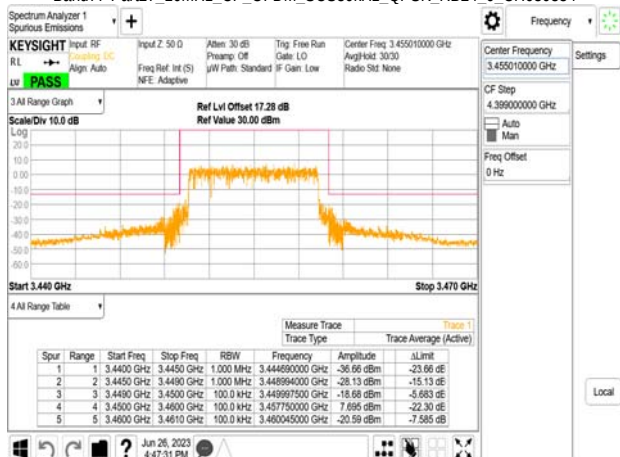
Band77-Part27_10MHz_CP_OFDM_SCS30kHz_QPSK_RB24_0_CH630334
