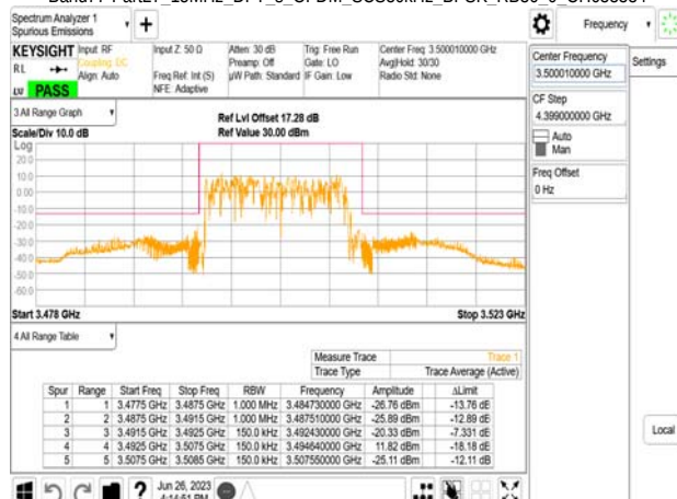
Band77-Part27_15MHz_DFT_s_OFDM_SCS30kHz_BPSK_RB36_0_CH636166
