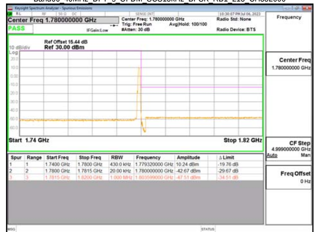
Band66 40MHz DFT s OFDM SCS15kHz BPSK RB1 215 CH352000
