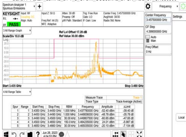
Band77-Part27_15MHz_DFT_s_OFDM_SCS30kHz_BPSK_RB1_37_CH630500
