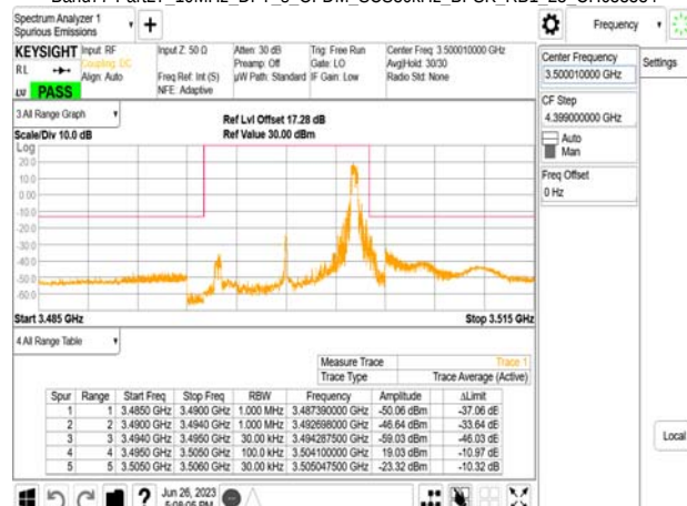
Band77-Part27_10MHz_DFT_s_OFDM_SCS30kHz_BPSK_RB1_23_CH636332
