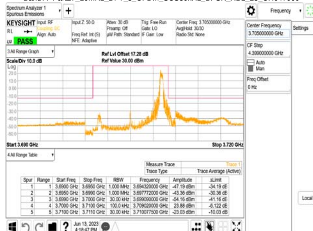
Band77-Part27_10MHz_DFT_s_OFDM_SCS30kHz_BPSK_RB1_23_CH647000
