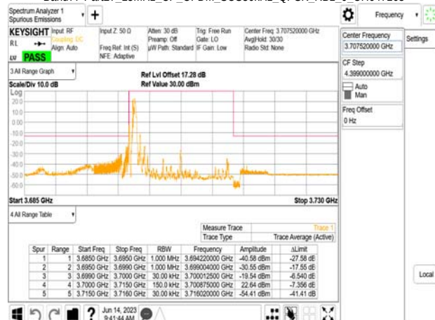
Band77-Part27_15MHz_CP_OFDM_SCS30kHz_QPSK_RB1_0_CH647168
