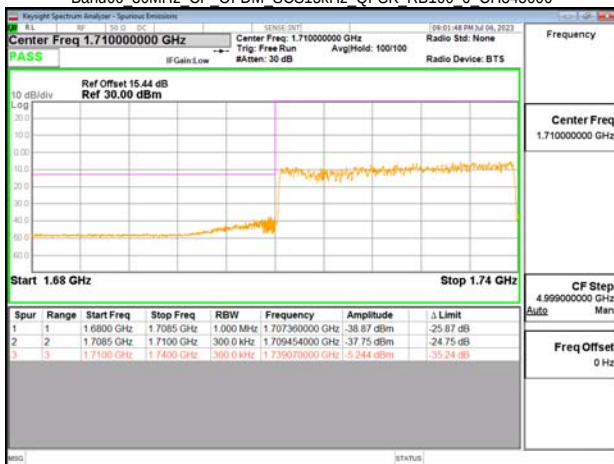
Band66 30MHz CP OFDM SCS15kHz QPSK RB160 0 CH345000
