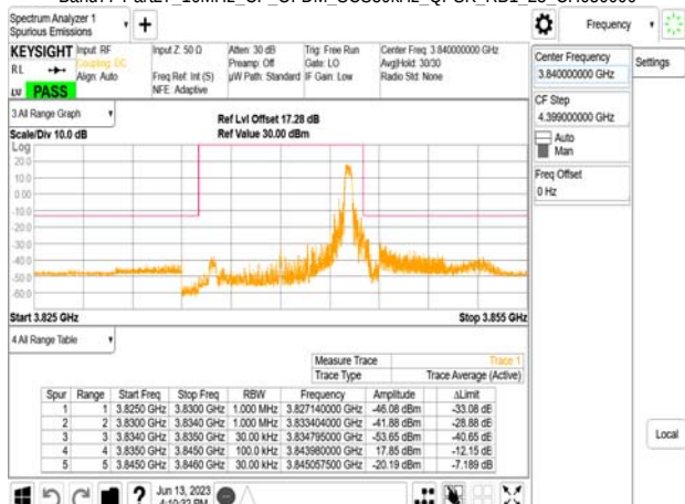
Band77-Part27_10MHz_CP_OFDM_SCS30kHz_QPSK_RB1_23_CH656000
