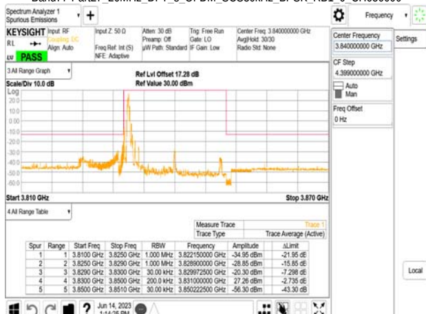
Band77-Part27_20MHz_DFT_s_OFDM_SCS30kHz_BPSK_RB1_0_CH664666
