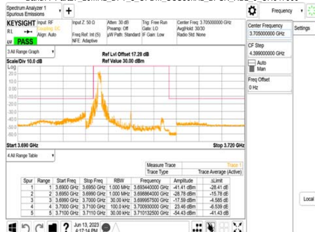
Band77-Part27_10MHz_DFT_s_OFDM_SCS30kHz_BPSK_RB1_0_CH647000
