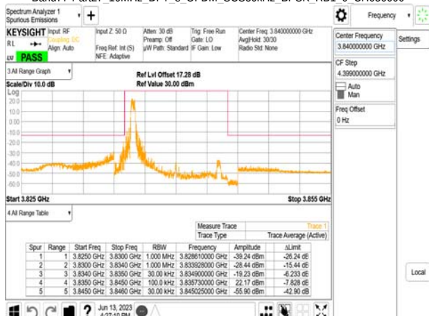
Band77-Part27_10MHz_DFT_s_OFDM_SCS30kHz_BPSK_RB1_0_CH656000
