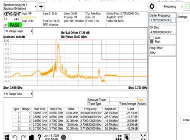
Band77-Part27_15MHz_DFT_s_OFDM_SCS30kHz_BPSK_RB1_0_CH647168
