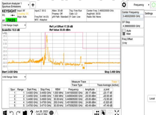
Band77-Part27_20MHz_DFT_s_OFDM_SCS30kHz_BPSK_RB1_0_CH630668
