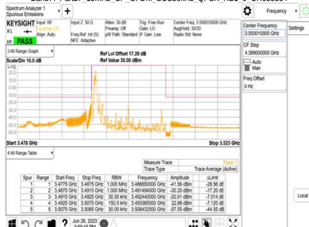
Band77-Part27_15MHz_CP_OFDM_SCS30kHz_QPSK_RB1_0_CH636166
