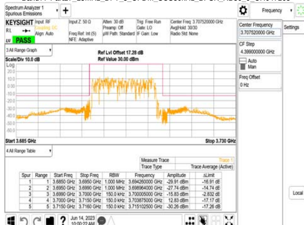
Band77-Part27_15MHz_DFT_s_OFDM_SCS30kHz_BPSK_RB36_0_CH647168
