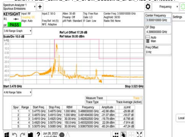
Band77-Part27_15MHz_DFT_s_OFDM_SCS30kHz_BPSK_RB1_0_CH636166
