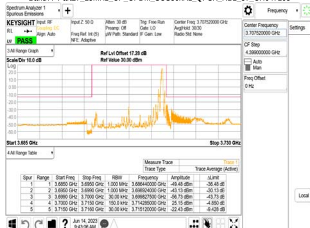
Band77-Part27_15MHz_CP_OFDM_SCS30kHz_QPSK_RB1_37_CH647168
