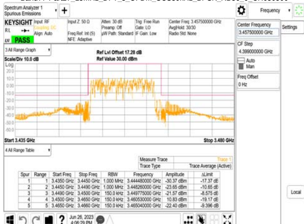
Band77-Part27_15MHz_DFT_s_OFDM_SCS30kHz_BPSK_RB36_0_CH630500
