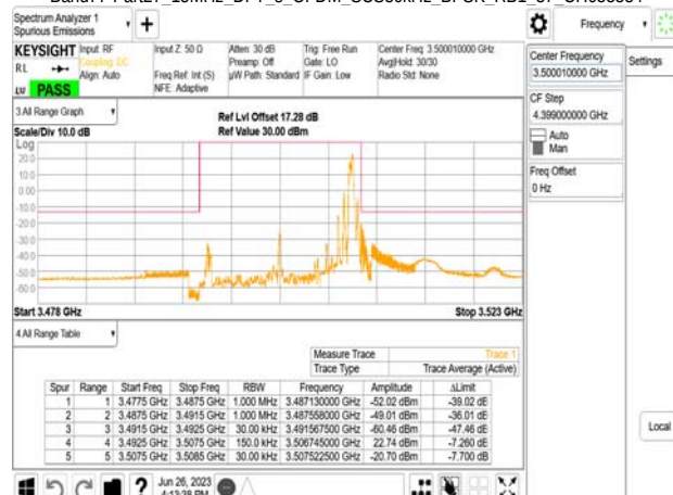
Band77-Part27_15MHz_DFT_s_OFDM_SCS30kHz_BPSK_RB1_37_CH636166
