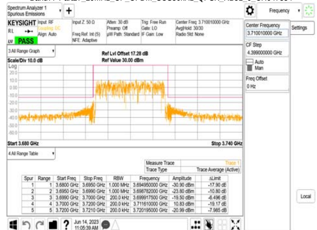
Band77-Part27_20MHz_CP_OFDM_SCS30kHz_QPSK_RB51_0_CH647334
