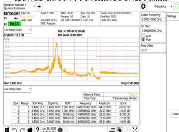
Band77-Part27_10MHz_DFT_s_OFDM_SCS30kHz_BPSK_RB1_0_CH636332
