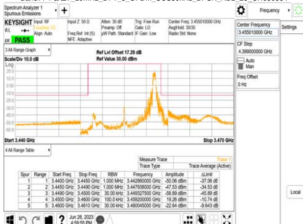
Band77-Part27_10MHz_DFT_s_OFDM_SCS30kHz_BPSK_RB1_23_CH630334
