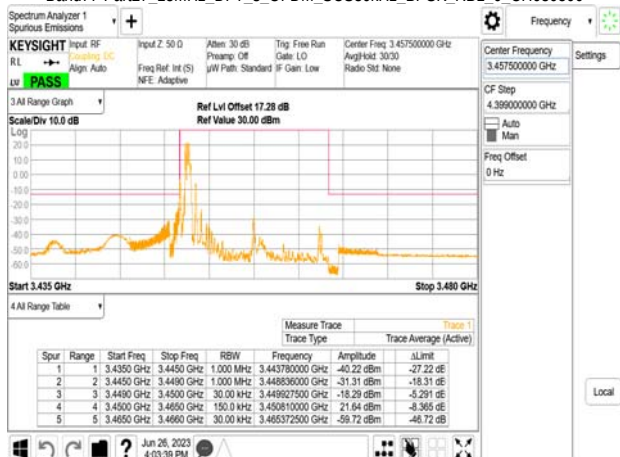
Band77-Part27_15MHz_DFT_s_OFDM_SCS30kHz_BPSK_RB1_0_CH630500
