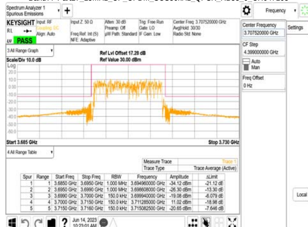
Band77-Part27_15MHz_CP_OFDM_SCS30kHz_QPSK_RB38_0_CH647168
