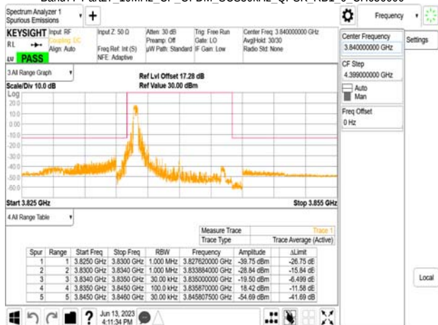
Band77-Part27_10MHz_CP_OFDM_SCS30kHz_QPSK_RB1_0_CH656000
