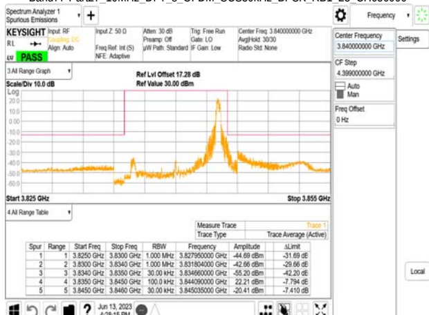
Band77-Part27_10MHz_DFT_s_OFDM_SCS30kHz_BPSK_RB1_23_CH656000
