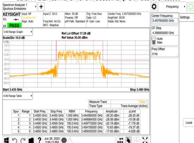
Band77-Part27_15MHz_CP_OFDM_SCS30kHz_QPSK_RB38_0_CH630500
