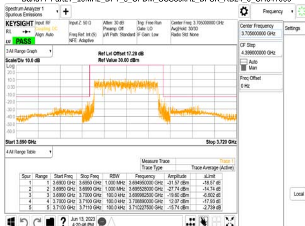
Band77-Part27_10MHz_DFT_s_OFDM_SCS30kHz_BPSK_RB24_0_CH647000
