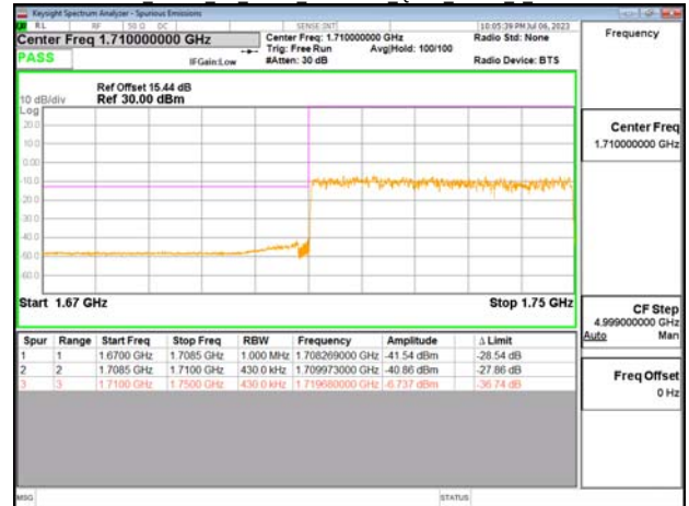
Band66 40MHz CP OFDM SCS15kHz QPSK RB216 0 CH352000
