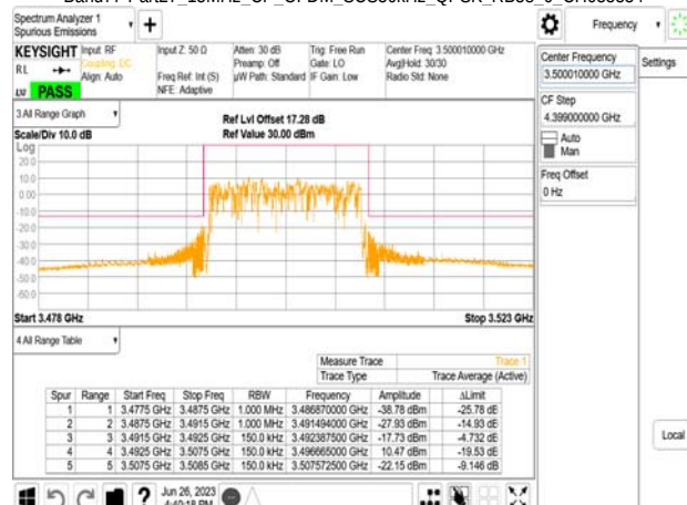
Band77-Part27_15MHz_CP_OFDM_SCS30kHz_QPSK_RB38_0_CH636166
