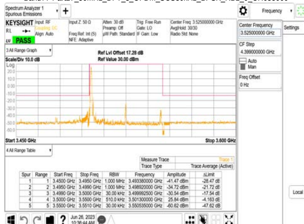
Band77-Part27_50MHz_DFT_s_OFDM_SCS30kHz_BPSK_RB1_0_CH648334
