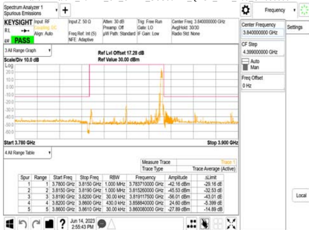
Band77-Part27_40MHz_CP_OFDM_SCS30kHz_QPSK_RB1_105_CH664000
