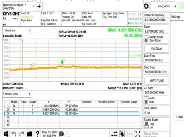
Band5_5MHz_DFT_s_OFDM_SCS15kHz_BPSK_RB1_1_CH169300
