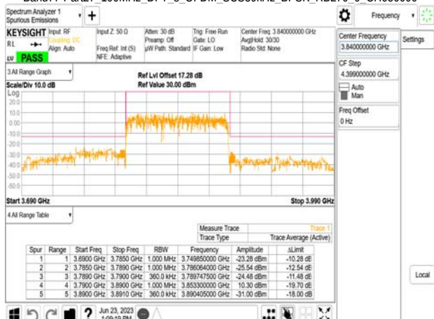
Band77-Part27_100MHz_DFT_s_OFDM_SCS30kHz_BPSK_RB270_0_CH662000
