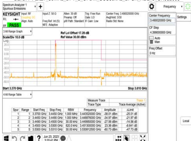
Band77-Part27_80MHz_DFT_s_OFDM_SCS30kHz_BPSK_RB1_0_CH632668
