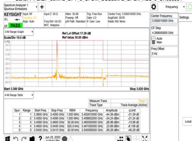
Band77-Part27_80MHz_DFT_s_OFDM_SCS30kHz_BPSK_RB1_0_CH634000
