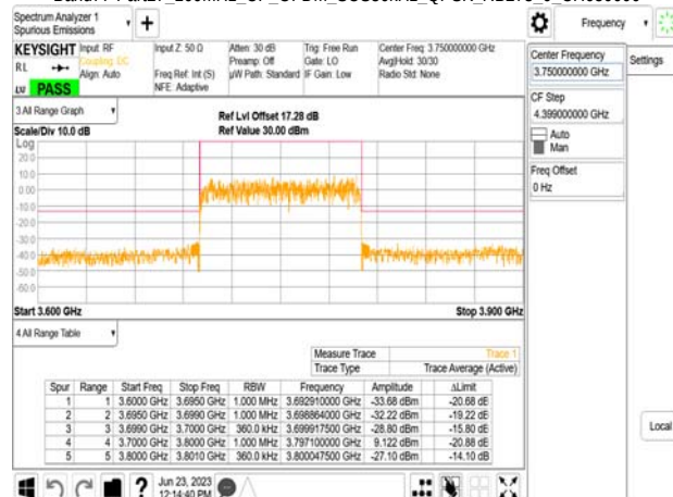
Band77-Part27_100MHz_CP_OFDM_SCS30kHz_QPSK_RB273_0_CH650000
