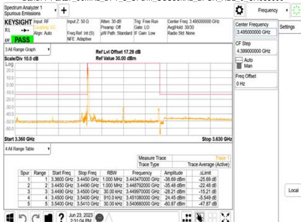
Band77-Part27_90MHz_DFT_s_OFDM_SCS30kHz_BPSK_RB1_0_CH633000
