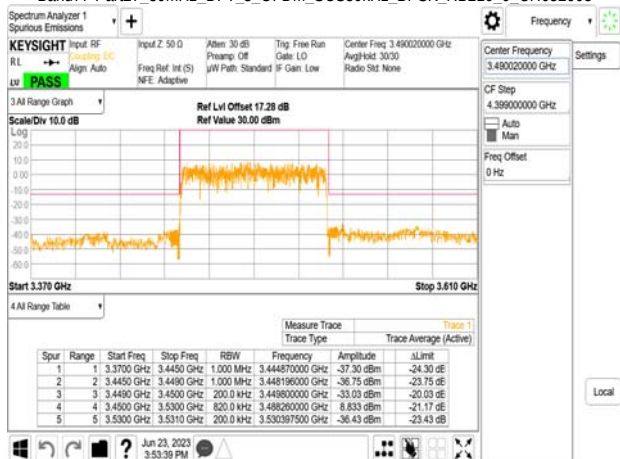
Band77-Part27_80MHz_DFT_s_OFDM_SCS30kHz_BPSK_RB216_0_CH632668
