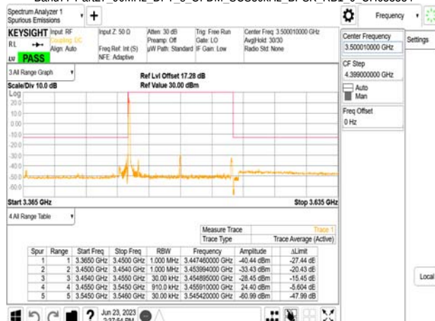
Band77-Part27_90MHz_DFT_s_OFDM_SCS30kHz_BPSK_RB1_0_CH633666
