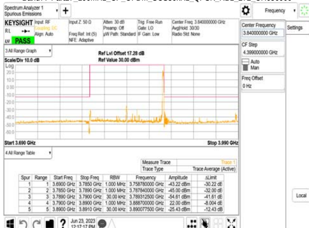
Band77-Part27_100MHz_CP_OFDM_SCS30kHz_QPSK_RB1_272_CH656000
