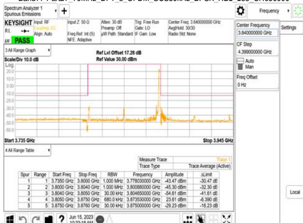
Band77-Part27_70MHz_DFT_s_OFDM_SCS30kHz_BPSK_RB1_188_CH663000
