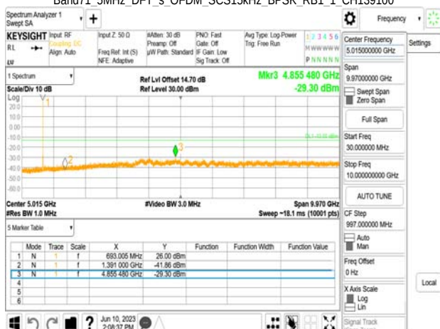
Band71 5MHz_DFT_s_OFDM_SCS15kHz_BPSK_RB1_1_CH139100
