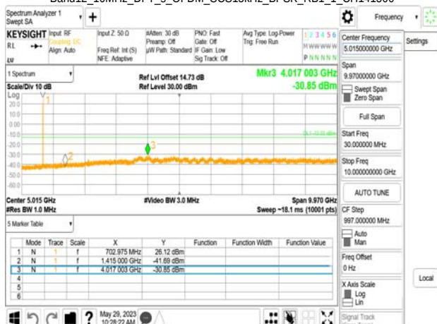
Band12 10MHz_DFT_s_OFDM_SCS15kHz_BPSK_RB1_1_CH142200
