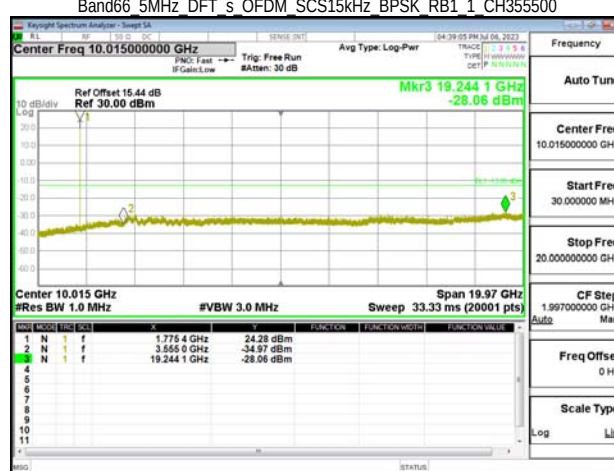
Band66 5MHz DFT s OFDM SCS15kHz BPSK RB1 1 CH355500
