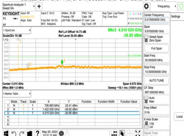
Band12 10MHz_DFT_s_OFDM_SCS15kHz_BPSK_RB1_1_CH142200
