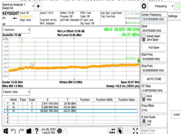
Band41_80MHz_DFT_s_OFDM_SCS30kHz_BPSK_RB1_1_CH529998
