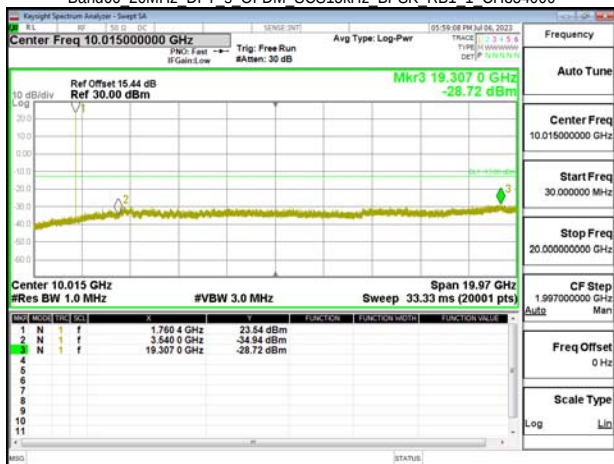
Band66 20MHz DFT s OFDM SCS15kHz BPSK RB1 1 CH354000
