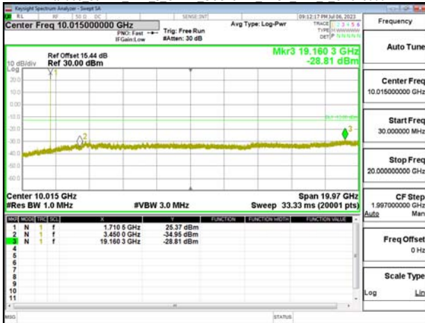
Band66 30MHz DFT s OFDM SCS15kHz BPSK RB1 1 CH349000
