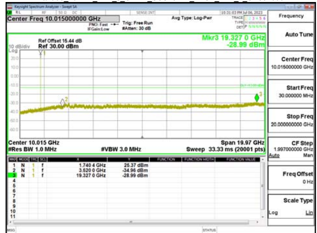
Band66 40MHz DFT s OFDM SCS15kHz BPSK RB1 1 CH352000
