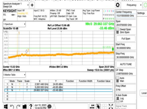
Band38 40MHz_DFT_s_OFDM_SCS30kHz_BPSK_RB1_1_CH520000
