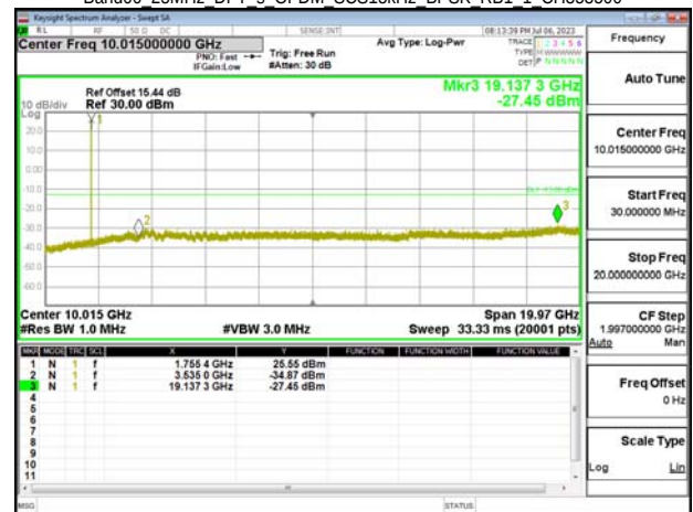
Band66 25MHz DFT s OFDM SCS15kHz BPSK RB1 1 CH353500
