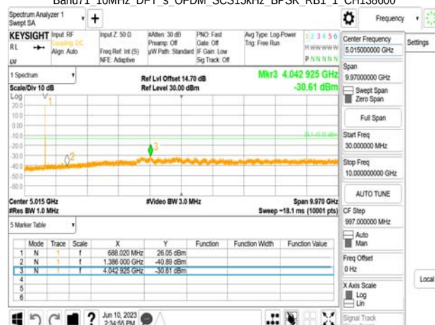
Band71 10MHz_DFT_s_OFDM_SCS15kHz_BPSK_RB1_1_CH138600
