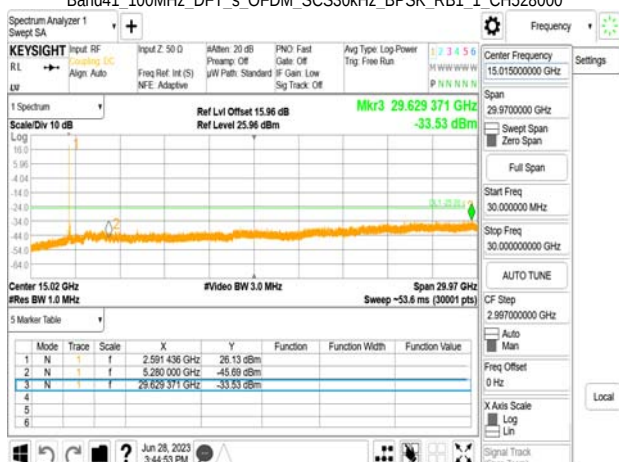
Band41 100MHz DFT s OFDM SCS30kHz BPSK RB1 1 CH528000
