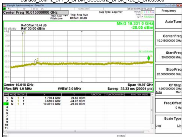
Band66 10MHz DFT s OFDM SCS15kHz BPSK RB1 1 CH355000
