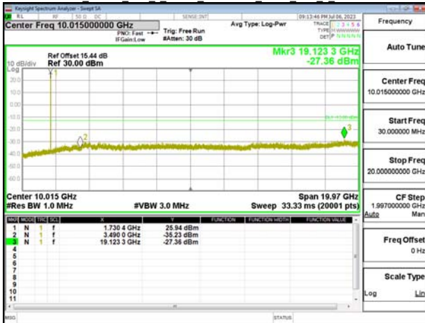
Band66 30MHz DFT s OFDM SCS15kHz BPSK RB1 1 CH353000
