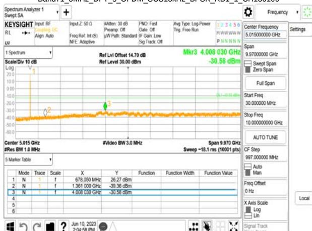
Band71 5MHz_DFT_s_OFDM_SCS15kHz_BPSK_RB1_1_CH139100
