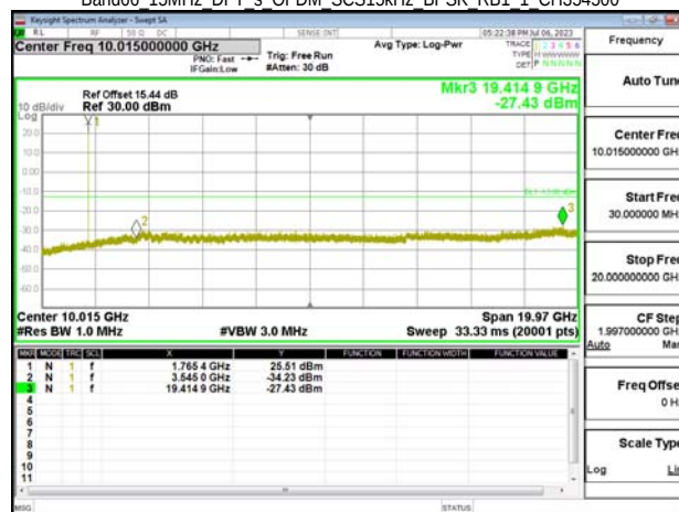
Band66 15MHz DFT s OFDM SCS15kHz BPSK RB1 1 CH354500
