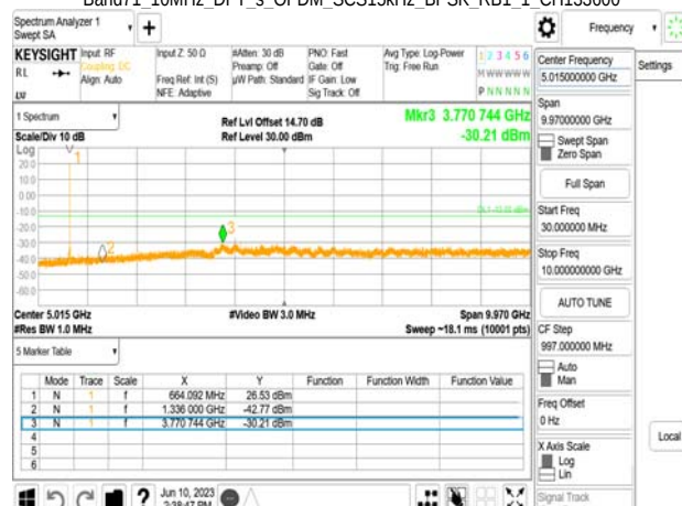
Band71 10MHz_DFT_s_OFDM_SCS15kHz_BPSK_RB1_1_CH136100
