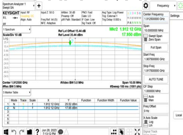
Band25_5MHz_DFT_s_OFDM_SCS15kHz_256QAM_RB25_0_CH382500
