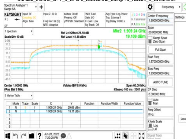
Band25 30MHz_DFT_s_OFDM_SCS15kHz_256QAM_RB160_0_CH380000
