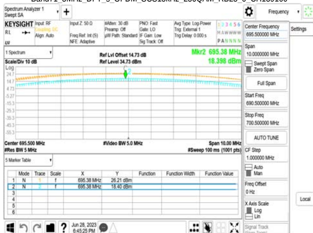
Band71_5MHz_DFT_s_OFDM_SCS15kHz_256QAM_RB25_0_CH139100
