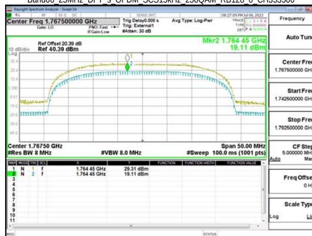
Band66 25MHz DFT s OFDM SCS15kHz 256QAM RB128 0 CH353500
