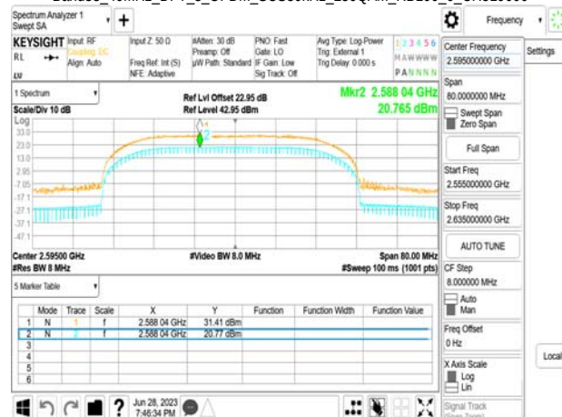
Band38_40MHz_DFT_s_OFDM_SCS30kHz_256QAM_RB100_0_CH520000
