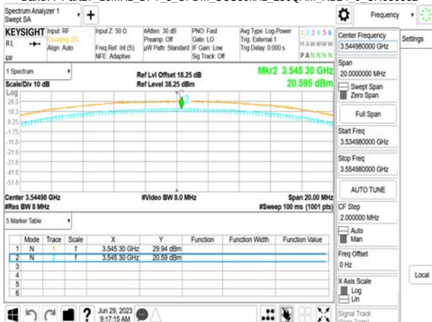
Band77-Part27_10MHz_DFT_s_OFDM_SCS30kHz_256QAM_RB24_0_CH636332
