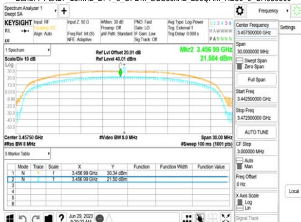
Band77-Part27_15MHz_DFT_s_OFDM_SCS30kHz_256QAM_RB36_0_CH6333334
