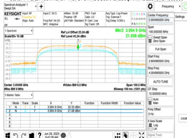
Band77-Part27 50MHz_DFT_s_OFDM_SCS30kHz_256QAM_RB128_0_CH663666
