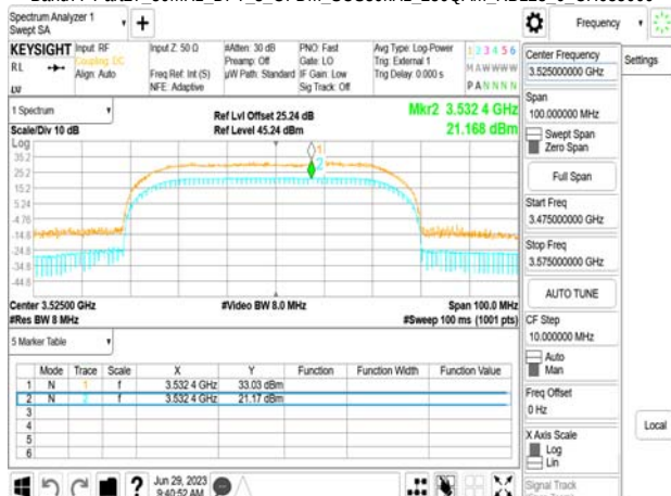
Band77-Part27 50MHz_DFT_s_OFDM_SCS30kHz_256QAM_RB128_0_CH635000
