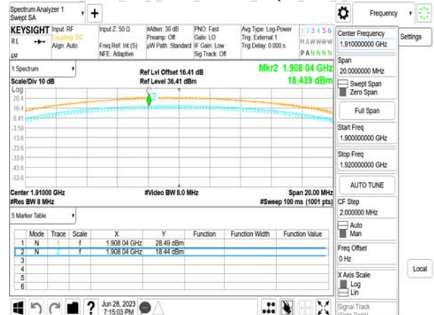
Band25_10MHz_DFT_s_OFDM_SCS15kHz_256QAM_RB50_0_CH382000
