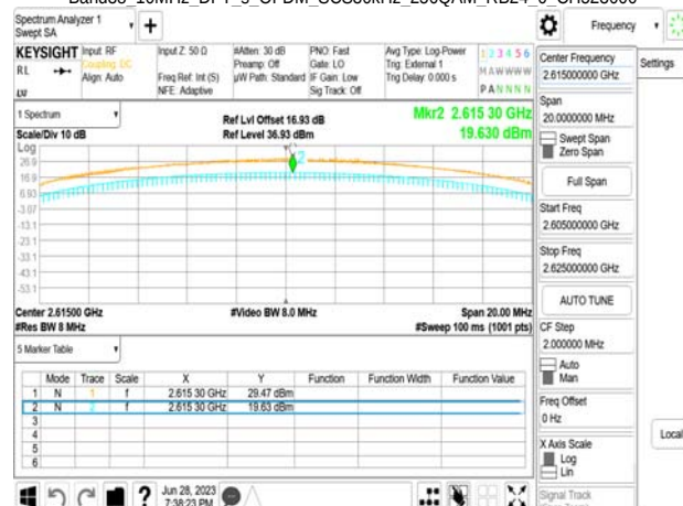
Band38 10MHz_DFT_s_OFDM_SCS30kHz_256QAM_RB24_0_CH523000
