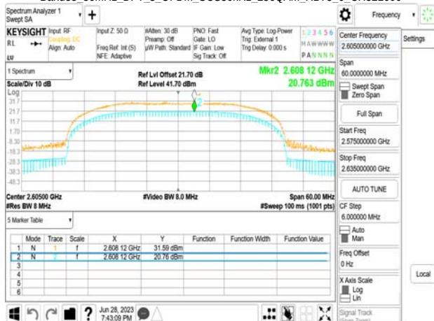
Band38_30MHz_DFT_s_OFDM_SCS30kHz_256QAM_RB75_0_CH521000
