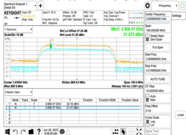
Band77-Part27_80MHz_DFT_s_OFDM_SCS30kHz_256QAM_RB216_0_CH662666
