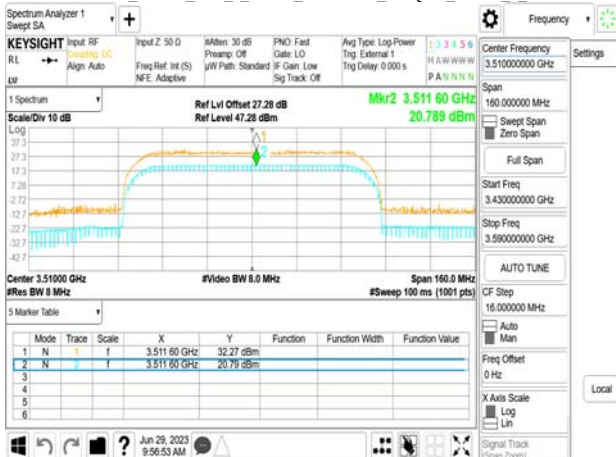
Band77-Part27_80MHz_DFT_s_OFDM_SCS30kHz_256QAM_RB216_0_CH634000
