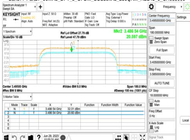
Band77-Part27_90MHz_DFT_s_OFDM_SCS30kHz_256QAM_RB243_0_CH633334
