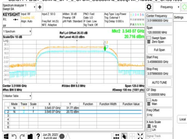
Band77-Part27_60MHz_DFT_s_OFDM_SCS30kHz_256QAM_RB162_0_CH634666
