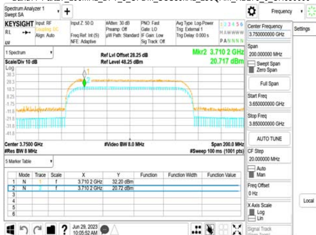
Band77-Part27_100MHz_DFT_s_OFDM_SCS30kHz_256QAM_RB270_0_CH650000
