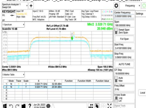
Band77-Part27_90MHz_DFT_s_OFDM_SCS30kHz_256QAM_RB243_0_CH633666
