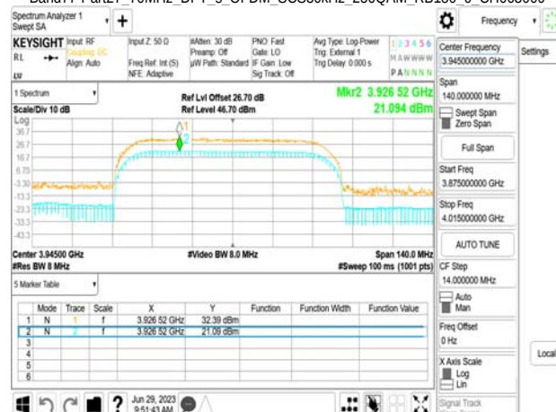
Band77-Part27 70MHz_DFT_s_OFDM_SCS30kHz_256QAM_RB180_0_CH663000
