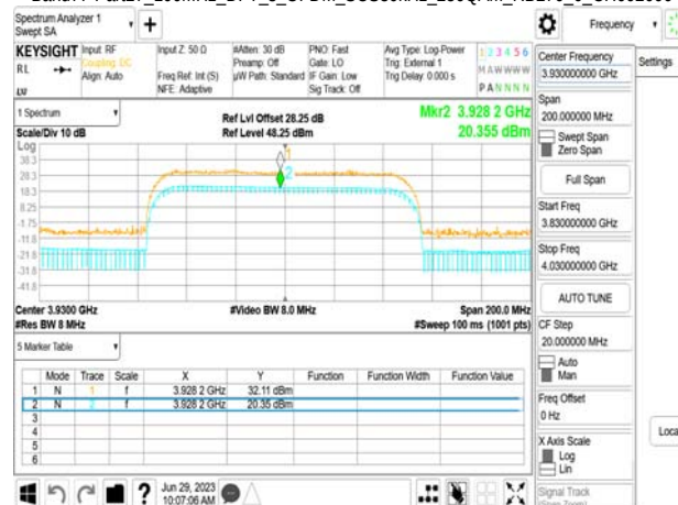
Band77-Part27_100MHz_DFT_s_OFDM_SCS30kHz_256QAM_RB270_0_CH662000
