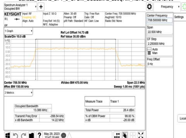
Band12 15MHz DFT_s_OFDM_SCS15kHz_256QAM_RB75_0_CH141700
