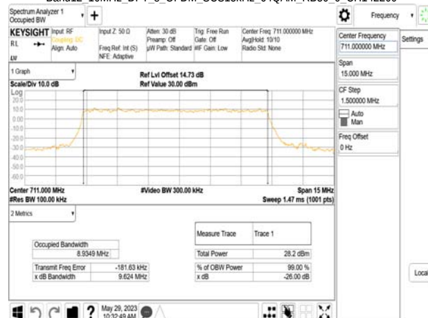
Band12 10MHz DFT_s_OFDM_SCS15kHz_64QAM_RB50_0_CH142200
