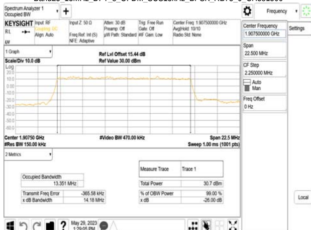
Band25_15MHz_DFT_s_OFDM_SCS15kHz_BPSK_RB75_0_CH381500
