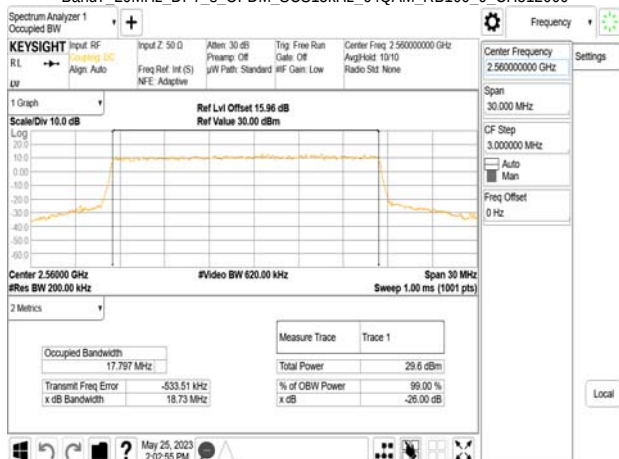
Band7 20MHz_DFT_s_OFDM_SCS15kHz_64QAM_RB100_0_CH512000
