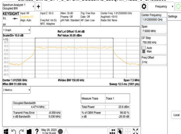
Band25_5MHz_DFT_s_OFDM_SCS15kHz_256QAM_RB25_0_CH382500
