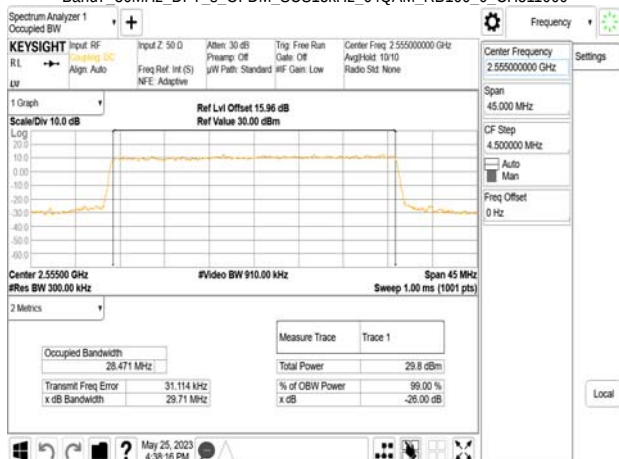
Band7_30MHz_DFT_s_OFDM_SCS15kHz_64QAM_RB160_0_CH511000
