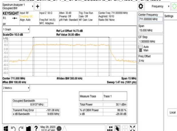
Band12_10MHz_DFT_s_OFDM_SCS15kHz_BPSK_RB50_0_CH142200
