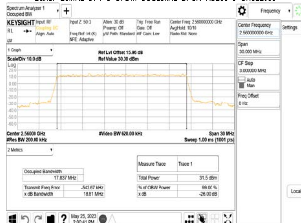
Band7_20MHz_DFT_s_OFDM_SCS15kHz_BPSK_RB100_0_CH512000
