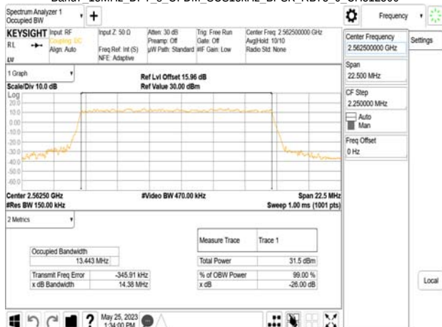
Band7 15MHz DFT_s_OFDM_SCS15kHz_BPSK_RB75_0_CH512500
