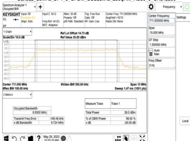
Band12_10MHz_DFT_s_OFDM_SCS15kHz_256QAM_RB50_0_CH142200
