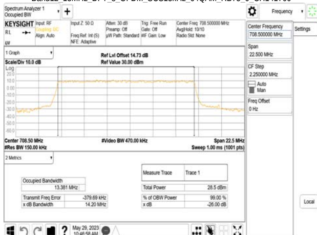
Band12 15MHz DFT_s_OFDM_SCS15kHz_64QAM_RB75_0_CH141700
