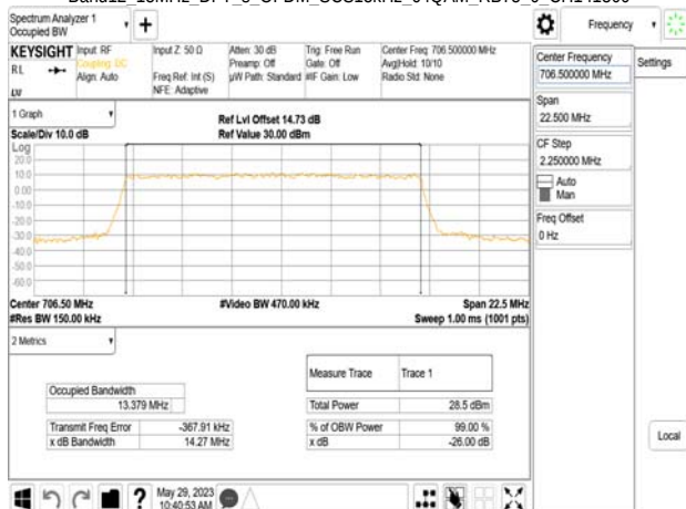
Band12 15MHz DFT_s_OFDM_SCS15kHz_64QAM_RB75_0_CH141500
