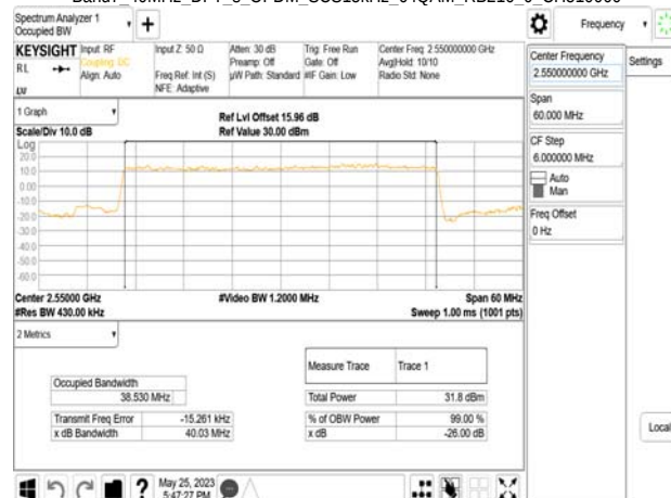
Band7_40MHz_DFT_s_OFDM_SCS15kHz_64QAM_RB216_0_CH510000
