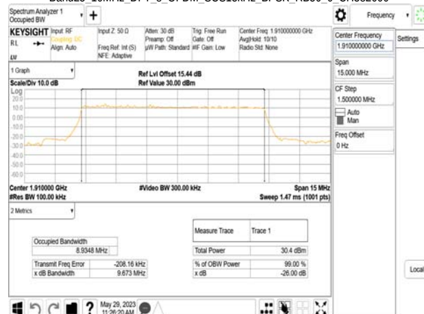
Band25_10MHz_DFT_s_OFDM_SCS15kHz_BPSK_RB50_0_CH382000
