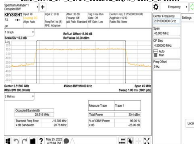
Band7_30MHz_DFT_s_OFDM_SCS15kHz_16QAM_RB160_0_CH507000
