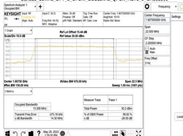
Band25_15MHz_DFT_s_OFDM_SCS15kHz_QPSK_RB75_0_CH381500
