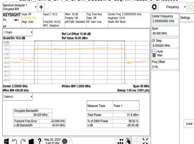
Band7_40MHz_DFT_s_OFDM_SCS15kHz_16QAM_RB216_0_CH510000
