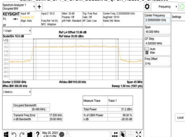
Band7_30MHz_DFT_s_OFDM_SCS15kHz_QPSK_RB160_0_CH511000
