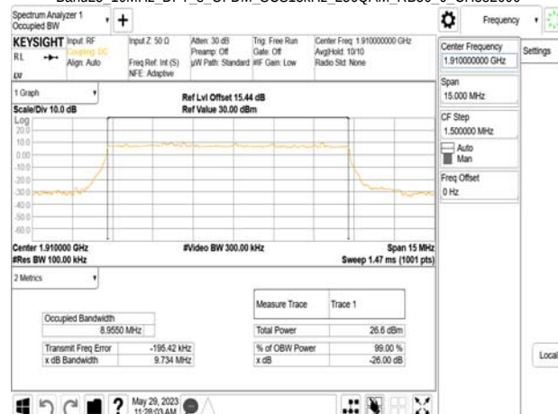
Band25_10MHz_DFT_s_OFDM_SCS15kHz_256QAM_RB50_0_CH382000
