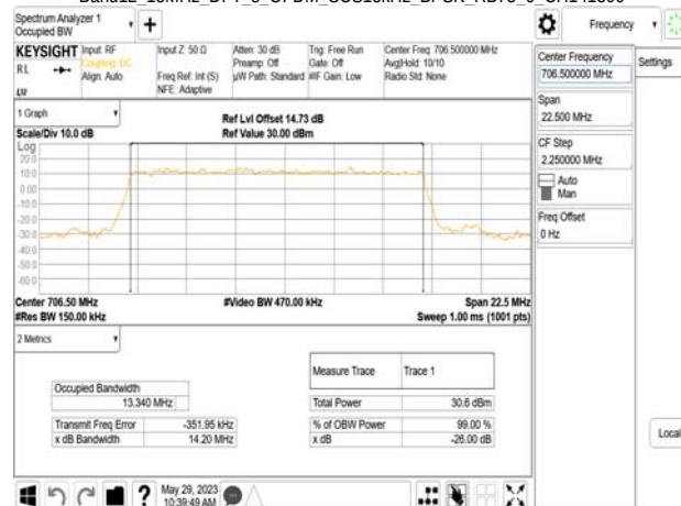
Band12_15MHz_DFT_s_OFDM_SCS15kHz_BPSK_RB75_0_CH141500
