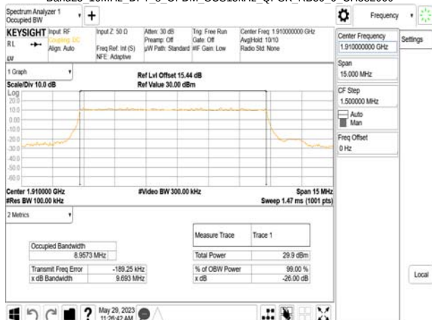
Band25 10MHz DFT s_OFDM_SCS15kHz_QPSK_RB50_0_CH382000
