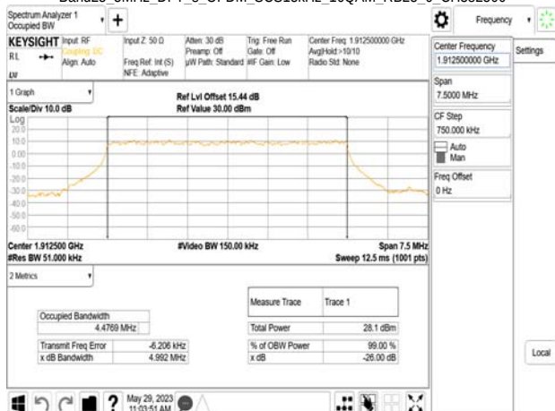
Band25 5MHz_DFT_s_OFDM_SCS15kHz_16QAM_RB25_0_CH382500
