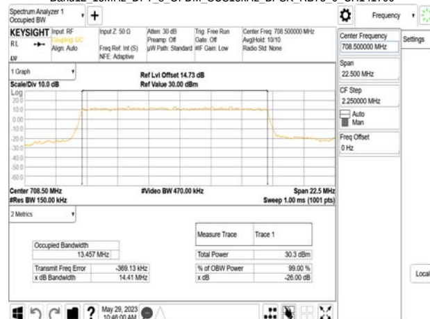
Band12_15MHz_DFT_s_OFDM_SCS15kHz_BPSK_RB75_0_CH141700
