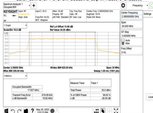
Band7_20MHz_DFT_s_OFDM_SCS15kHz_16QAM_RB100_0_CH512000
