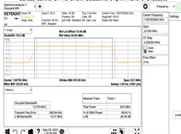
Band25 15MHz DFT_s_OFDM_SCS15kHz 64QAM RB75 0 CH381500
