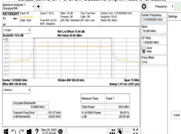
Band25_10MHz_DFT_s_OFDM_SCS15kHz_64QAM_RB50_0_CH382000
