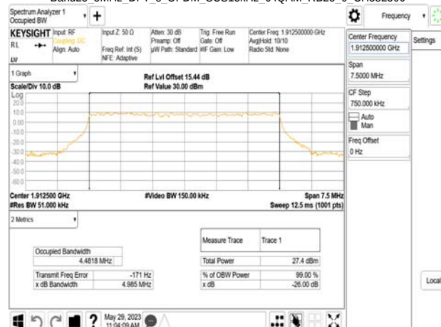
Band25 5MHz_DFT_s_OFDM_SCS15kHz_64QAM_RB25_0_CH382500
