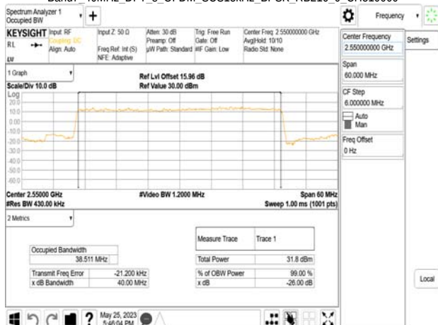
Band7_40MHz_DFT_s_OFDM_SCS15kHz_BPSK_RB216_0_CH510000
