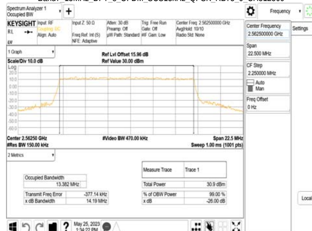
Band7 15MHz DFT_s_OFDM_SCS15kHz_QPSK_RB75_0_CH512500
