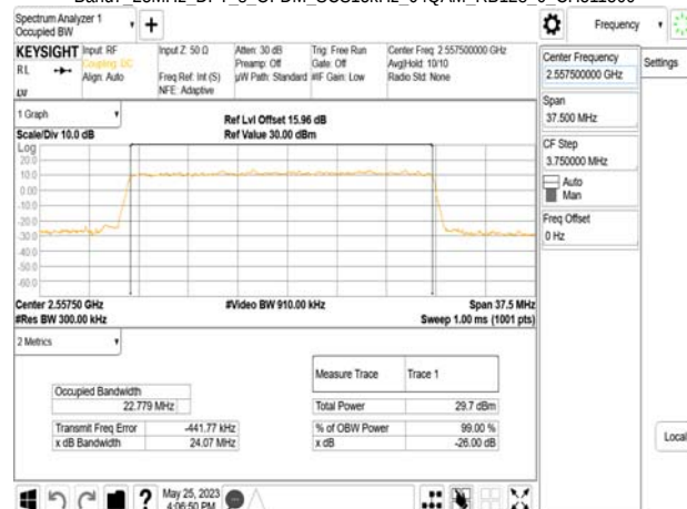
Band7_25MHz_DFT_s_OFDM_SCS15kHz_64QAM_RB128_0_CH511500
