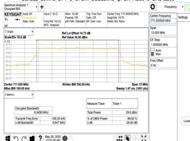
Band12_10MHz_DFT_s_OFDM_SCS15kHz_QPSK_RB50_0_CH142200
