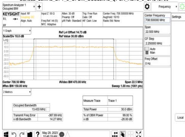
Band12 15MHz_DFT_s_OFDM_SCS15kHz_QPSK_RB75_0_CH141700
