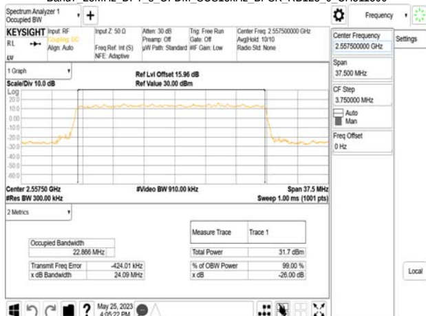
Band7_25MHz_DFT_s_OFDM_SCS15kHz_BPSK_RB128_0_CH511500
