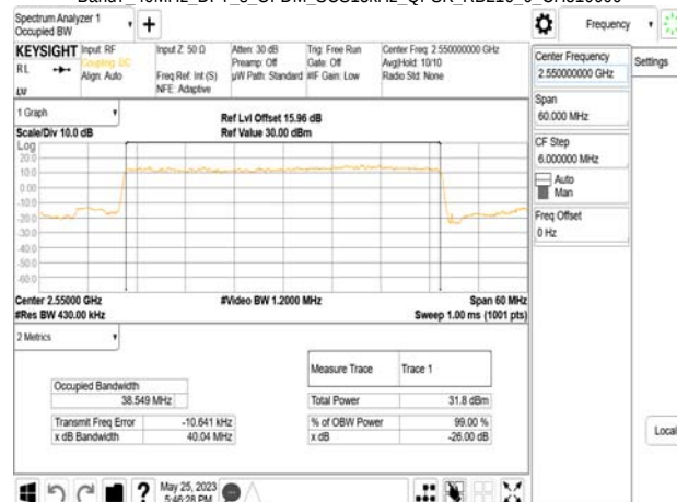
Band7_40MHz_DFT_s_OFDM_SCS15kHz_QPSK_RB216_0_CH510000
