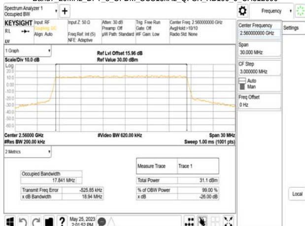
Band7_20MHz_DFT_s_OFDM_SCS15kHz_QPSK_RB100_0_CH512000
