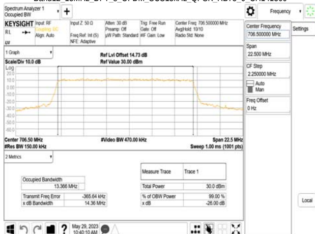
Band12 15MHz_DFT_s_OFDM_SCS15kHz_QPSK_RB75_0_CH141500
