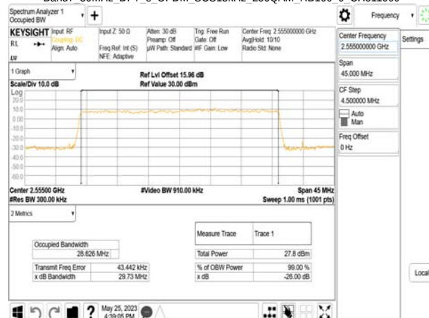
Band7_30MHz_DFT_s_OFDM_SCS15kHz_256QAM_RB160_0_CH511000
