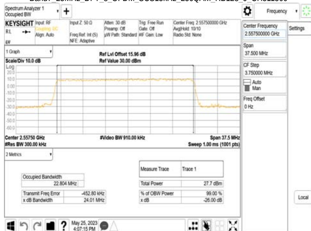
Band7 25MHz_DFT_s_OFDM_SCS15kHz_256QAM_RB128_0_CH511500
