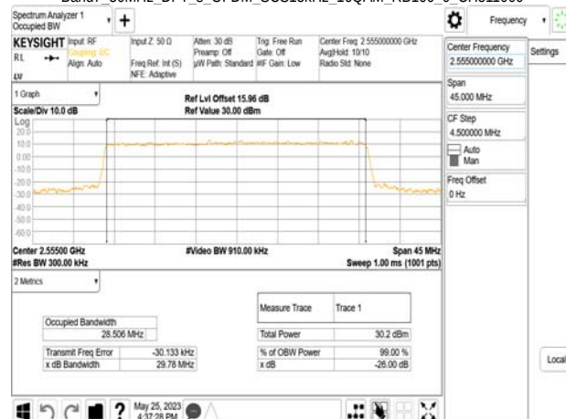
Band7_30MHz_DFT_s_OFDM_SCS15kHz_16QAM_RB160_0_CH511000
