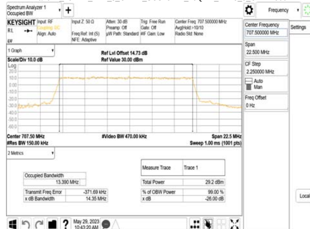
Band12 15MHz_DFT_s_OFDM_SCS15kHz_16QAM_RB75_0_CH141700
