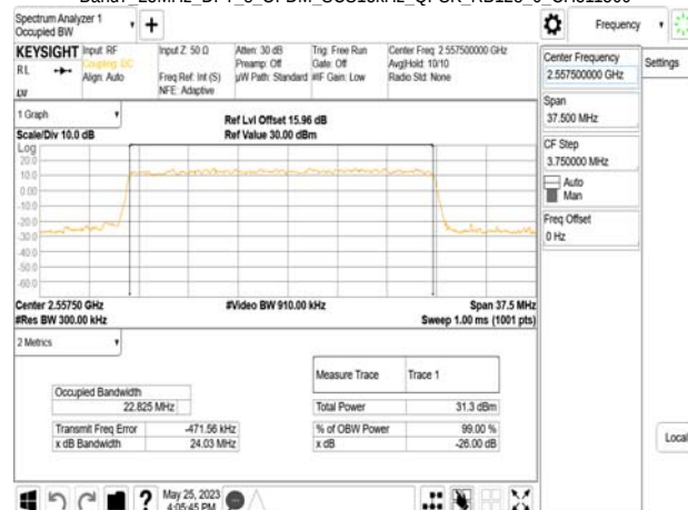
Band7_25MHz_DFT_s_OFDM_SCS15kHz_QPSK_RB128_0_CH511500
