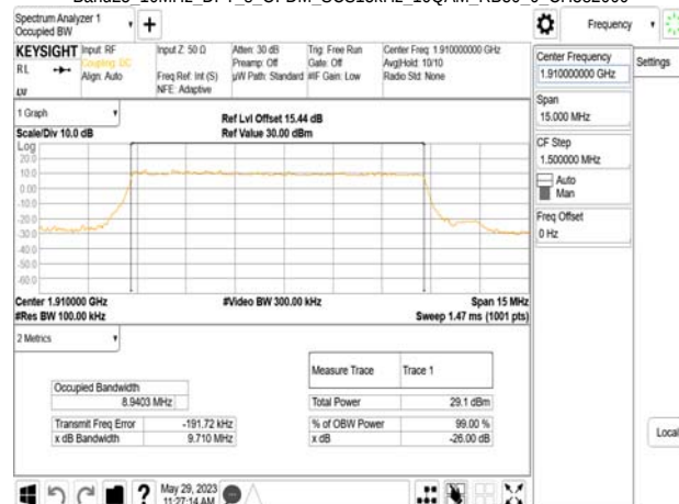
Band25 10MHz DFT s_OFDM_SCS15kHz_16QAM_RB50_0_CH382000
