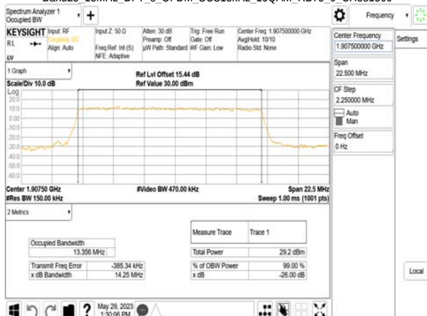
Band25 15MHz DFT_s_OFDM_SCS15kHz 16QAM RB75 0 CH381500
