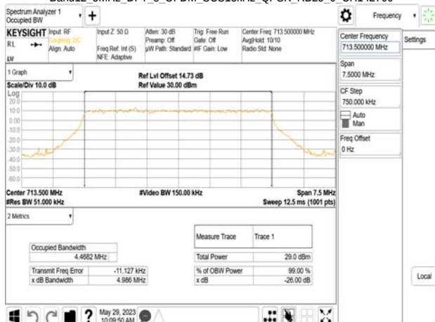
Band12_5MHz_DFT_s_OFDM_SCS15kHz_QPSK_RB25_0_CH142700
