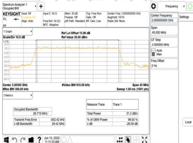
Band38_30MHz_DFT_s_OFDM_SCS30kHz_BPSK_RB75_0_CH521000
