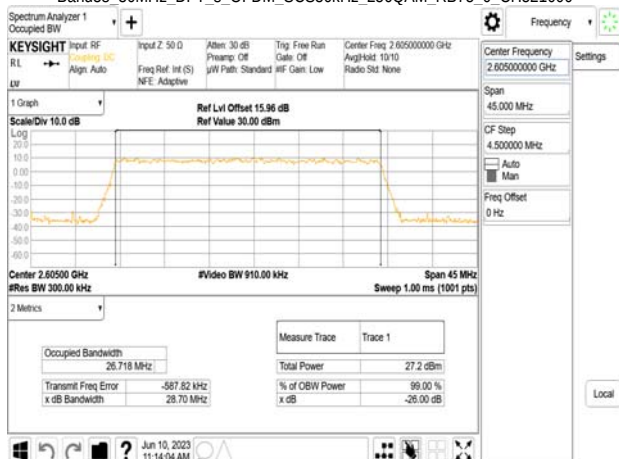
Band38 30MHz DFT_s_OFDM_SCS30kHz_256QAM_RB75_0_CH521000
