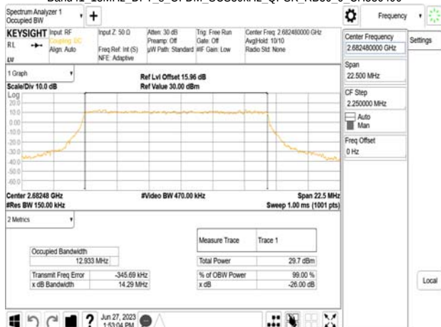
Band41 15MHz DFT s_OFDM_SCS30kHz_QPSK_RB36_0_CH536496
