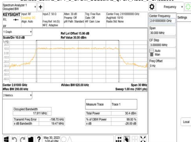
Band38 20MHz DFT_s_OFDM_SCS30kHz_QPSK_RB50_0_CH522000
