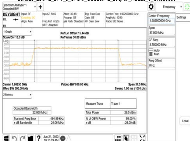
Band25 25MHz DFT_s_OFDM_SCS15kHz_16QAM_RB128_0_CH380500
