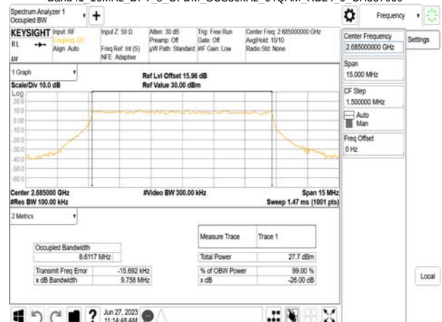
Band41_10MHz_DFT_s_OFDM_SCS30kHz_64QAM_RB24_0_CH537000
