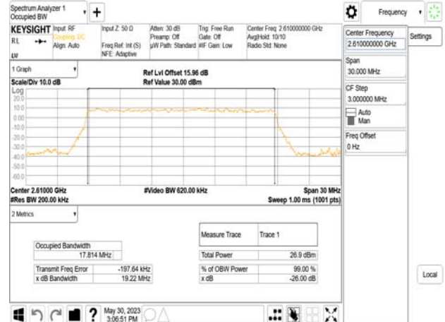
Band38 20MHz DFT_s_OFDM_SCS30kHz 256QAM RB50_0 CH522000
