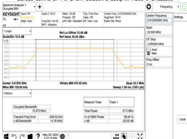
Band38 15MHz_DFT_s_OFDM_SCS30kHz_256QAM_RB36_0_CH522500
