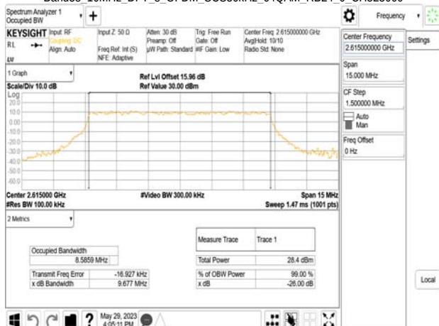
Band38 10MHz DFT_s_OFDM_SCS30kHz 64QAM RB24 0 CH523000
