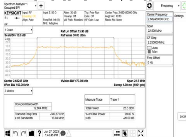
Band41_15MHz_DFT_s_OFDM_SCS30kHz_256QAM_RB36_0_CH536496
