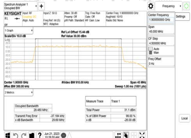
Band25 30MHz_DFT_s_OFDM_SCS15kHz_BPSK_RB160_0_CH380000
