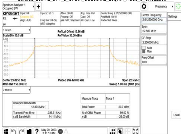
Band38 15MHz DFT_s_OFDM_SCS30kHz 16QAM_RB36_0_CH522500
