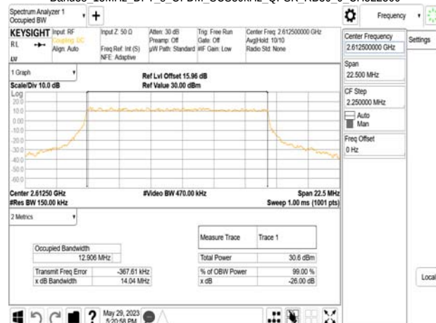
Band38_15MHz_DFT_s_OFDM_SCS30kHz_QPSK_RB36_0_CH522500
