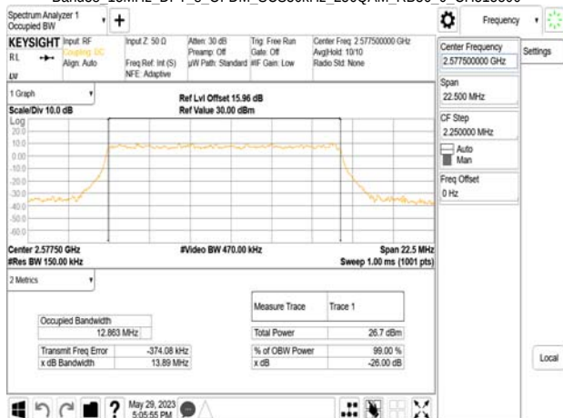
Band38 15MHz_DFT_s_OFDM_SCS30kHz_256QAM_RB36_0_CH519000
