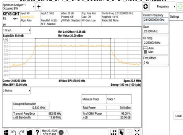
Band38_15MHz_DFT_s_OFDM_SCS30kHz_BPSK_RB36_0_CH522500
