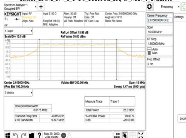
Band38 10MHz DFT_s_OFDM_SCS30kHz_16QAM_RB24_0_CH523000
