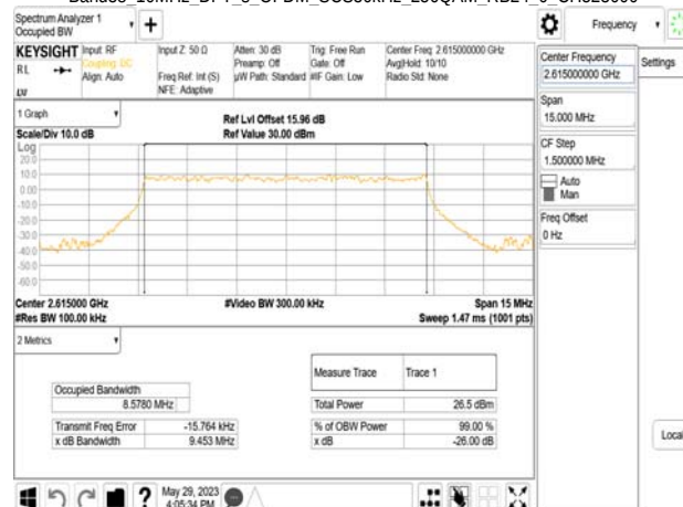
Band38 10MHz DFT_s_OFDM_SCS30kHz 256QAM RB24 0 CH523000
