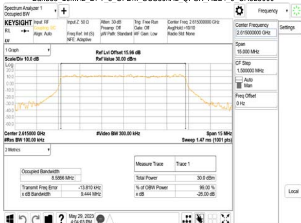
Band38 10MHz DFT_s_OFDM_SCS30kHz_QPSK_RB24_0_CH523000
