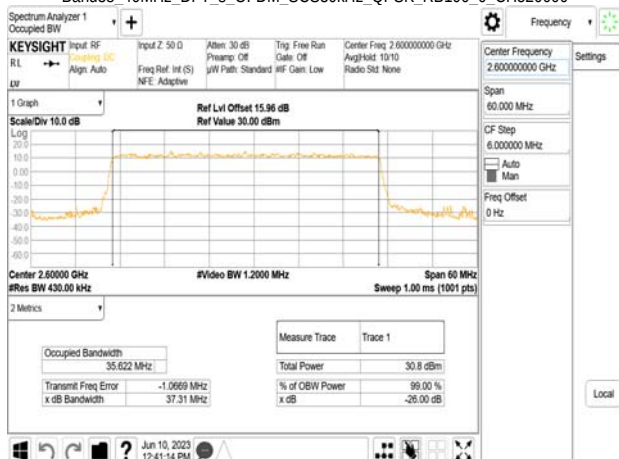
Band38 40MHz DFT_s_OFDM_SCS30kHz QPSK_RB100_0_CH520000
