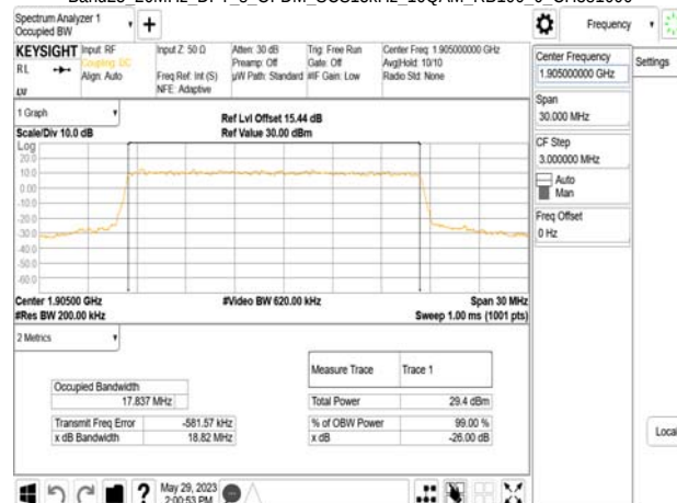
Band25 20MHz DFT_s_OFDM_SCS15kHz 16QAM_RB100_0_CH381000
