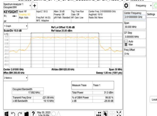
Band38 20MHz_DFT_s_OFDM_SCS30kHz_BPSK_RB50_0_CH522000
