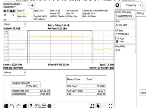
Band25 25MHz DFT_s OFDM_SCS15kHz_QPSK_RB128_0_CH380500
