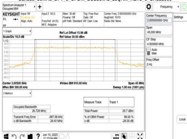
Band38_30MHz_DFT_s_OFDM_SCS30kHz_16QAM_RB75_0_CH521000
