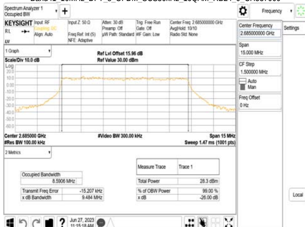
Band41_10MHz_DFT_s_OFDM_SCS30kHz_16QAM_RB24_0_CH537000
