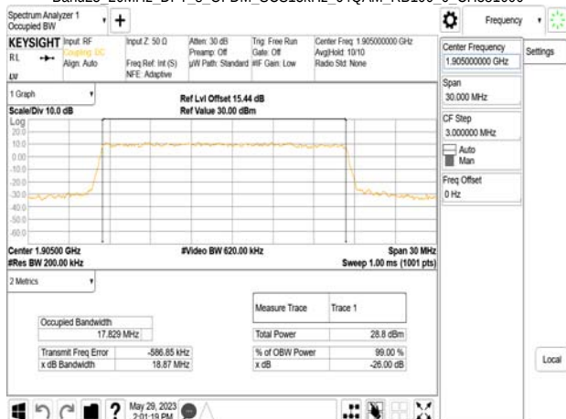
Band25 20MHz DFT s_OFDM_SCS15kHz_64QAM_RB100_0_CH381000
