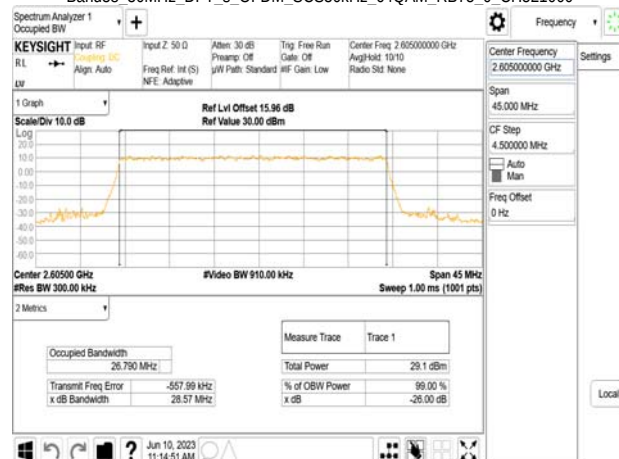
Band38_30MHz_DFT_s_OFDM_SCS30kHz_64QAM_RB75_0_CH521000
