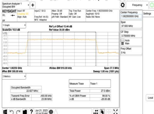
Band25 25MHz_DFT_s_OFDM_SCS15kHz_256QAM_RB128_0_CH380500
