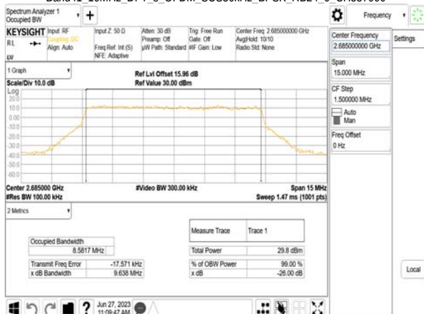
Band41_10MHz_DFT_s_OFDM_SCS30kHz_BPSK_RB24_0_CH537000
