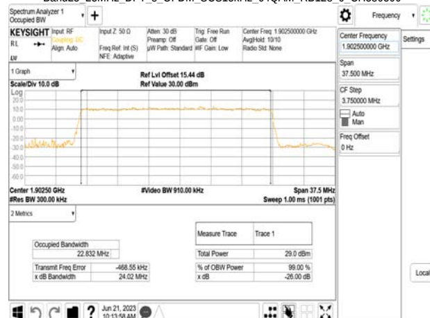
Band25 25MHz DFT_s_OFDM_SCS15kHz_64QAM_RB128_0_CH380500
