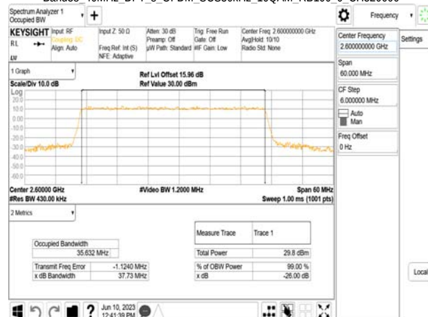
Band38 40MHz DFT_s_OFDM_SCS30kHz_16QAM_RB100_0_CH520000
