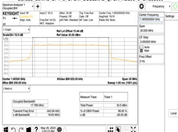
Band25 20MHz DFT_s_OFDM_SCS15kHz QPSK_RB100_0_CH381000
