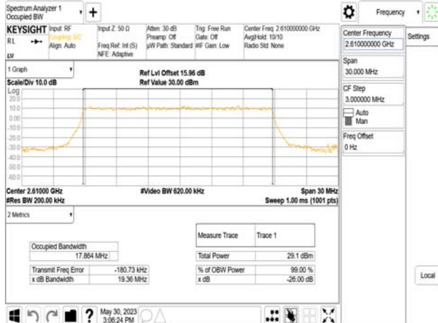
Band38 20MHz DFT_s_OFDM_SCS30kHz 64QAM RB50_0 CH522000
