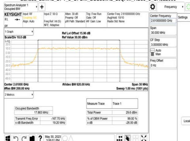
Band38 20MHz DFT_s_OFDM_SCS30kHz_16QAM_RB50_0_CH522000
