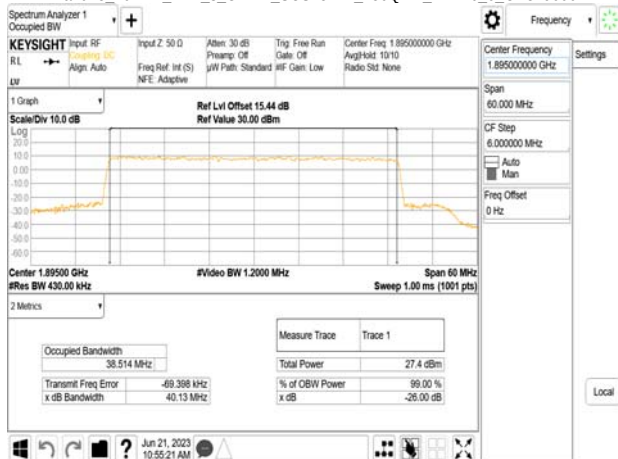
Band25 40MHz_DFT_s_OFDM_SCS15kHz_256QAM_RB216_0_CH379000
