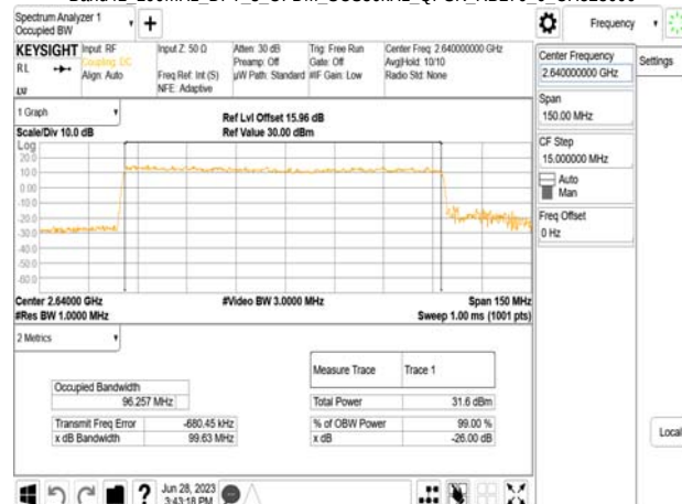
Band41_100MHz_DFT_s_OFDM_SCS30kHz_QPSK_RB270_0_CH528000
