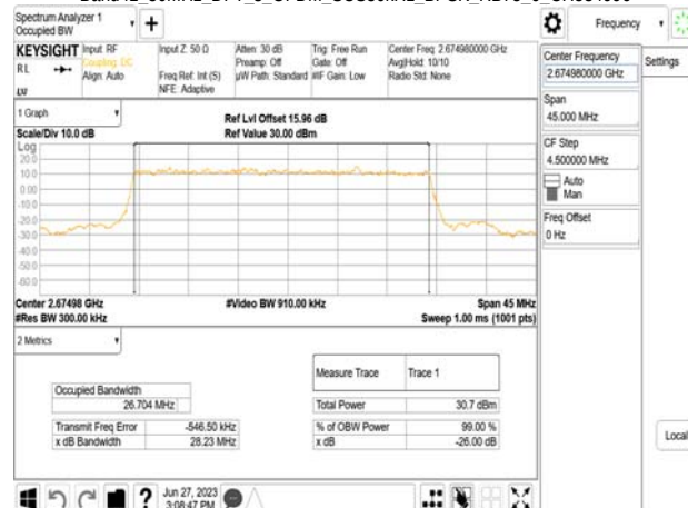
Band41_30MHz_DFT_s_OFDM_SCS30kHz_BPSK_RB75_0_CH534996
