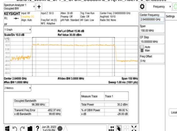
Band41_100MHz_DFT_s_OFDM_SCS30kHz_64QAM_RB270_0_CH528000
