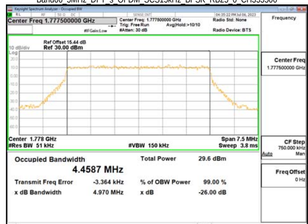
Band66 5MHz DFT s OFDM_SCS15kHz BPSK_RB25_0_CH355500
