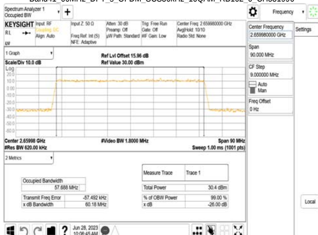
Band41_60MHz_DFT_s_OFDM_SCS30kHz_16QAM_RB162_0_CH531996
