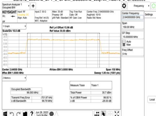
Band41_100MHz_DFT_s_OFDM_SCS30kHz_16QAM_RB270_0_CH528000
