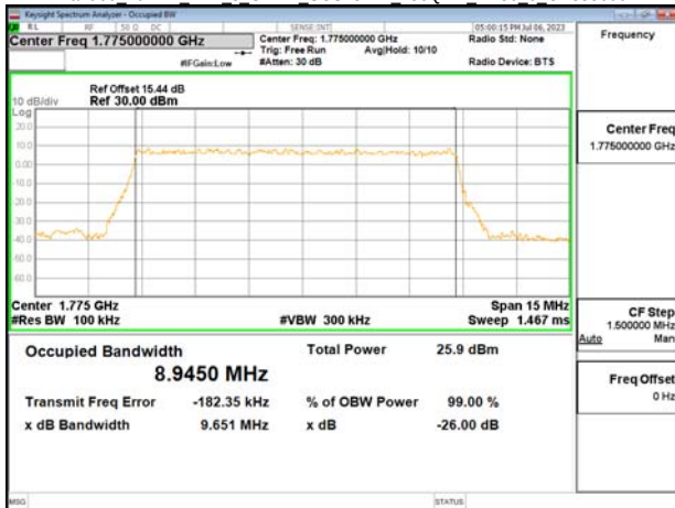
Band66 10MHz DFT s OFDM SCS15kHz 256QAM RB50 0 CH355000
