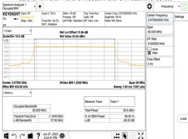
Band41 40MHz DFT_s_OFDM_SCS30kHz_BPSK_RB100_0_CH534000
