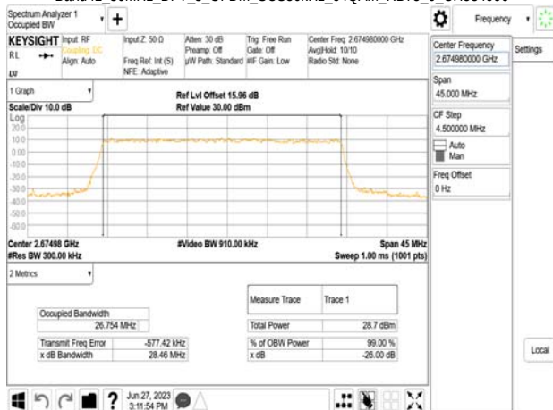
Band41_30MHz_DFT_s_OFDM_SCS30kHz_64QAM_RB75_0_CH534996
