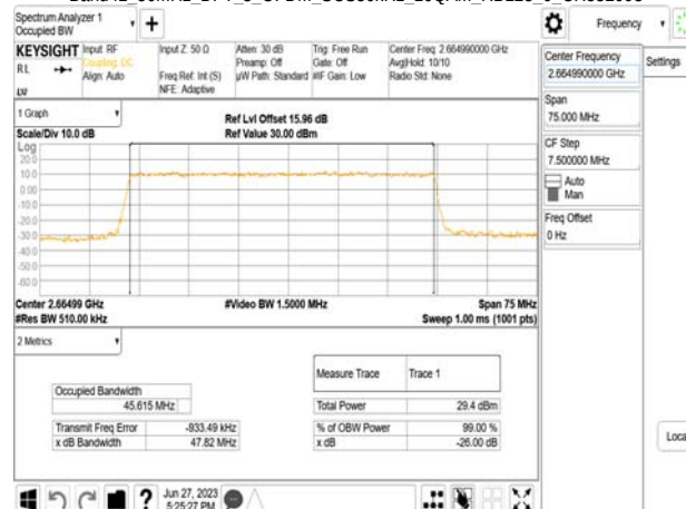
Band41_50MHz_DFT_s_OFDM_SCS30kHz_16QAM_RB128_0_CH532998
