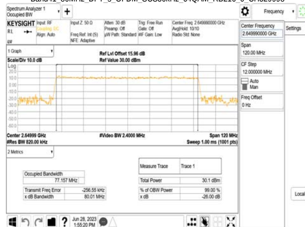
Band41_80MHz_DFT_s_OFDM_SCS30kHz_64QAM_RB216_0_CH529998
