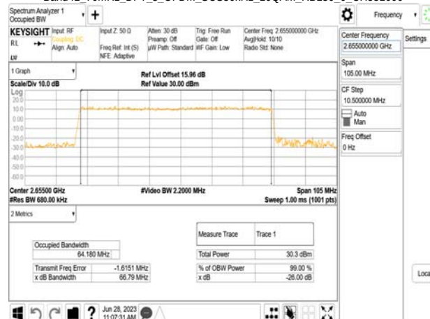
Band41_70MHz_DFT_s_OFDM_SCS30kHz_16QAM_RB180_0_CH531000
