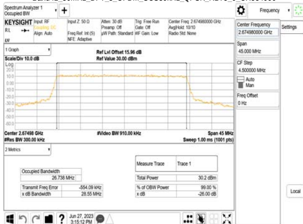
Band41_30MHz_DFT_s_OFDM_SCS30kHz_QPSK_RB75_0_CH534996
