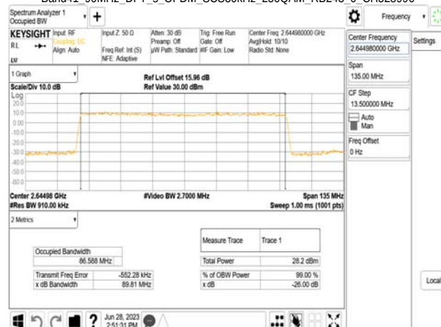
Band41_90MHz_DFT_s_OFDM_SCS30kHz_256QAM_RB243_0_CH528996
