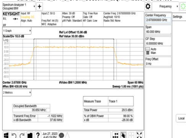
Band41_40MHz_DFT_s_OFDM_SCS30kHz_16QAM_RB100_0_CH534000
