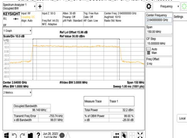
Band41_100MHz_DFT_s_OFDM_SCS30kHz_BPSK_RB270_0_CH528000
