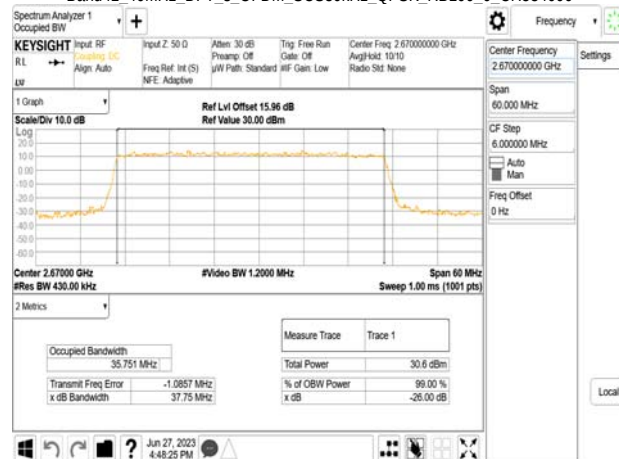
Band41 40MHz DFT_s_OFDM_SCS30kHz_QPSK_RB100_0_CH534000
