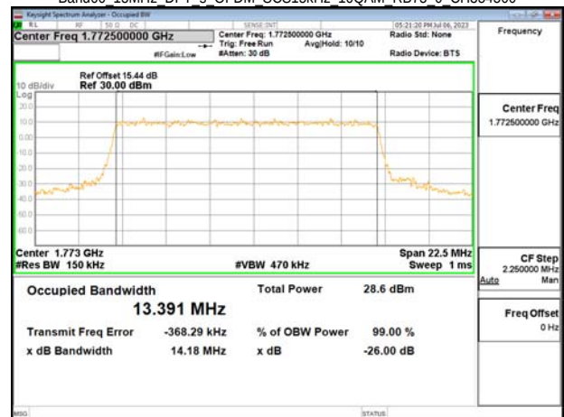
Band66 15MHz DFT s OFDM SCS15kHz 16QAM RB75 0 CH354500
