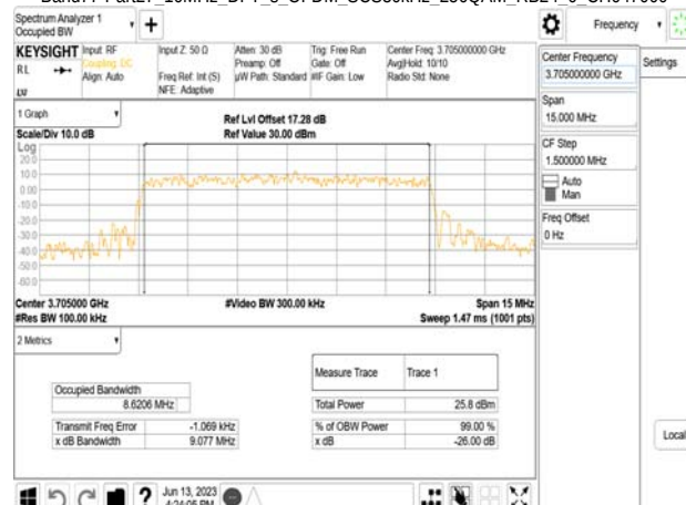
Band77-Part27_10MHz_DFT_s_OFDM_SCS30kHz_256QAM_RB24_0_CH656000
