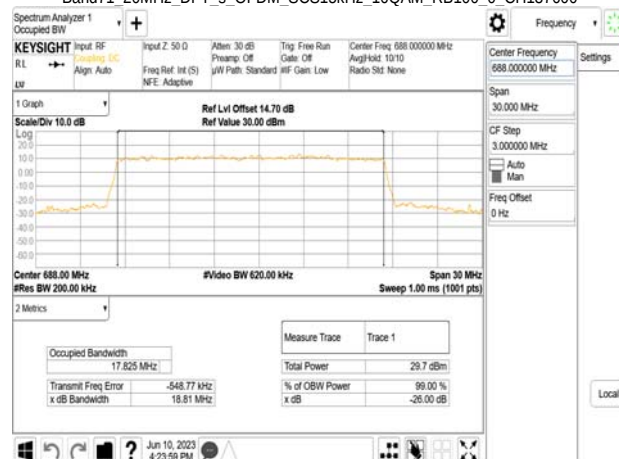
Band71 20MHz_DFT_s_OFDM_SCS15kHz_16QAM_RB100_0_CH137600
