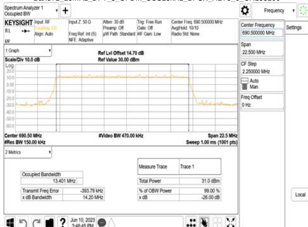
Band71_15MHz_DFT_s_OFDM_SCS15kHz_BPSK_RB75_0_CH138100
