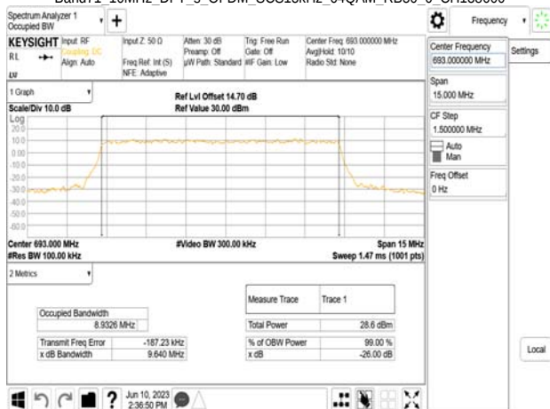
Band71_10MHz_DFT_s_OFDM_SCS15kHz_64QAM_RB50_0_CH138600
