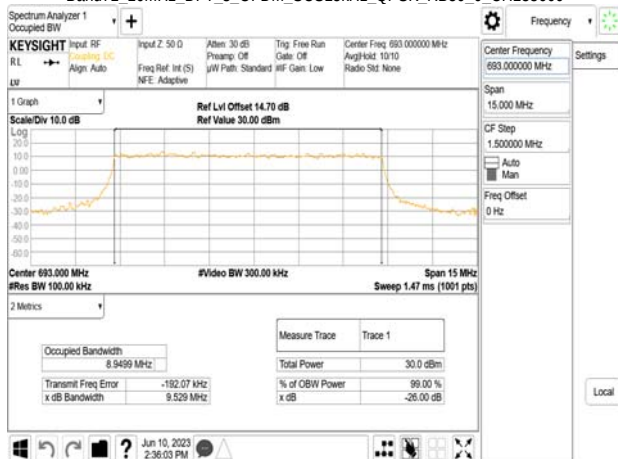
Band71_10MHz_DFT_s_OFDM_SCS15kHz_QPSK_RB50_0_CH138600
