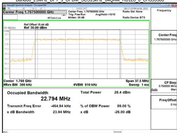
Band66 25MHz DFT s OFDM SCS15kHz 64QAM RB128 0 CH353500
