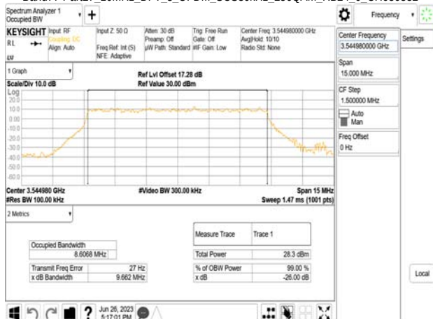
Band77-Part27_10MHz_DFT_s_OFDM_SCS30kHz_256QAM_RB24_0_CH636332
