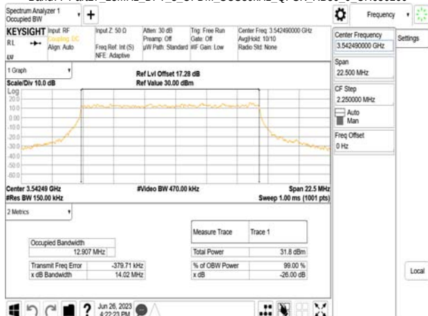
Band77-Part27_15MHz_DFT_s_OFDM_SCS30kHz_QPSK_RB36_0_CH636166
