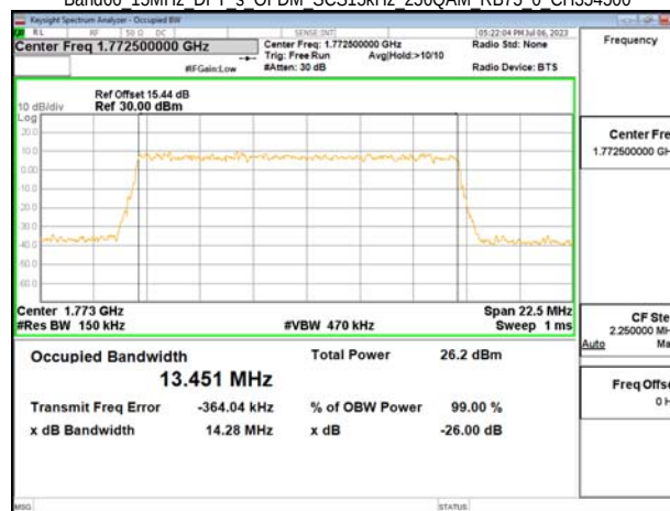
Band66 15MHz DFT s OFDM SCS15kHz 256QAM RB75 0 CH354500
