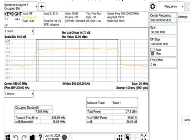
Band71_20MHz_DFT_s_OFDM_SCS15kHz_256QAM_RB100_0_CH137600
