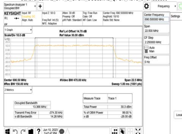
Band71_15MHz_DFT_s_OFDM_SCS15kHz_QPSK_RB75_0_CH138100
