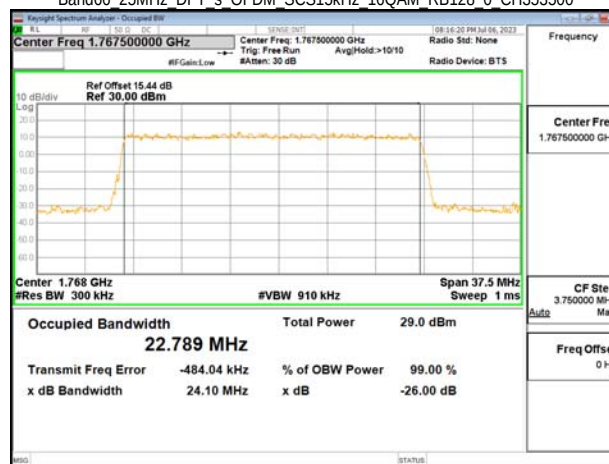
Band66 25MHz DFT s OFDM SCS15kHz 16OAM RB128 0 CH353500
