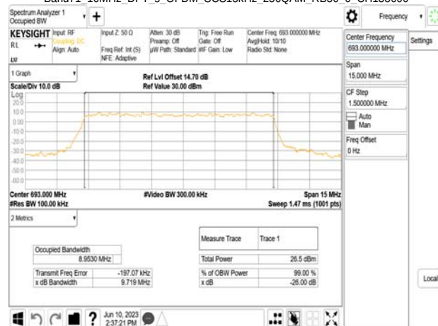
Band71_10MHz_DFT_s_OFDM_SCS15kHz_256QAM_RB50_0_CH138600
