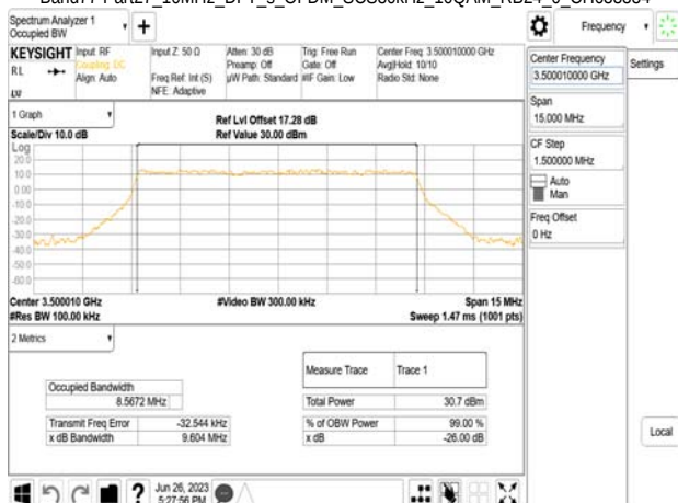
Band77-Part27_10MHz_DFT_s_OFDM_SCS30kHz_16QAM_RB24_0_CH636332
