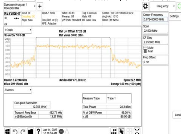
Band77-Part27_15MHz_DFT_s_OFDM_SCS30kHz_QPSK_RB36_0_CH664832
