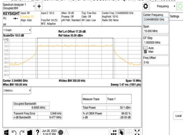
Band77-Part27_10MHz_DFT_s_OFDM_SCS30kHz_64QAM_RB24_0_CH636332
