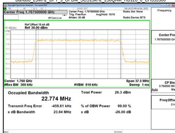
Band66 25MHz DFT s OFDM SCS15kHz 256QAM RB128 0 CH353500
