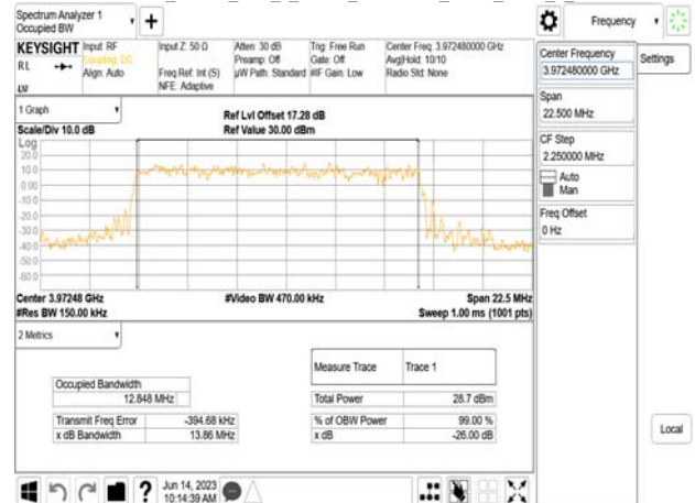
Band77-Part27_15MHz_DFT_s_OFDM_SCS30kHz_BPSK_RB36_0_CH664832
