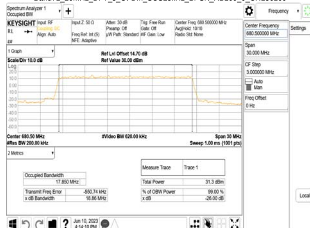
Band71 20MHz_DFT_s_OFDM_SCS15kHz_BPSK_RB100_0_CH137600
