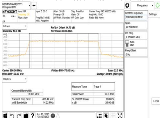
Band71 15MHz_DFT_s_OFDM_SCS15kHz_256QAM_RB75_0_CH138100
