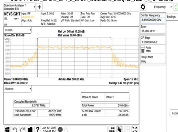
Band77-Part27_10MHz_DFT_s_OFDM_SCS30kHz_256QAM_RB24_0_CH656000
