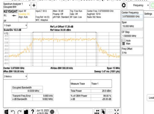
Band77-Part27_10MHz_DFT_s_OFDM_SCS30kHz_QPSK_RB24_0_CH665000
