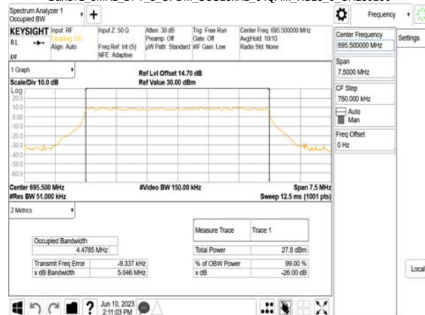
Band71_5MHz_DFT_s_OFDM_SCS15kHz_64QAM_RB25_0_CH139100
