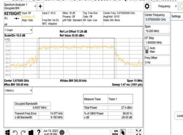
Band77-Part27_10MHz_DFT_s_OFDM_SCS30kHz_64QAM_RB24_0_CH665000
