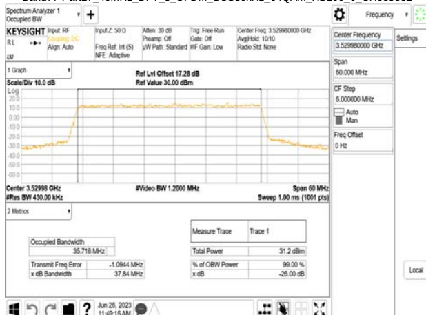
Band77-Part27 40MHz_DFT_s_OFDM_SCS30kHz_64QAM_RB100_0_CH635334
