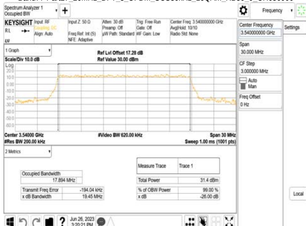
Band77-Part27_20MHz_DFT_s_OFDM_SCS30kHz_16QAM_RB50_0_CH636000
