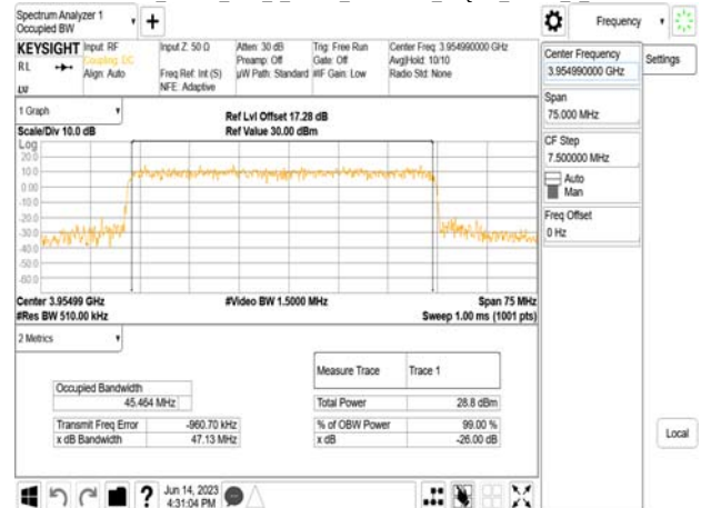
Band77-Part27_50MHz_DFT_s_OFDM_SCS30kHz_16QAM_RB128_0_CH663666
