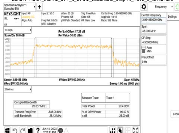
Band77-Part27_30MHz_DFT_s_OFDM_SCS30kHz_16QAM_RB75_0_CH664332
