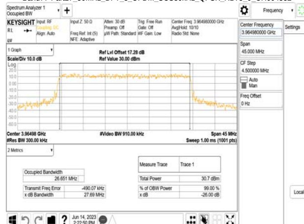
Band77-Part27_30MHz_DFT_s_OFDM_SCS30kHz_QPSK_RB75_0_CH664332
