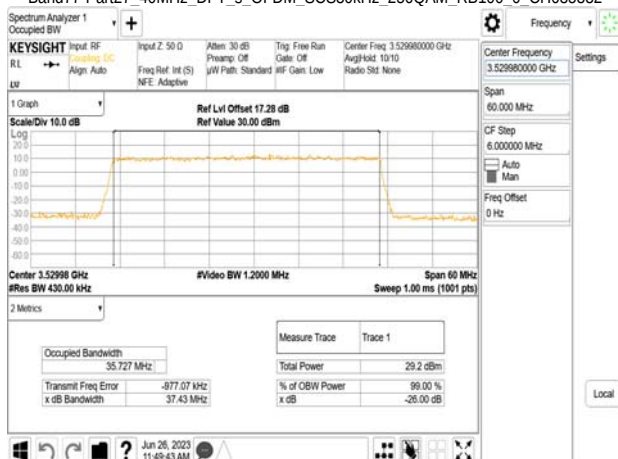
Band77-Part27 40MHz_DFT_s_OFDM_SCS30kHz_256QAM_RB100_0_CH635332
