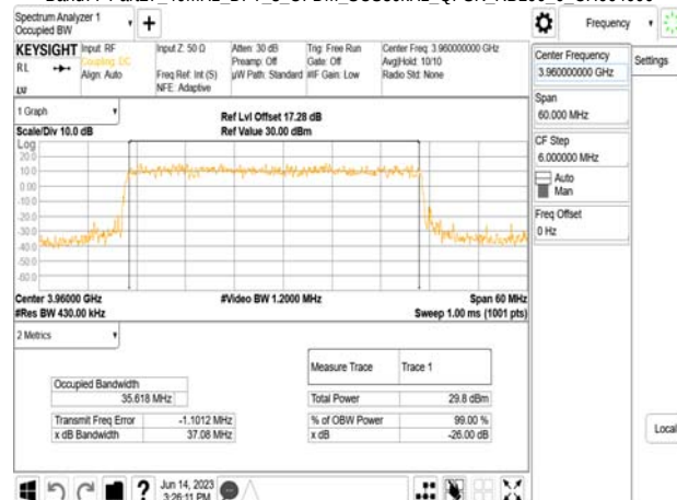
Band77-Part27_40MHz_DFT_s_OFDM_SCS30kHz_QPSK_RB100_0_CH664000
