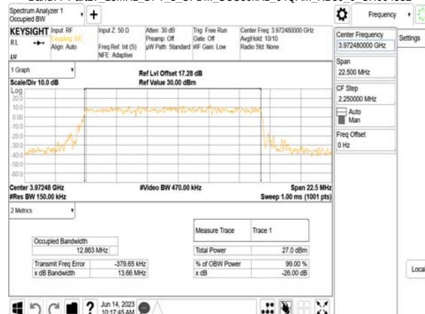
Band77-Part27_15MHz_DFT_s_OFDM_SCS30kHz_64QAM_RB36_0_CH664832
