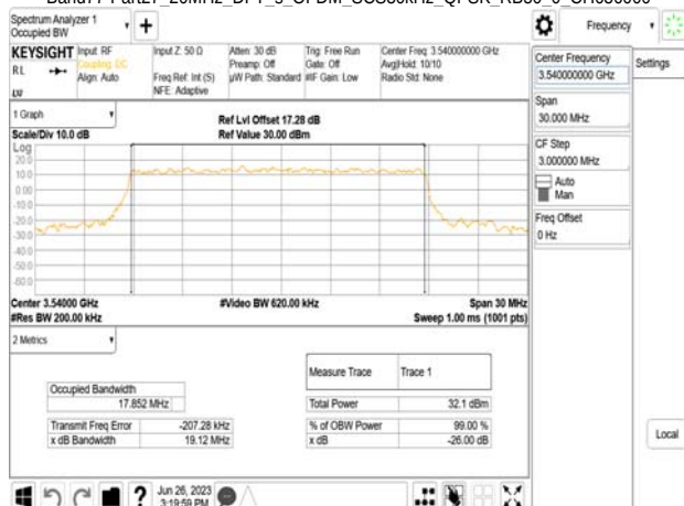
Band77-Part27_20MHz_DFT_s_OFDM_SCS30kHz_QPSK_RB50_0_CH636000
