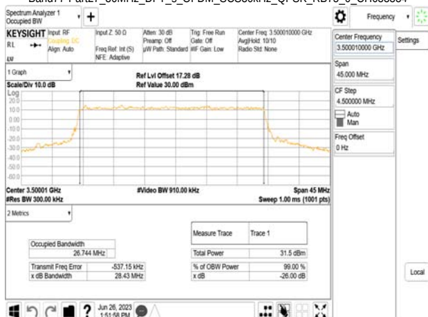
Band77-Part27_30MHz_DFT_s_OFDM_SCS30kHz_QPSK_RB75_0_CH635666
