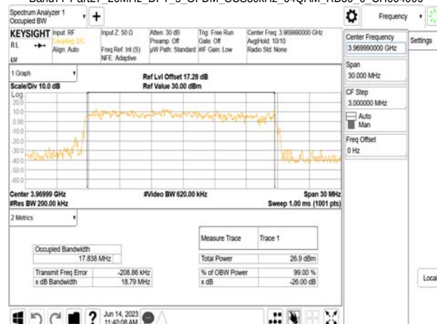
Band77-Part27_20MHz_DFT_s_OFDM_SCS30kHz_64QAM_RB50_0_CH664666
