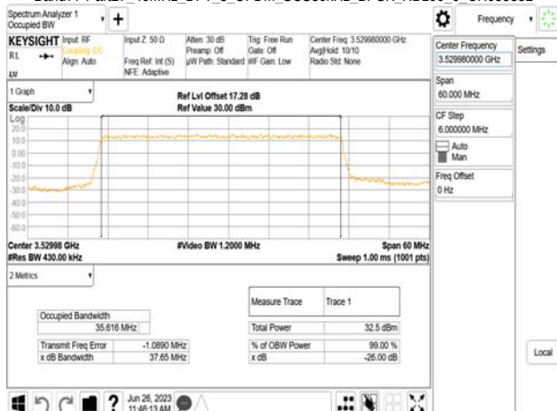
Band77-Part27_40MHz_DFT_s_OFDM_SCS30kHz_BPSK_RB100_0_CH635332
