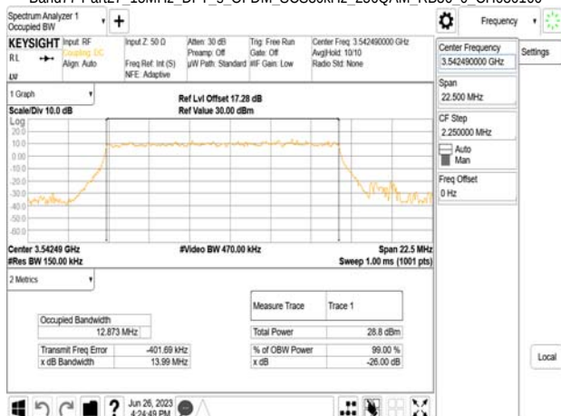
Band77-Part27_15MHz_DFT_s_OFDM_SCS30kHz_256QAM_RB36_0_CH636166
