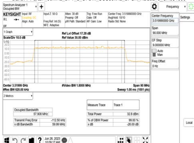
Band77-Part27_60MHz_DFT_s_OFDM_SCS30kHz_BPSK_RB162_0_CH634666
