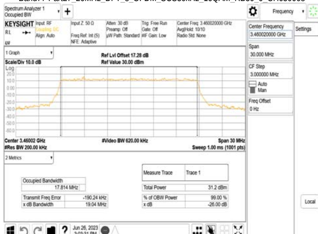
Band77-Part27_20MHz_DFT_s_OFDM_SCS30kHz_16QAM_RB50_0_CH633334
