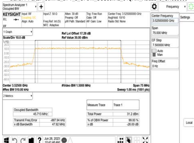
Band77-Part27_50MHz_DFT_s_OFDM_SCS30kHz_64QAM_RB128_0_CH635000
