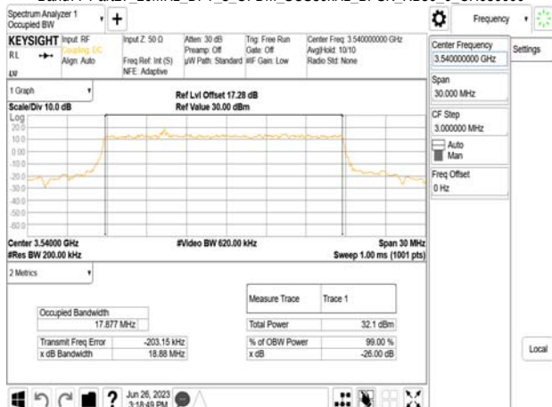
Band77-Part27_20MHz_DFT_s_OFDM_SCS30kHz_BPSK_RB50_0_CH636000
