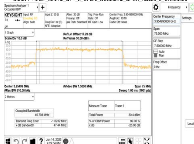
Band77-Part27_50MHz_DFT_s_OFDM_SCS30kHz_BPSK_RB128_0_CH663666
