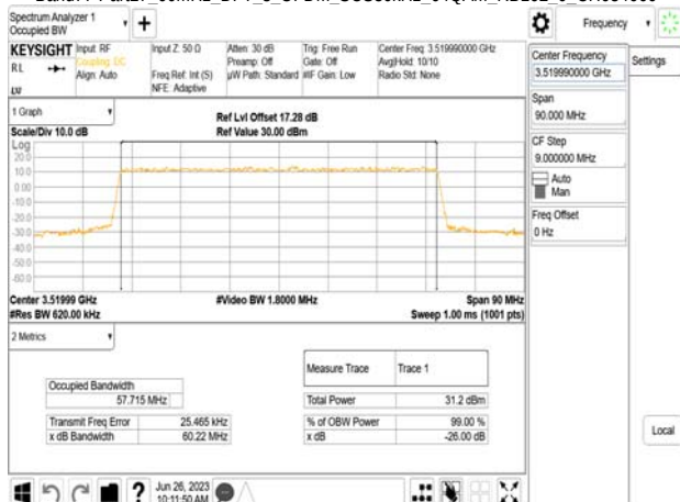
Band77-Part27_60MHz_DFT_s_OFDM_SCS30kHz_64QAM_RB162_0_CH634666
