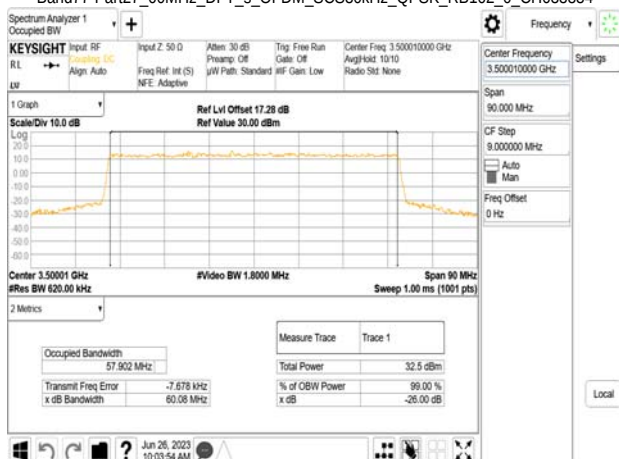
Band77-Part27_60MHz_DFT_s_OFDM_SCS30kHz_QPSK_RB162_0_CH634666
