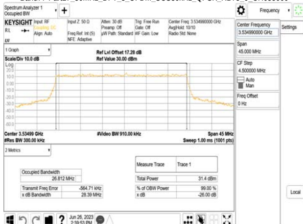
Band77-Part27_30MHz_DFT_s_OFDM_SCS30kHz_QPSK_RB75_0_CH635666
