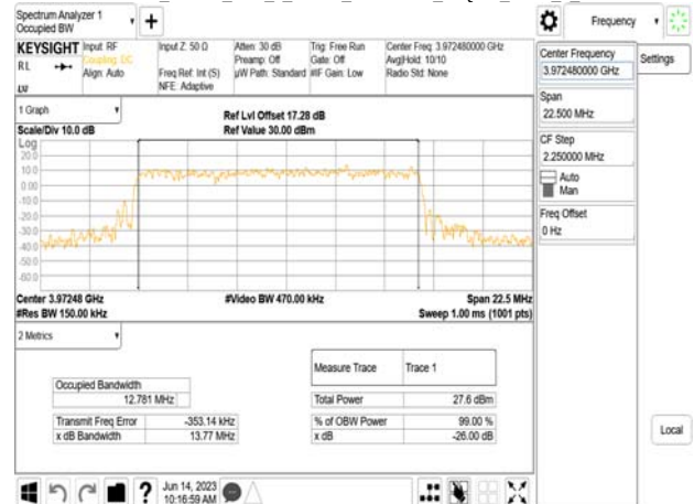
Band77-Part27_15MHz_DFT_s_OFDM_SCS30kHz_16QAM_RB36_0_CH664832
