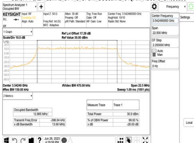
Band77-Part27_15MHz_DFT_s_OFDM_SCS30kHz_64QAM_RB36_0_CH636166
