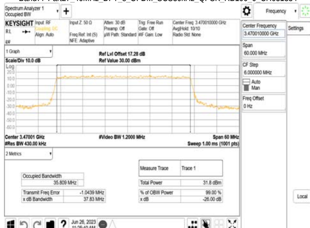
Band77-Part27_40MHz_DFT_s_OFDM_SCS30kHz_QPSK_RB100_0_CH633332
