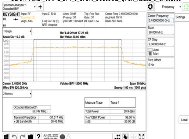
Band77-Part27_60MHz_DFT_s_OFDM_SCS30kHz_QPSK_RB162_0_CH633334
