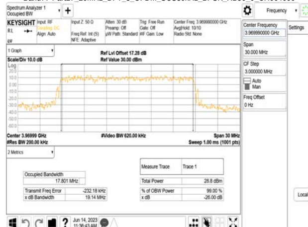
Band77-Part27_20MHz_DFT_s_OFDM_SCS30kHz_BPSK_RB50_0_CH664666
