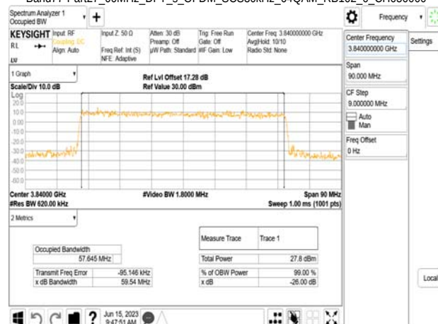
Band77-Part27_60MHz_DFT_s_OFDM_SCS30kHz_64QAM_RB162_0_CH663332
