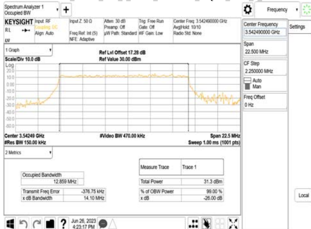
Band77-Part27_15MHz_DFT_s_OFDM_SCS30kHz_16QAM_RB36_0_CH636166
