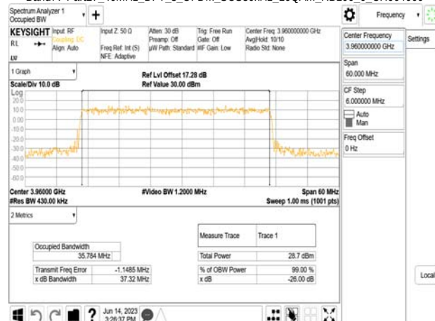
Band77-Part27 40MHz_DFT_s_OFDM_SCS30kHz_16QAM_RB100_0_CH664000
