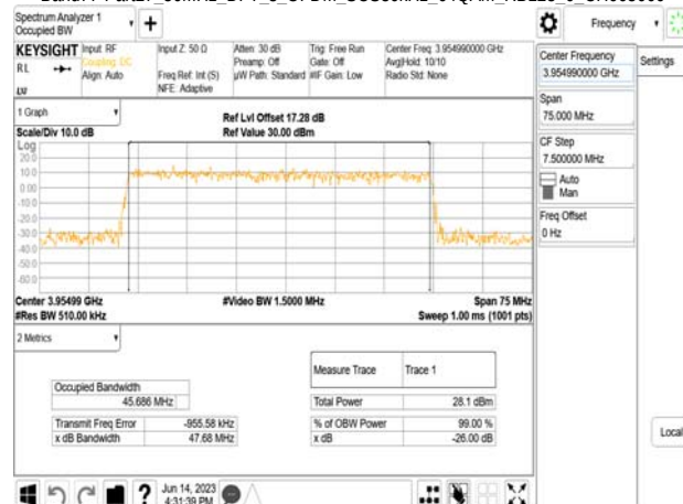
Band77-Part27_50MHz_DFT_s_OFDM_SCS30kHz_64QAM_RB128_0_CH663666
