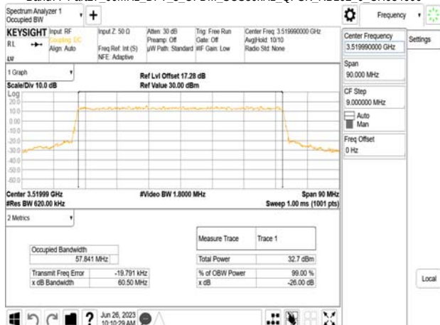
Band77-Part27_60MHz_DFT_s_OFDM_SCS30kHz_QPSK_RB162_0_CH634666
