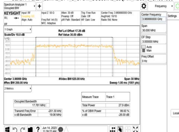
Band77-Part27_20MHz_DFT_s_OFDM_SCS30kHz_16QAM_RB50_0_CH664666
