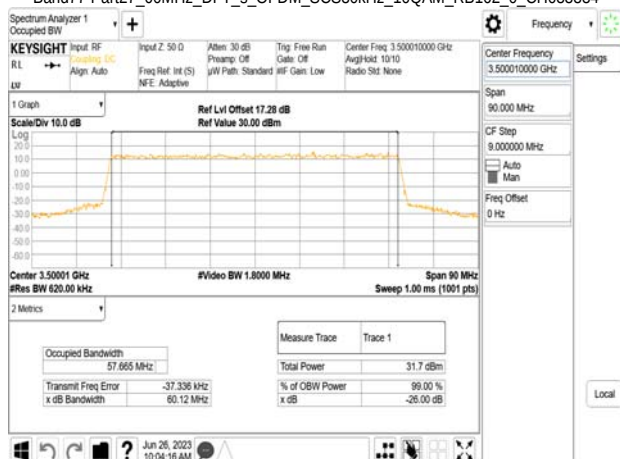
Band77-Part27_60MHz_DFT_s_OFDM_SCS30kHz_16QAM_RB162_0_CH634666
