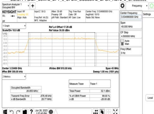
Band77-Part27_30MHz_DFT_s_OFDM_SCS30kHz_BPSK_RB75_0_CH635666
