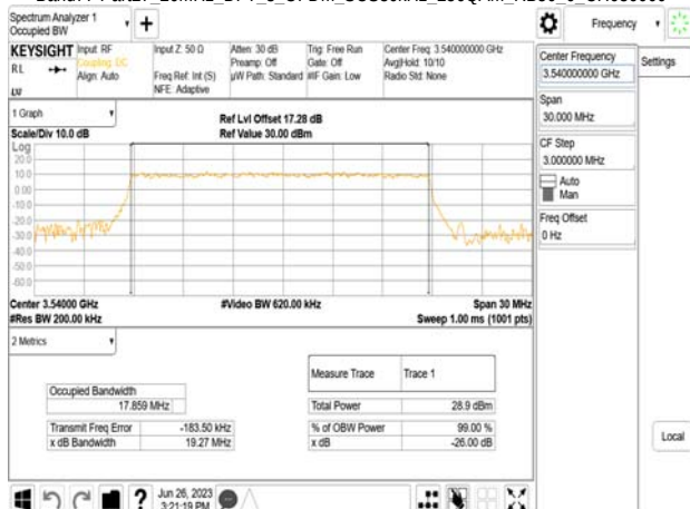
Band77-Part27_20MHz_DFT_s_OFDM_SCS30kHz_256QAM_RB50_0_CH636000
