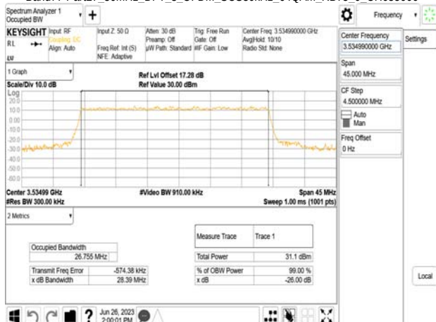
Band77-Part27_30MHz_DFT_s_OFDM_SCS30kHz_64QAM_RB75_0_CH635666
