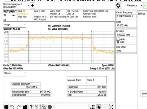
Band77-Part27_30MHz_DFT_s_OFDM_SCS30kHz_BPSK_RB75_0_CH664332
