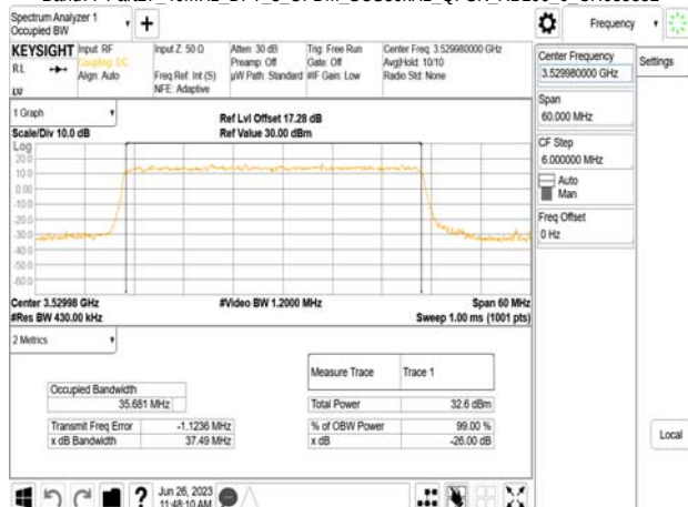
Band77-Part27_40MHz_DFT_s_OFDM_SCS30kHz_QPSK_RB100_0_CH635332
