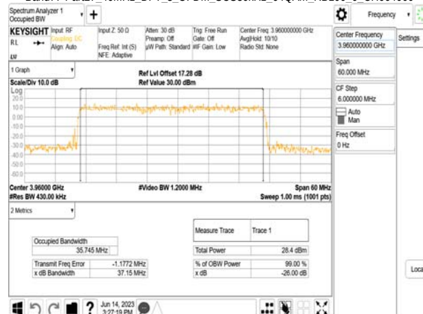
Band77-Part27 40MHz_DFT_s_OFDM_SCS30kHz_64QAM_RB100_0_CH664000
