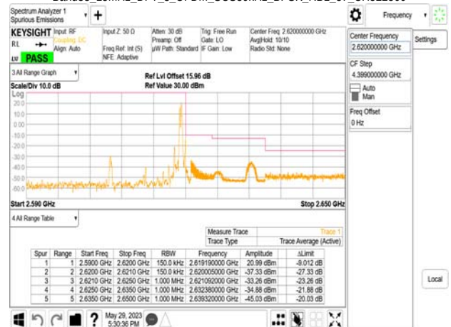
Band38_15MHz_DFT_s_OFDM_SCS30kHz_BPSK_RB1_37_CH522500
