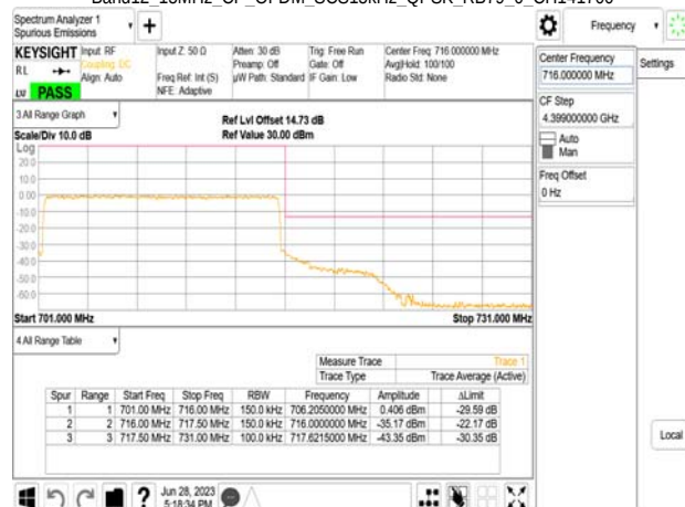
Band12 15MHz_CP_OFDM_SCS15kHz_QPSK_RB79_0_CH141700
