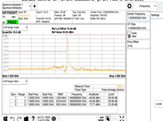
Band25_30MHz_CP_OFDM_SCS15kHz_QPSK_RB1_0_CH373000
