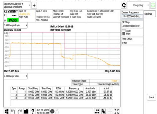
Band25_10MHz_DFT_s_OFDM_SCS15kHz_BPSK_RB50_0_CH382000
