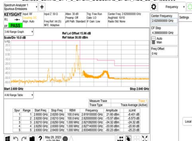
Band38 10MHz DFT_s_OFDM_SCS30kHz_BPSK_RB24_0_CH515000
