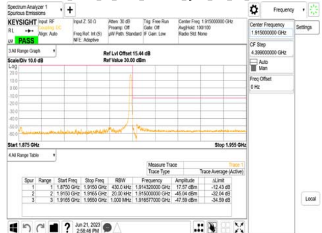
Band25 40MHz CP_OFDM_SCS15kHz_QPSK_RB1_215_CH379000
