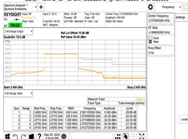
Band7 40MHz_CP_OFDM_SCS15kHz_QPSK_RB216_0_CH510000
