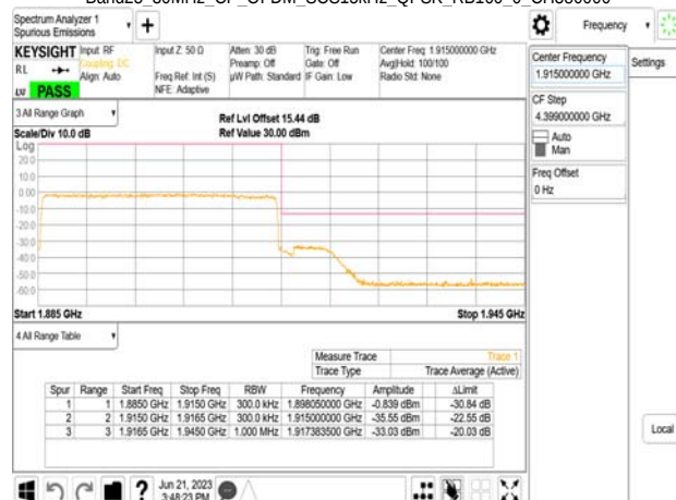
Band25_30MHz_CP_OFDM_SCS15kHz_QPSK_RB160_0_CH380000
