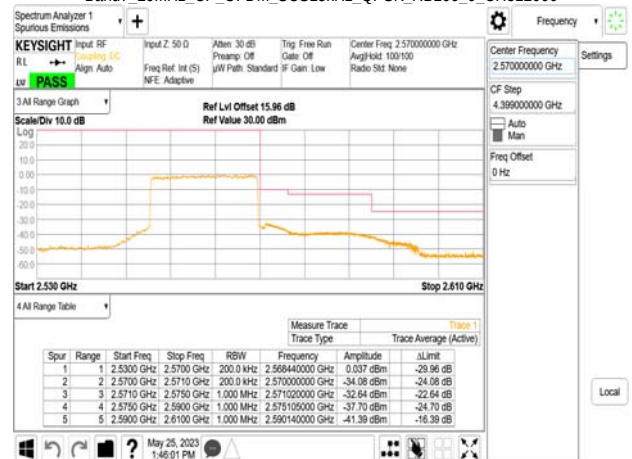
Band7 20MHz_CP_OFDM_SCS15kHz_QPSK_RB106_0_CH512000
