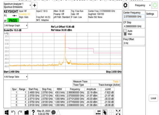
Band7_40MHz_DFT_s_OFDM_SCS15kHz_BPSK_RB1_215_CH510000
