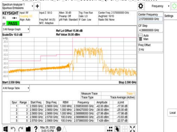
Band38_10MHz_CP_OFDM_SCS30kHz_QPSK_RB24_0_CH515000
