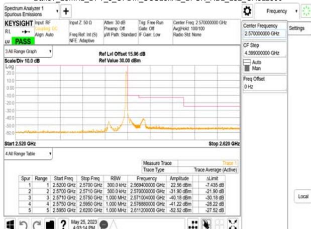
Band7_25MHz_DFT_s_OFDM_SCS15kHz_BPSK_RB128_0_CH502500
