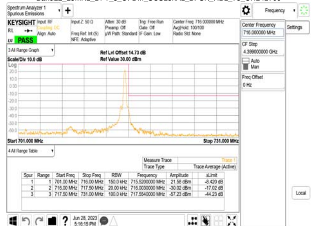
Band12_15MHz_DFT_s_OFDM_SCS15kHz_BPSK_RB1_78_CH141700
