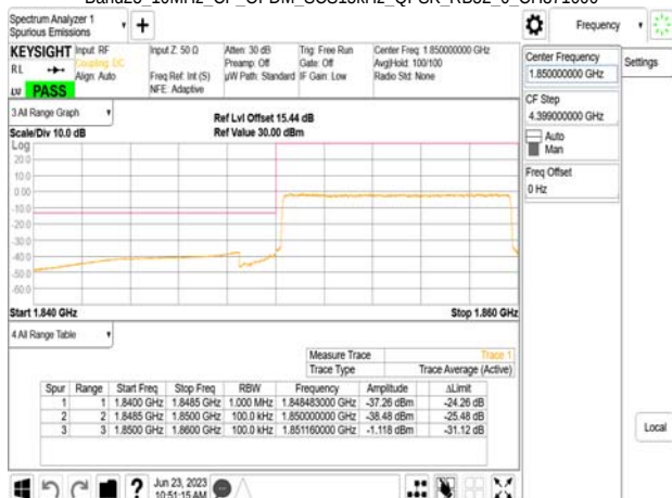
Band25_10MHz_CP_OFDM_SCS15kHz_QPSK_RB52_0_CH371000
