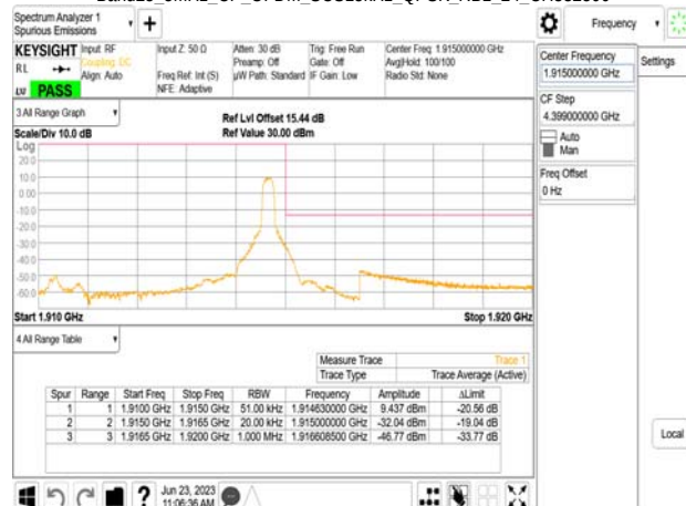
Band25 5MHz_CP_OFDM_SCS15kHz_QPSK_RB1_24_CH382500
