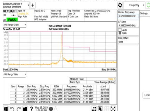
Band7_20MHz_DFT_s_OFDM_SCS15kHz_BPSK_RB1_105_CH512000
