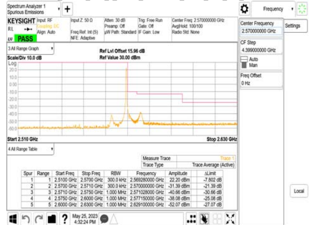
Band7_30MHz_DFT_s_OFDM_SCS15kHz_BPSK_RB160_0_CH503000
