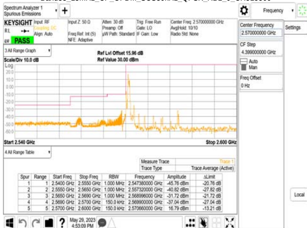
Band38 15MHz_CP_OFDM_SCS30kHz_QPSK_RB1_0_CH515500
