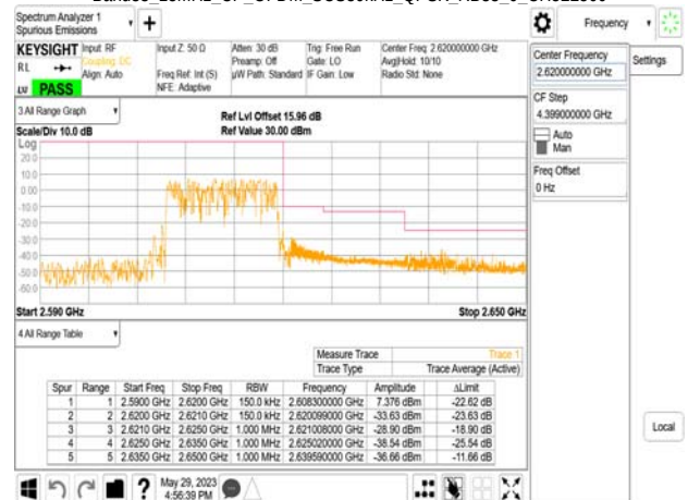
Band38 15MHz_CP_OFDM_SCS30kHz_QPSK_RB38_0_CH522500
