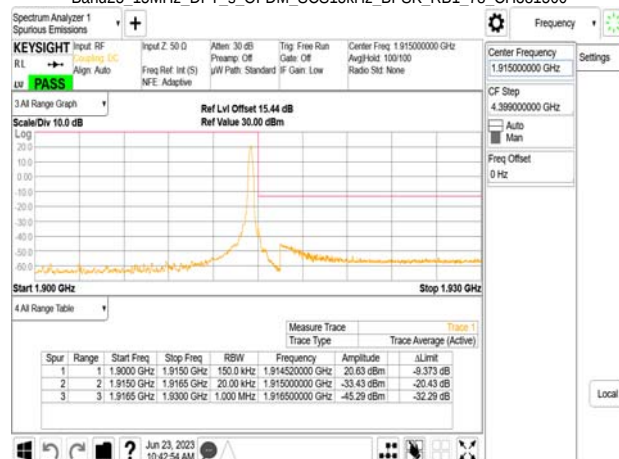
Band25_15MHz_DFT_s_OFDM_SCS15kHz_BPSK_RB1_78_CH381500
