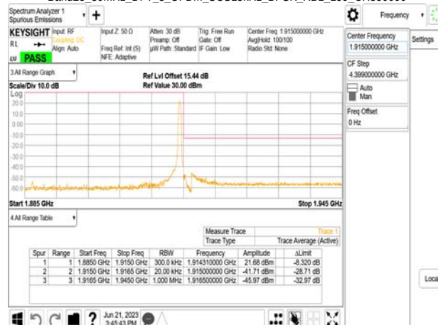
Band25_30MHz_DFT_s_OFDM_SCS15kHz_BPSK_RB1_159_CH380000
