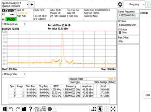
Band25 40MHz DFT_s_OFDM_SCS15kHz_BPSK_RB1_215_CH379000
