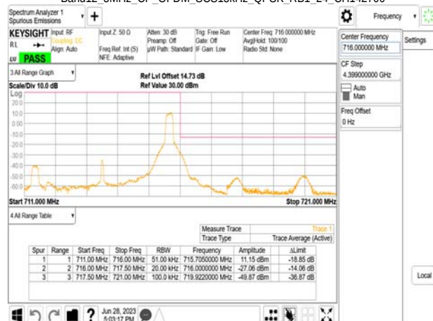
Band12 5MHz_CP_OFDM_SCS15kHz_QPSK_RB1_24_CH142700
