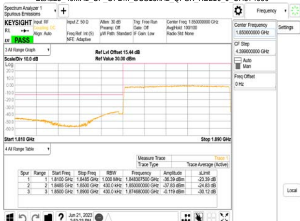
Band25 40MHz CP_OFDM_SCS15kHz_QPSK_RB216_0_CH379000
