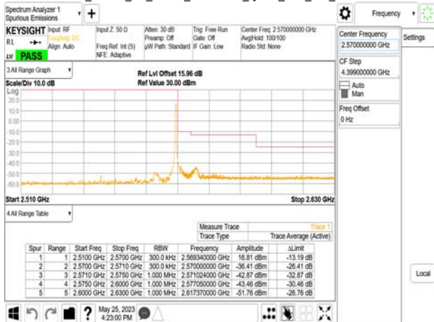
Band7_30MHz_CP_OFDM_SCS15kHz_QPSK_RB160_0_CH503000
