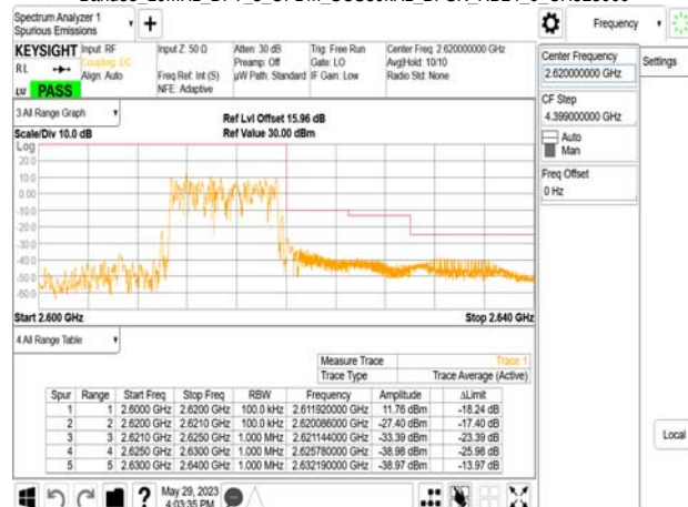
Band38 10MHz DFT_s_OFDM_SCS30kHz_BPSK_RB24_0_CH523000
