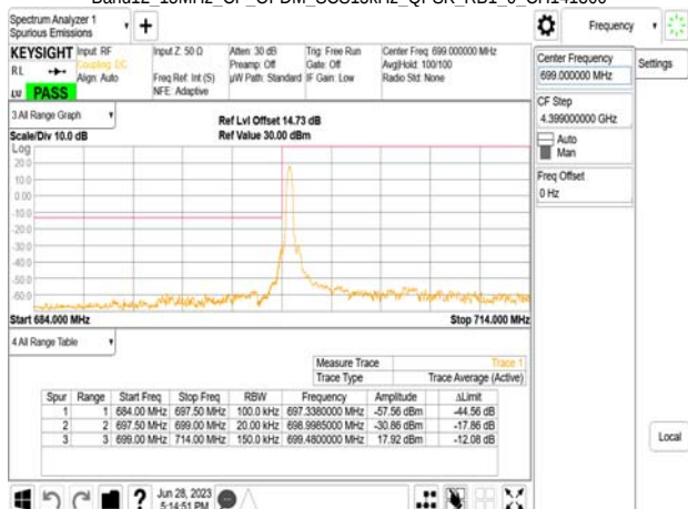
Band12 15MHz_CP_OFDM_SCS15kHz_QPSK_RB1_0_CH141300
