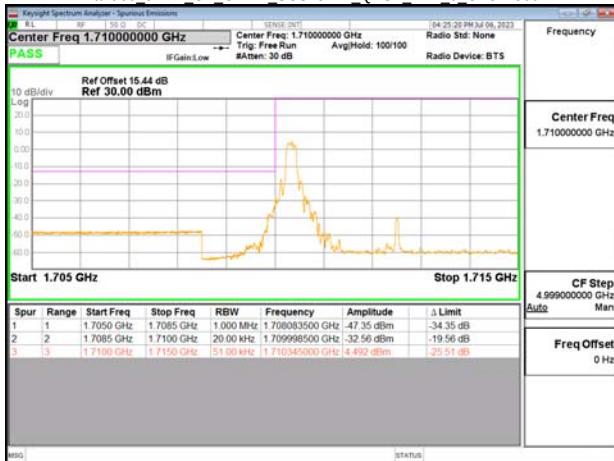
Band66 5MHz CP OFDM SCS15kHz QPSK RB1 0 CH342500
