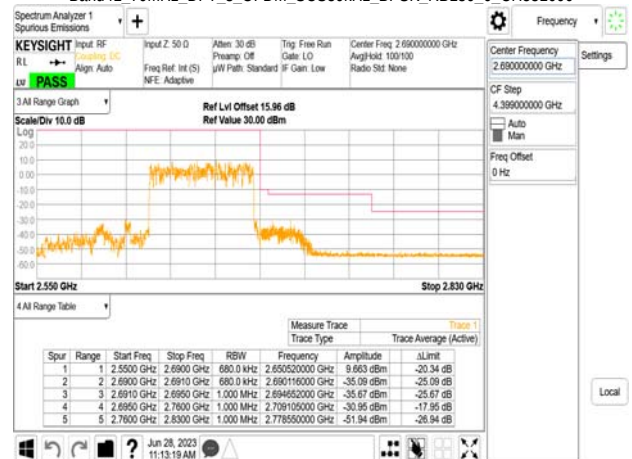
Band41_70MHz_DFT_s_OFDM_SCS30kHz_BPSK_RB180_0_CH531000
