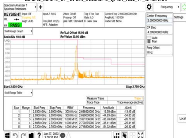
Band41_30MHz_CP_OFDM_SCS30kHz_QPSK_RB1_77_CH534996
