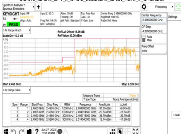
Band41_30MHz_DFT_s_OFDM_SCS30kHz_BPSK_RB75_0_CH502200
