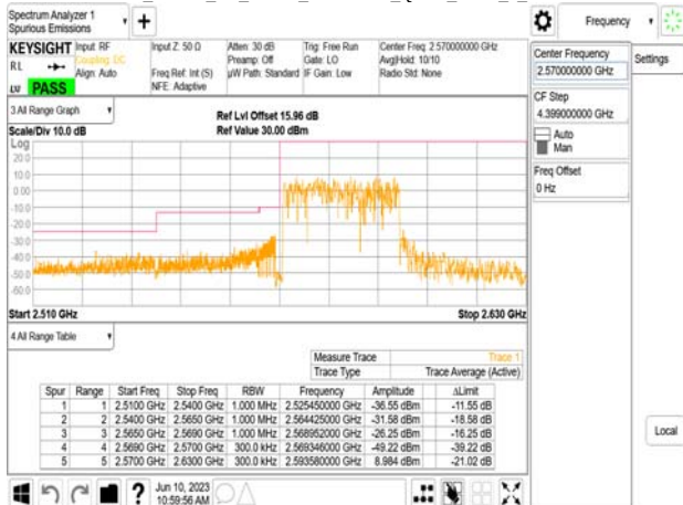
Band38_30MHz_CP_OFDM_SCS30kHz_QPSK_RB78_0_CH517000
