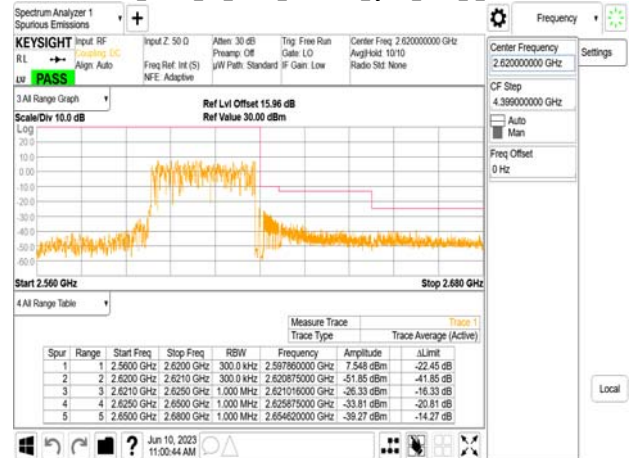
Band38_40MHz_DFT_s_OFDM_SCS30kHz_BPSK_RB1_0_CH518000
