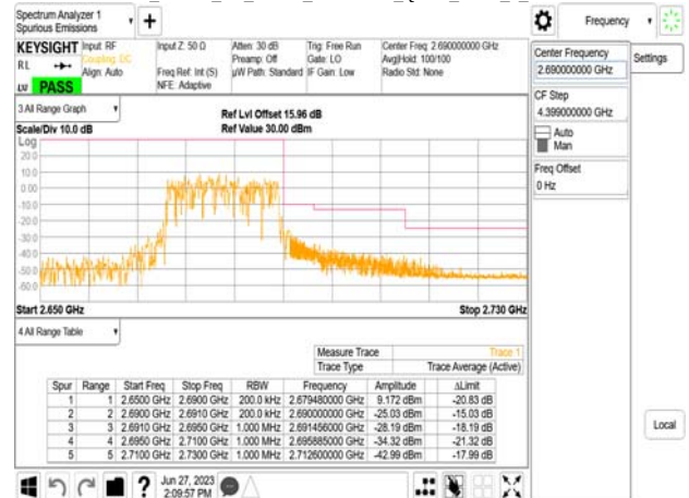
Band41_20MHz_CP_OFDM_SCS30kHz_QPSK_RB51_0_CH535998
