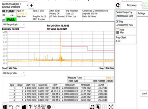
Band41_100MHz_CP_OFDM_SCS30kHz_QPSK_RB273_0_CH509202
