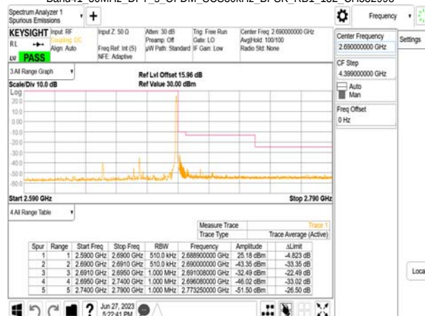
Band41_50MHz_DFT_s_OFDM_SCS30kHz_BPSK_RB1_132_CH532998
