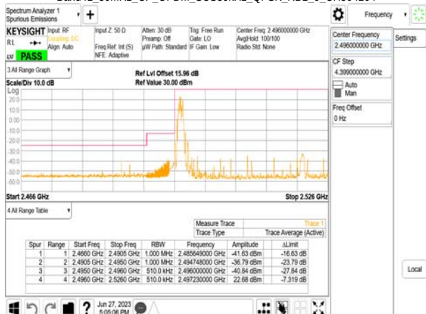
Band41_50MHz_CP_OFDM_SCS30kHz_QPSK_RB1_0_CH504204
