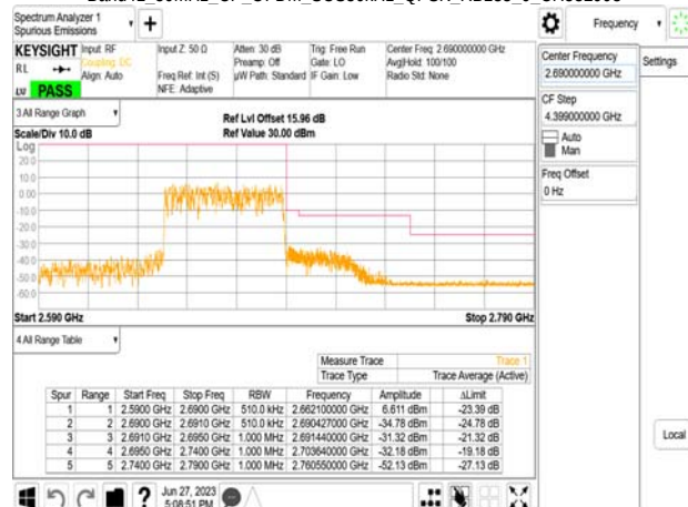
Band41_50MHz_CP_OFDM_SCS30kHz_QPSK_RB133_0_CH532998
