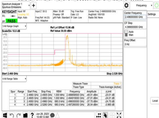
Band41_70MHz_DFT_s_OFDM_SCS30kHz_BPSK_RB1_0_CH506202
