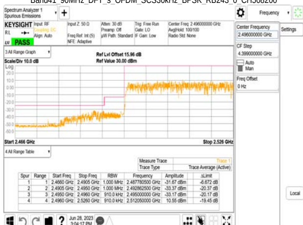
Band41_90MHz_DFT_s_OFDM_SCS30kHz_BPSK_RB243_0_CH508200
