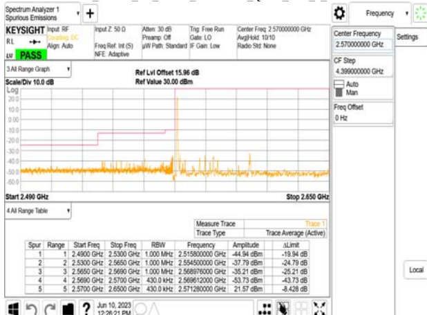
Band38_40MHz_CP_OFDM_SCS30kHz_QPSK_RB1_0_CH518000
