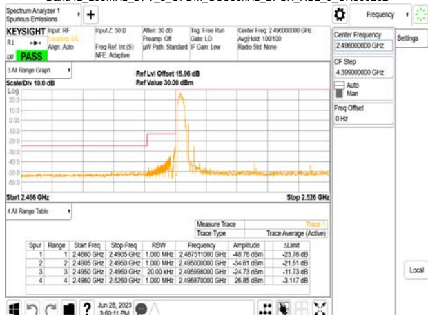
Band41_100MHz_DFT_s_OFDM_SCS30kHz_BPSK_RB1_0_CH509202
