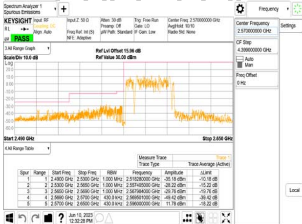
Band38_40MHz_DFT_s_OFDM_SCS30kHz_BPSK_RB100_0_CH520000
