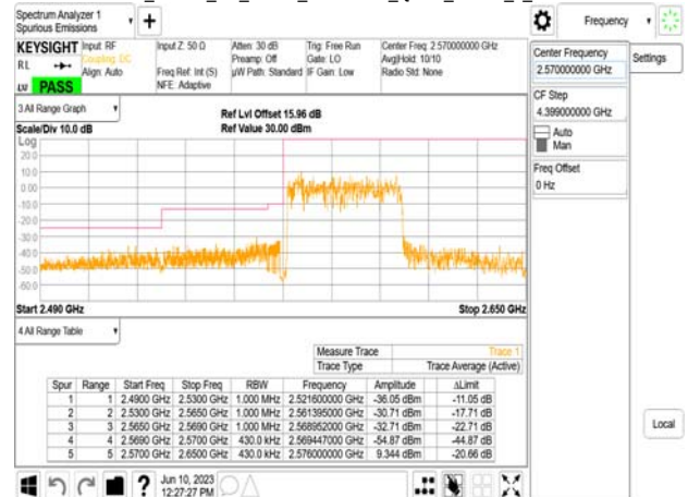
Band38_40MHz_CP_OFDM_SCS30kHz_QPSK_RB106_0_CH520000
