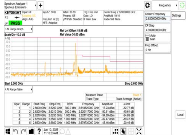
Band38_30MHz_DFT_s_OFDM_SCS30kHz_BPSK_RB75_0_CH517000
