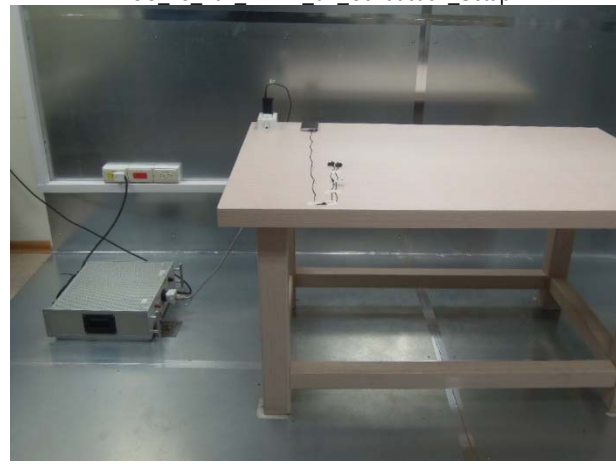
FCC 15 407 WLAN 6E Conduction Setup
