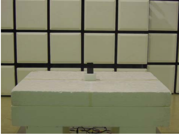
FCC_15_225_NFC_Radiated_Setup
