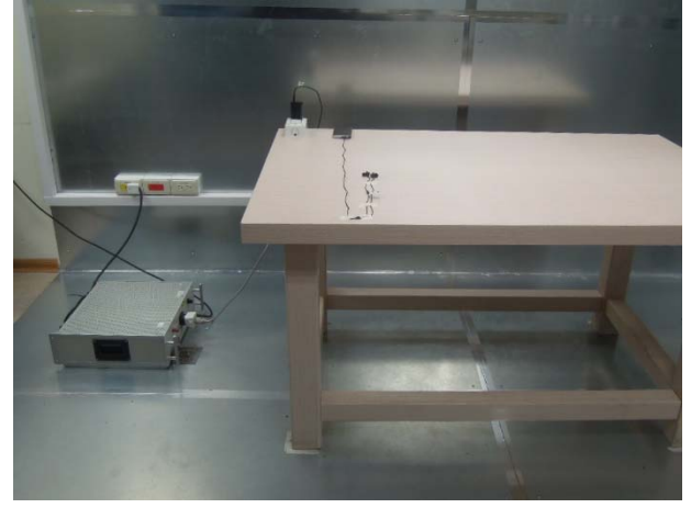
FCC_15_225_NFC_Conduction_Setup
