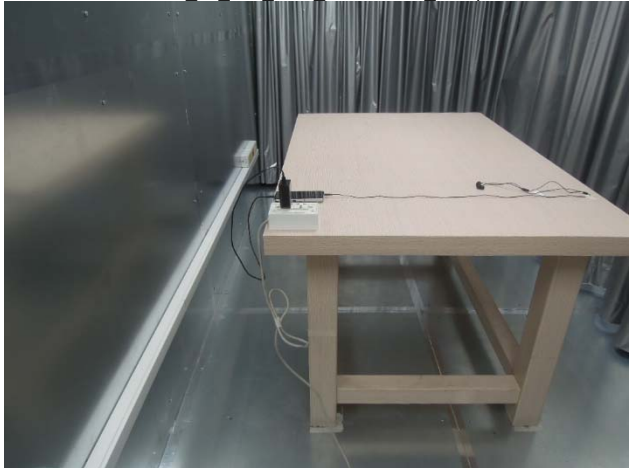
FCC_15_225_NFC_Conduction_Setup
