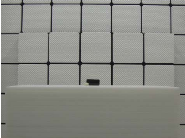
FCC_22_24_27_LTE_ULCA_Radiated_Setup
