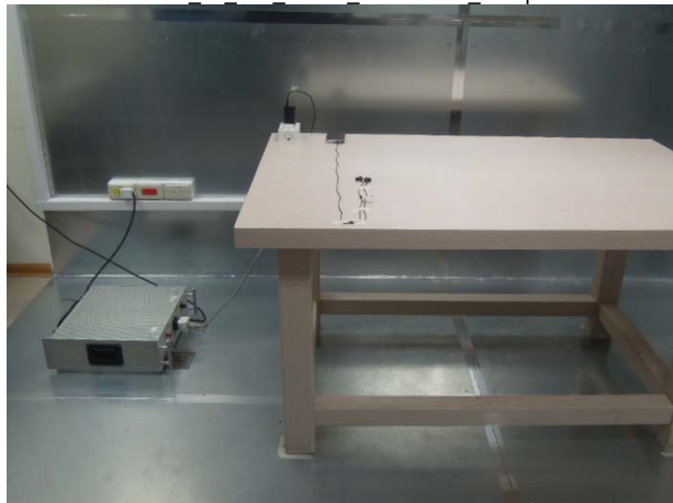
FCC 15 247 WLAN Conduction Setup
