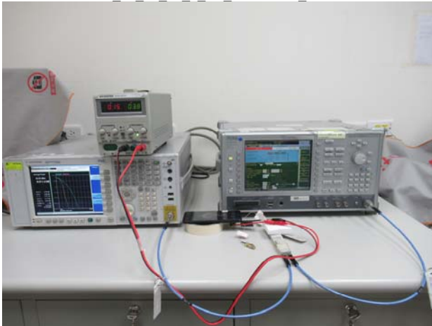
FCC 22 24 27 2 3G Radiated Setup
