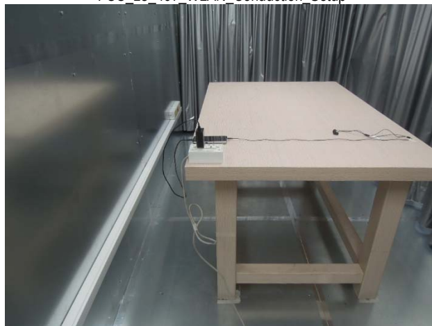
FCC_15_407_WLAN_6E_Conducted_Setup
