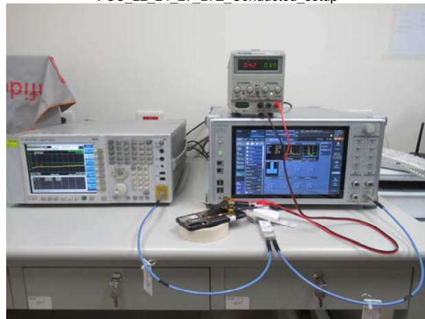
FCC 22 24 27 LTE Radiated Setup
