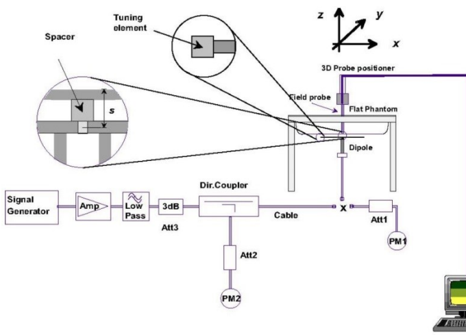
System Performance Check Setup
