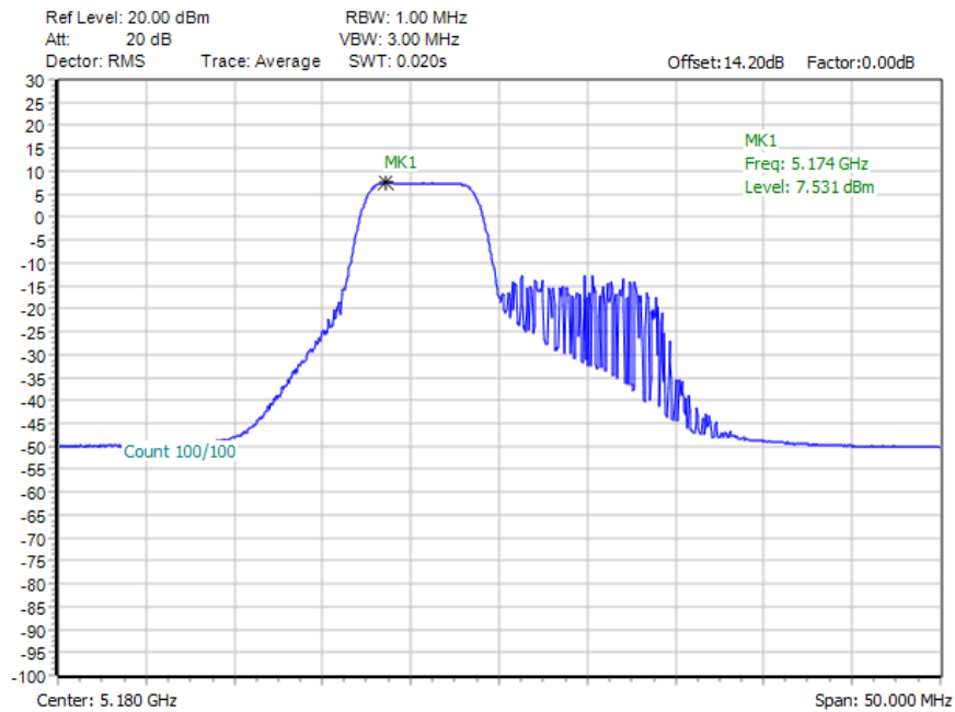
11BE20MIMO_Ant5_5180_106+26_OFDMA_1
