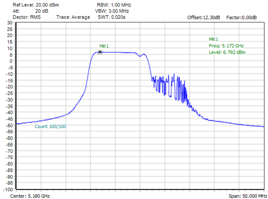
11BE20MIMO_Ant5_5180_106+26_OFDMA_1
