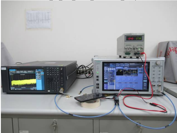
FCC 96_NR_Conducted_Setup
