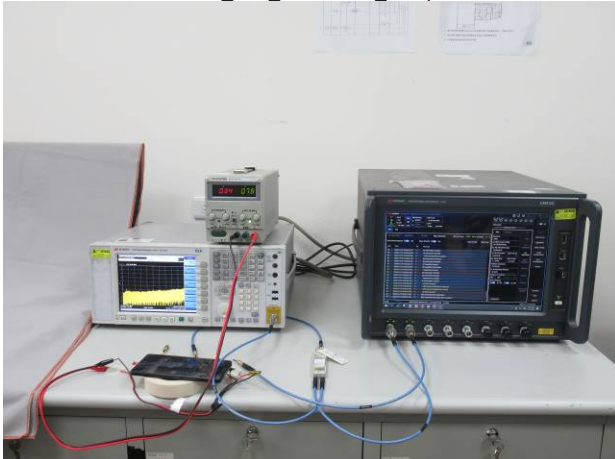
FR1_2TX_Conducted_Setup
