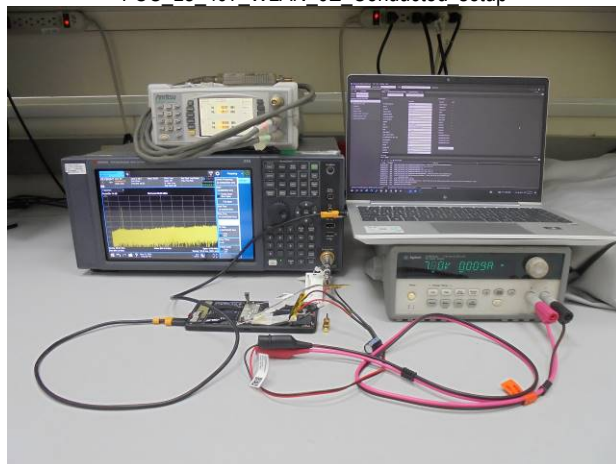
FCC 15 407 WLAN 6E Conducted setup
