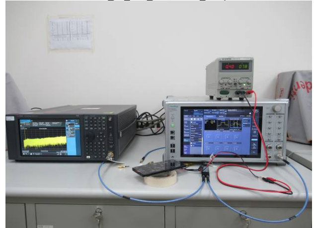
FCC_96_LTE_Conducted_setup
