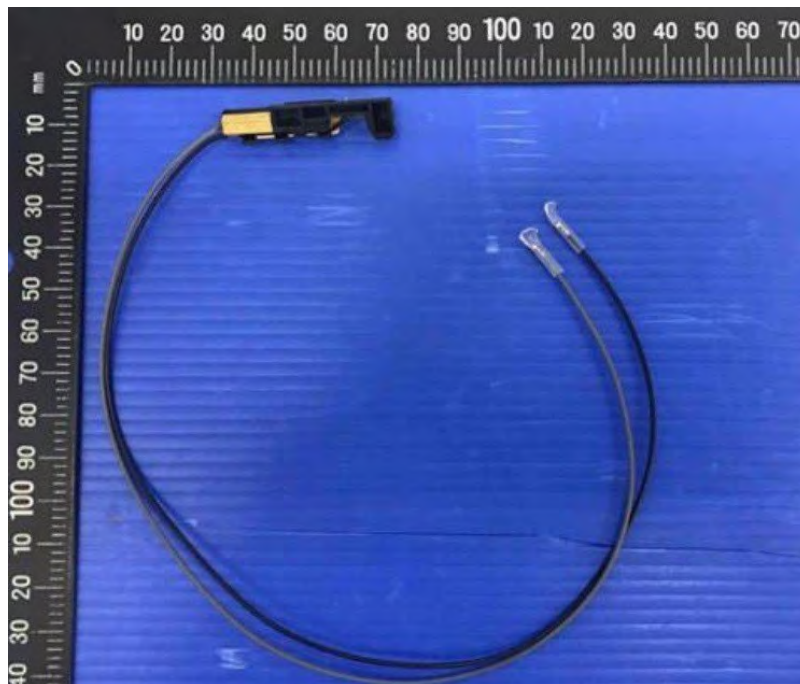
LUXSHARE Main 0 / Main 1 Antenna Part No.: LA9RF274-CS-H ASUS Part No. 14008-04150100
