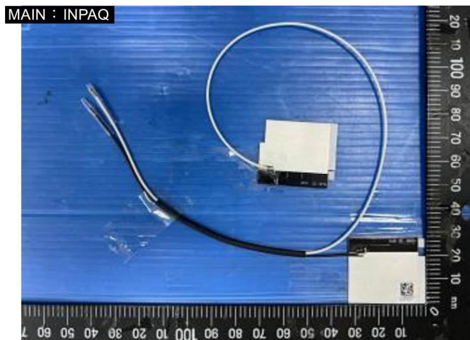
EUT Photo (42)
