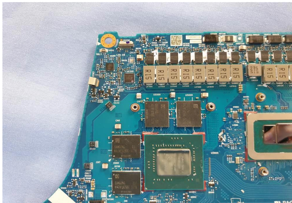
EUT Photo (22)
