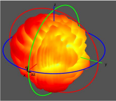
Max Antenna 3D Radiation Pattern 5250-5350 MHz
