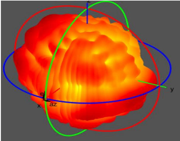
Max Antenna 3D Radiation Pattern 6425-6525 MHz
