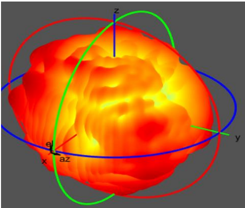
Max Antenna 3D Radiation Pattern 6525-6875 MHz
