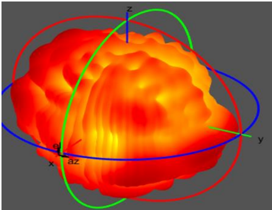
Max Antenna 3D Radiation Pattern 6525-6875 MHz
