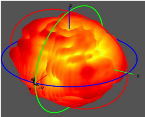
Max Antenna 3D Radiation Pattern 6425-6525 MHz
