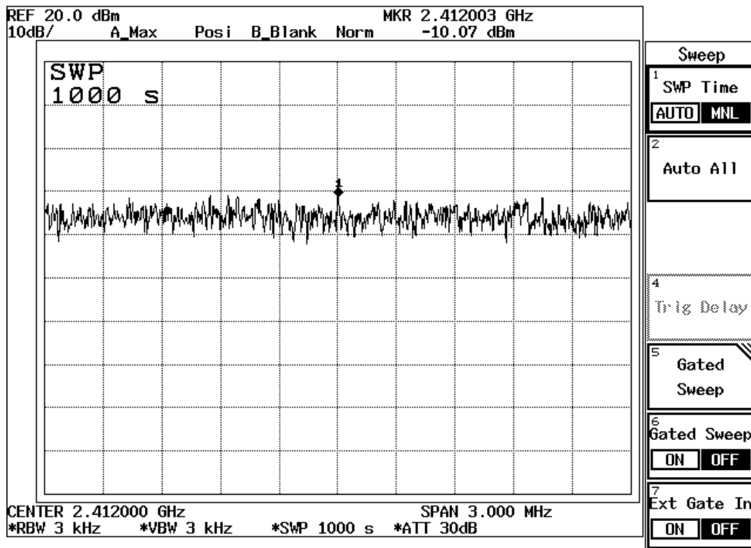
Figure Channel 1: 11Mbps
