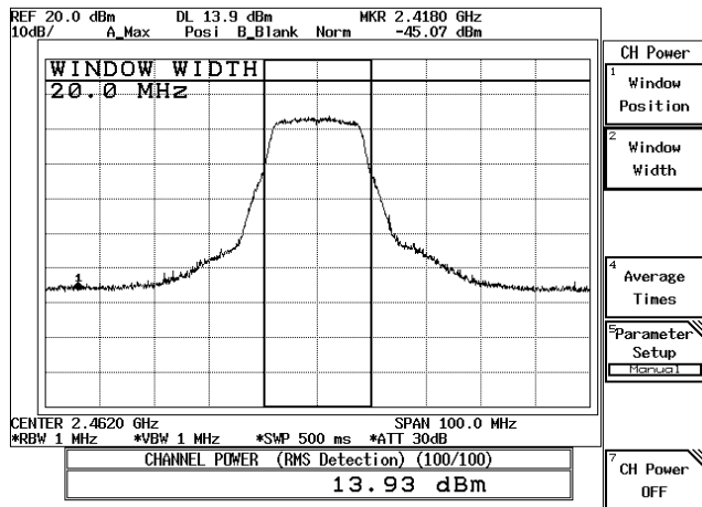
54Mbps-CH11
