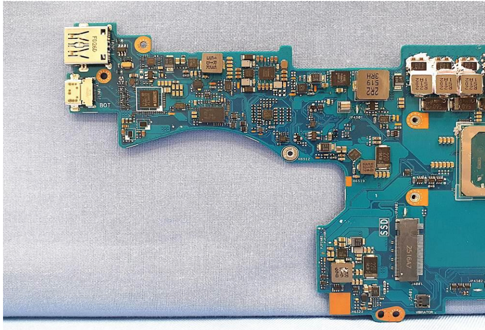
EUT Photo (22)
