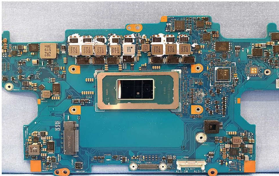
EUT Photo (22)
