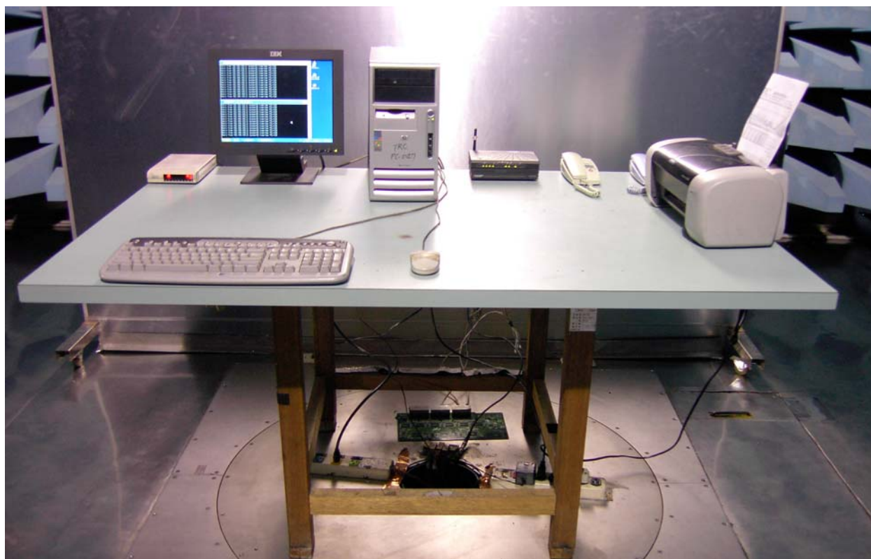
Front View of the Test Configuration
