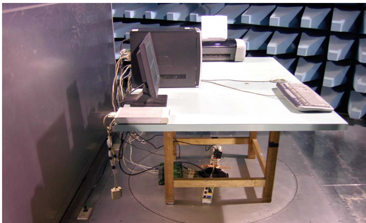
Side View of the Test Configuration
