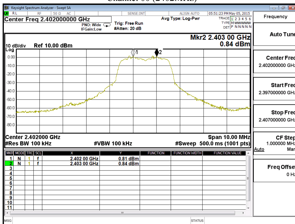
Channel 00 (2402MHz)
