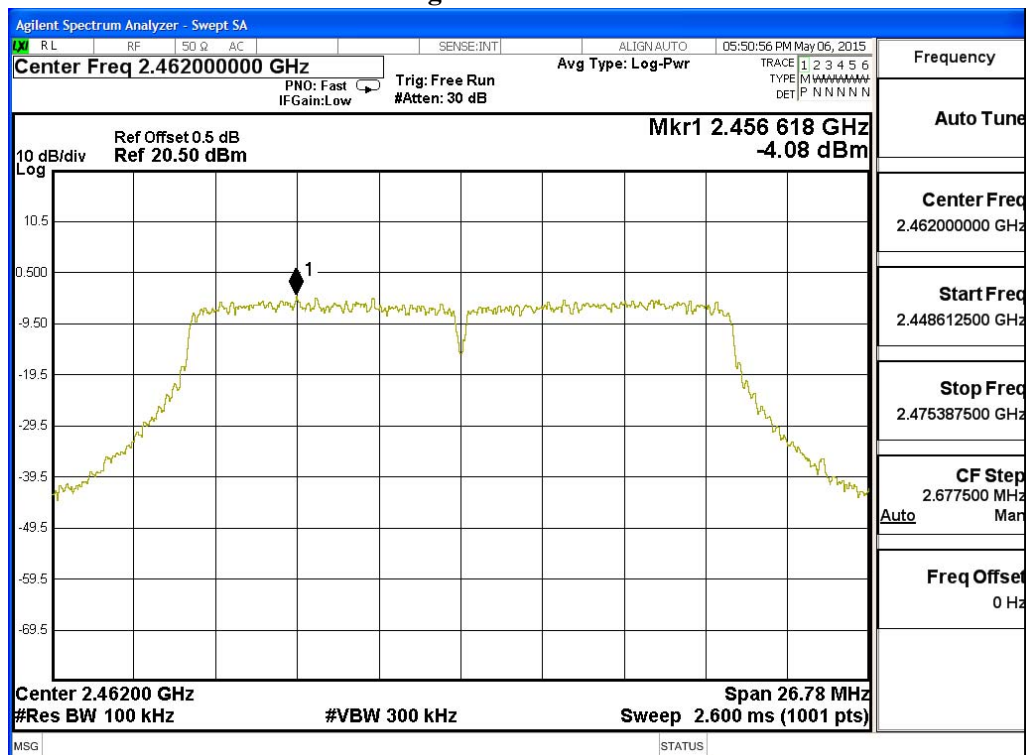
Figure Channel 11:
