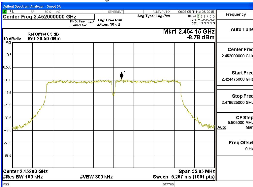
Figure Channel 09:
