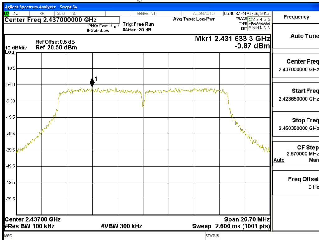
Figure Channel 06:
