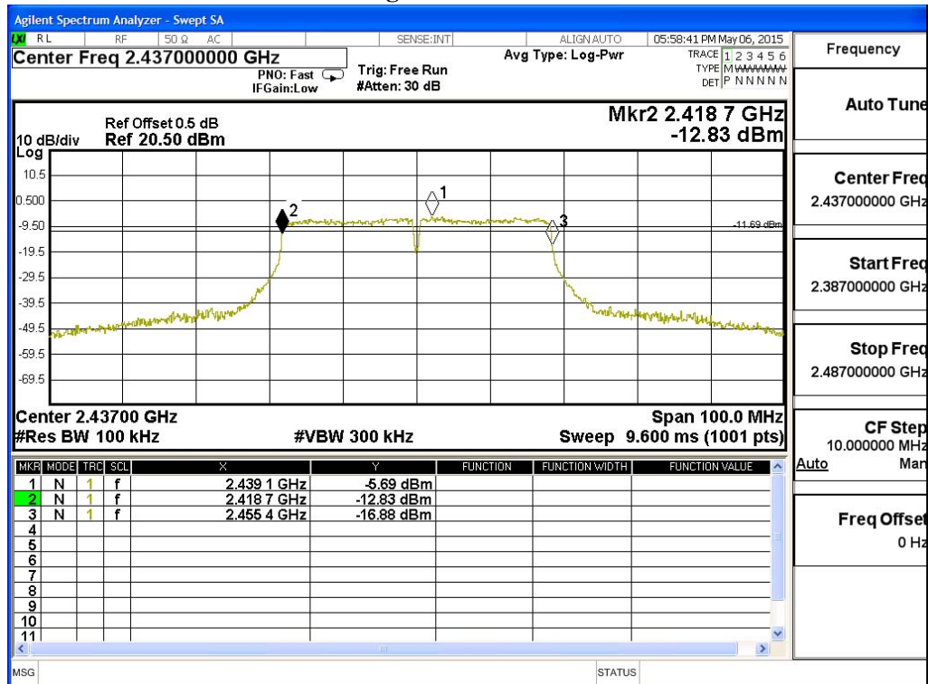
Figure Channel 06:
