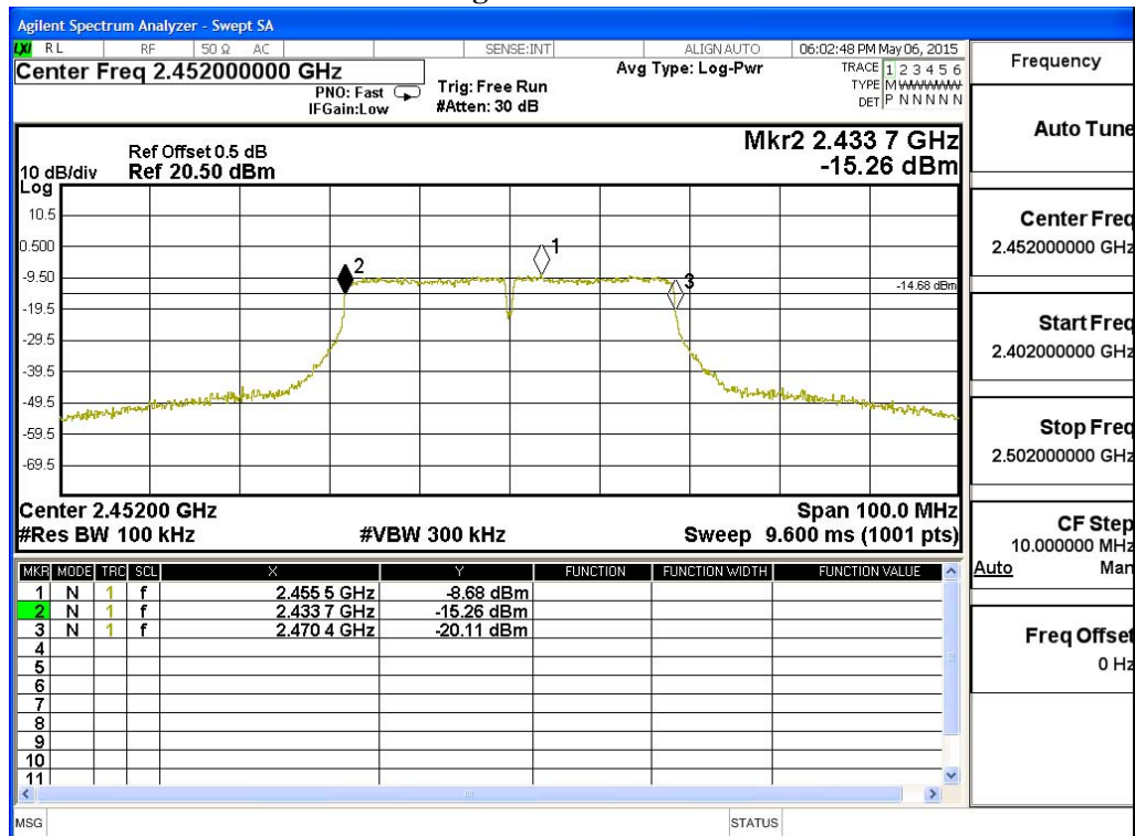
Figure Channel 09:
