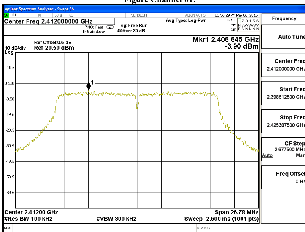
Figure Channel 01:
