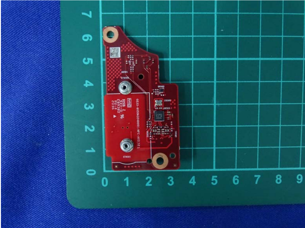
(15) EUT Photo (NFC PCB Board)
