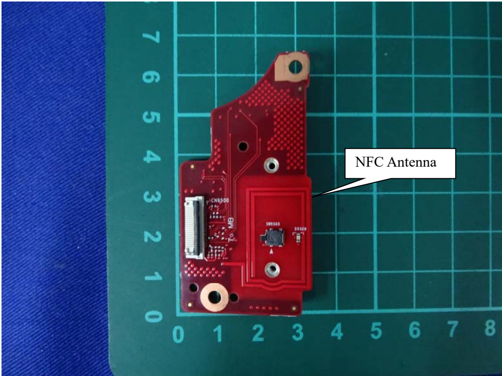
(16) EUT Photo (NFC PCB Board)
