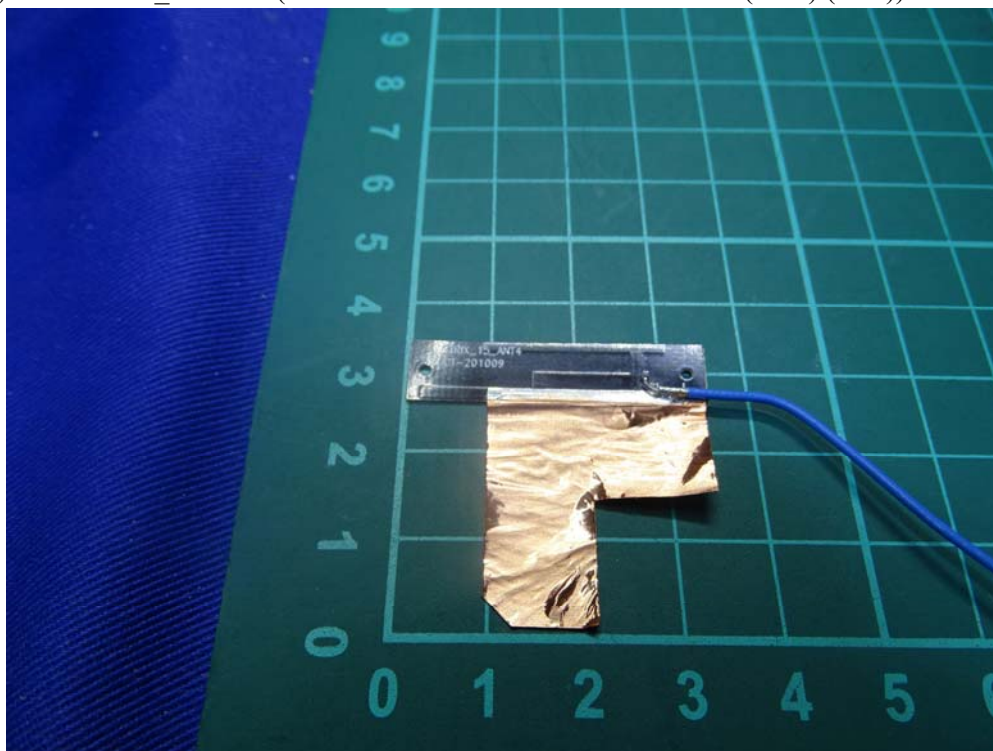
(66) EUT Photo_Antenna (LUXSHARE / LA9RF309-CS-H TX4 (Blue) (Aux))
