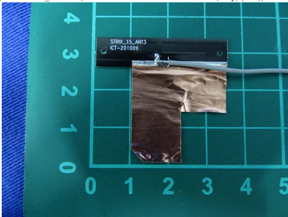
(64) EUT Photo_Antenna (LUXSHARE / LA9RF308-CS-H TX3 (Gray) (Aux))
