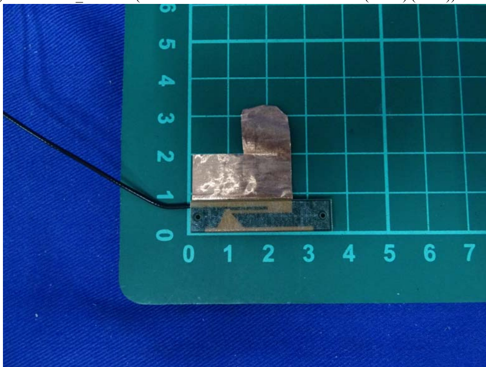
(61) EUT Photo_Antenna (LUXSHARE / LA9RF306-CS-H TX1 (Black) (Main))
