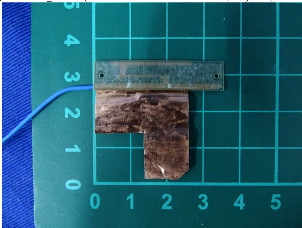
(67) EUT Photo_Antenna (LUXSHARE / LA9RF309-CS-H TX4 (Blue) (Aux))
