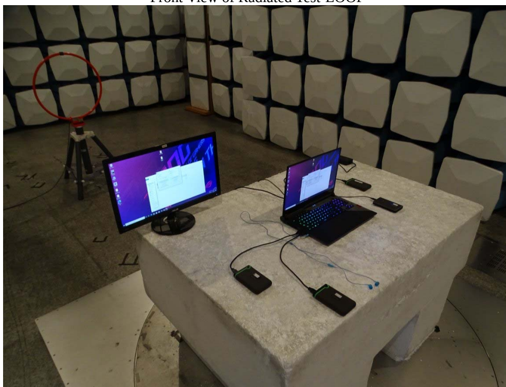
Front View of Radiated Test-LOOP
