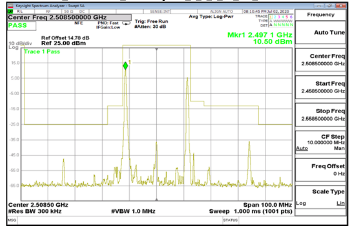
Mask LTE\Band41 25MHz\QPSK 100 0 25 0 CH Low2508.5
