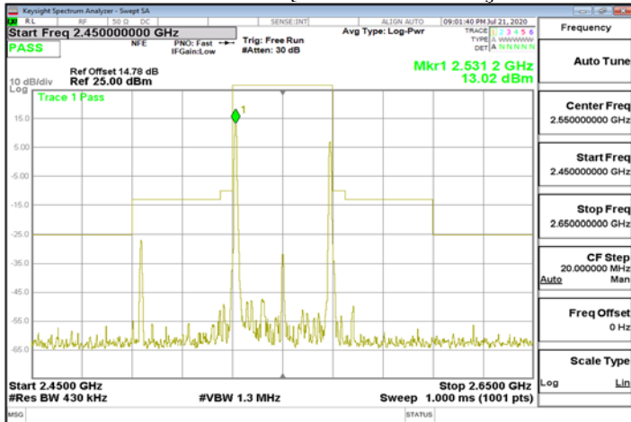
Mask LTE\Band7 40MHz\QPSK 100 0 100 0 CH High 2550
