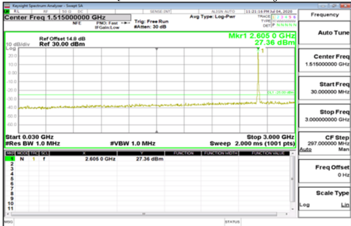
Emission Band38 30MHz QPSK 1 74 1 0 30MHz~3GHz CH HighCH38150-2610
