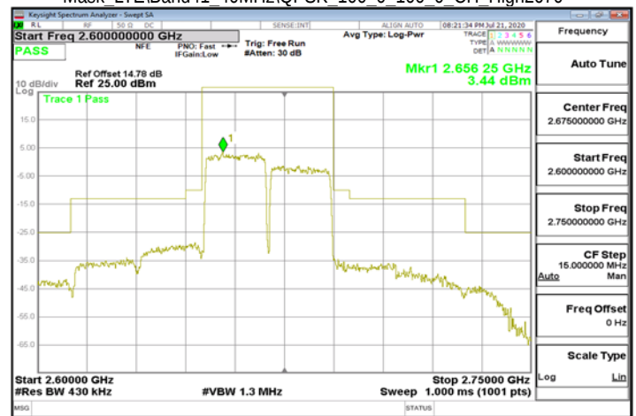
Mask LTE\Band41 40MHz\QPSK 100 0 100 0 CH High2670
