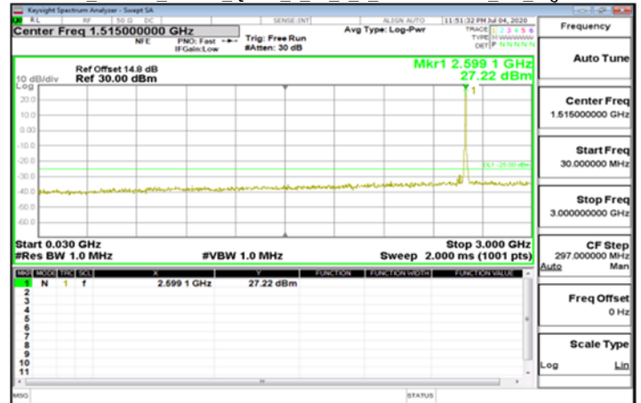
Emission Band38 40MHz QPSK 1 99 1 0 30MHz~3GHz CH High 2600
