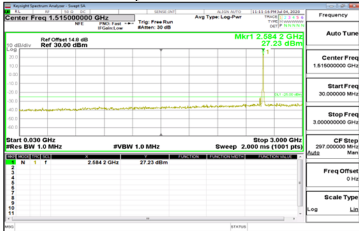
Emission Band38 30MHz QPSK 1 74 1 0 30MHz~3GHz CH Mid 2595
