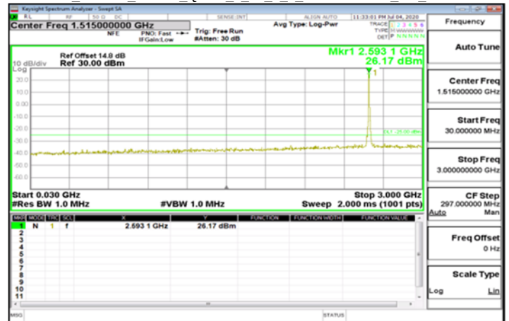
Emission Band38 40MHz QPSK 1 99 1 0 30MHz~3GHz CH Mid 2595
