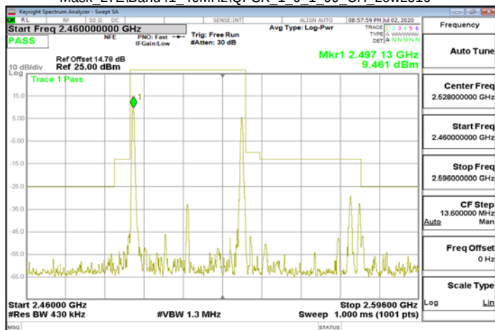
Mask LTE\Band41 40MHz\QPSK 1 0 1 99 CH Low2516
