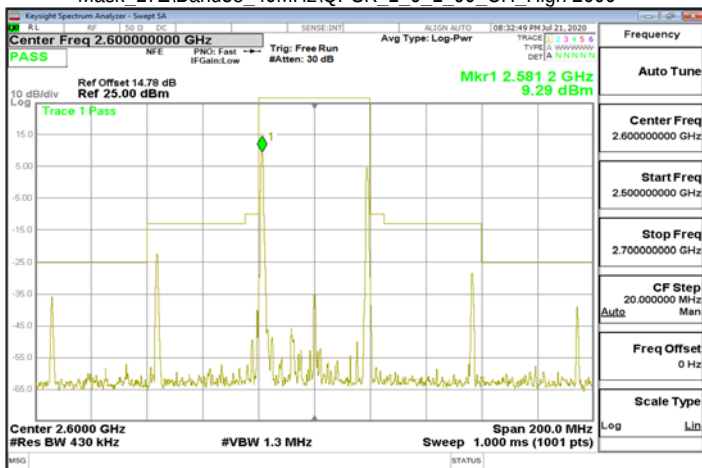
Mask LTE\Band38 40MHz\QPSK 1 0 1 99 CH High 2600
