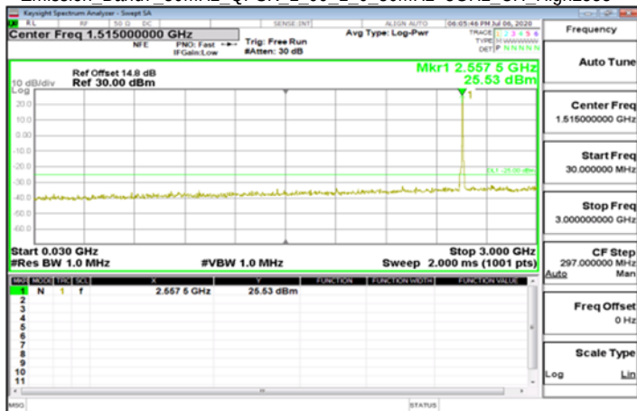
Emission Band7 30MHz QPSK 1 99 1 0 30MHz-3GHz CH High2555
