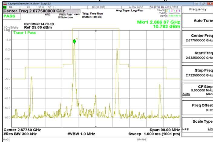
Mask LTE\Band41 25MHz\QPSK 100 0 25 0 CH High2677.5
