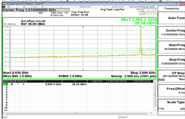
Emission Band41 25MHz QPSK 1 99 1 0 30MHz~3GHz CH High 2677.5
