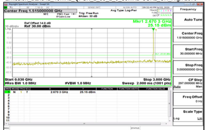
Emission Band41 40MHz QPSK 1 99 1 0 30MHz~3GHz CH High 2670
