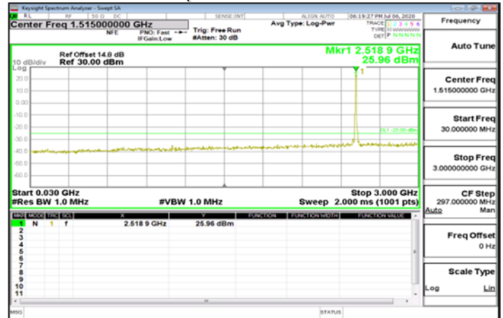
Emission Band7 40MHz QPSK 1 99 1 0 30MHz-3GHz CH Mid2535
