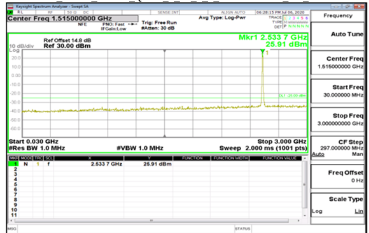
Emission Band7 40MHz QPSK 1 99 1 0 30MHz-3GHz CH High2550
