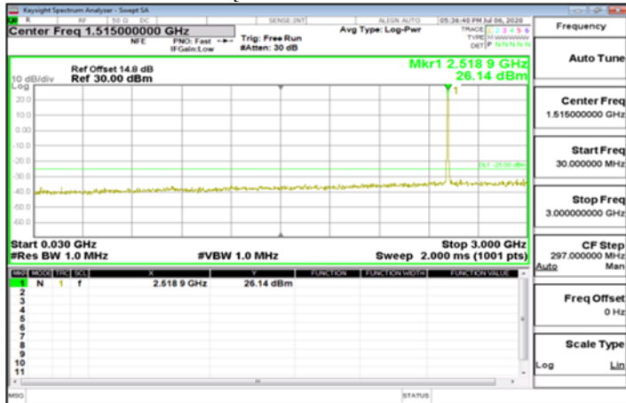
Emission Band7 30MHz QPSK 1 99 1 0 30MHz-3GHz CH Mid2535
