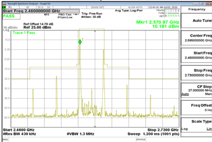
Mask LTE\Band38 40MHz\QPSK 100 0 100 0 CH Low 2590
