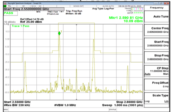
Mask LTE\Band38 30MHz\QPSK 75 0 75 0 CH High 2605
