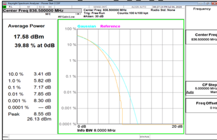
Band5_20MHz_256QAM_50_0_50_0_Mid836.5
