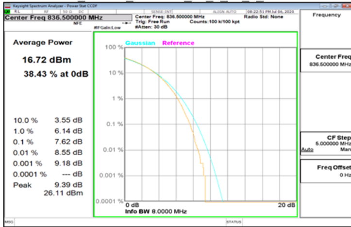
Band5_15MHz_256QAM_50_0_25_0_Mid836.5
