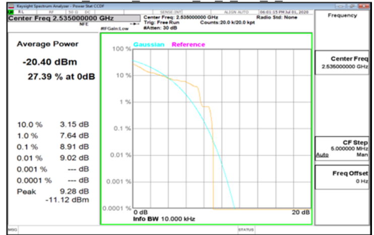
Band7_30MHz_256QAM_100_0_50_0_Mid2535
