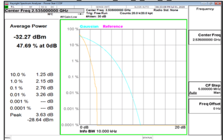
Band7_40MHz_256QAM_100_0_100_0_Mid2535
