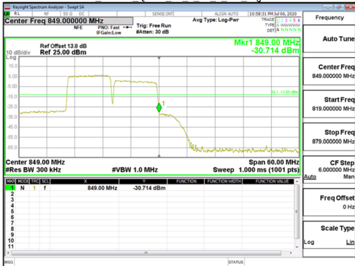
Band5 20MHz QPSK 50 0 50 0 CH High839
