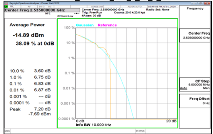
Band7_40MHz_256QAM_100_0_100_0_Mid2535
