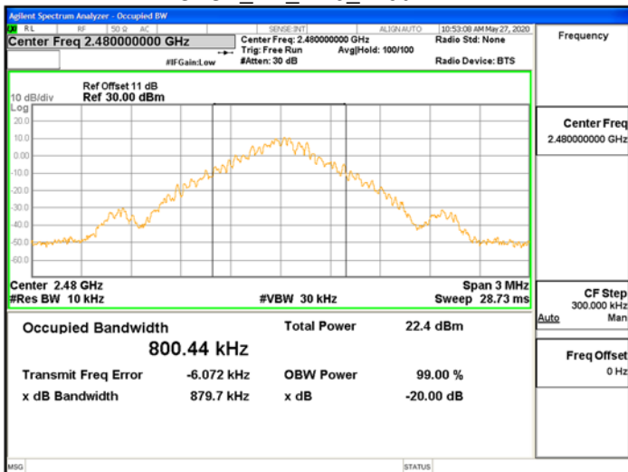
GFSK_1M_DH5_2480MHz
