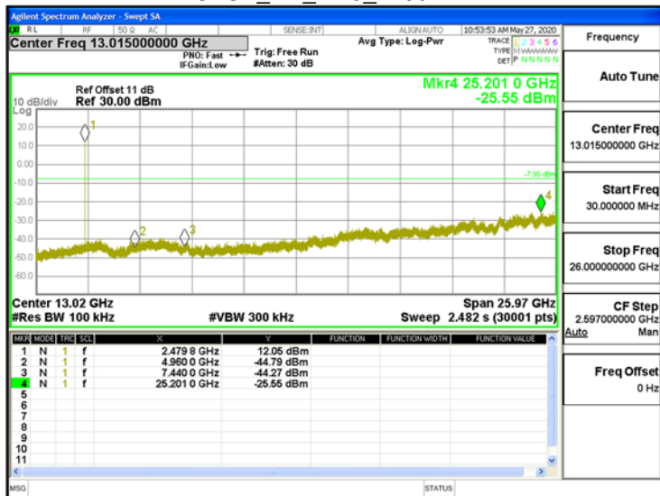
GFSK_1M_DH5_2480MHz
