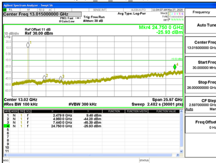
\pi/4 DQPSK_2M_DH5_2480MHz
