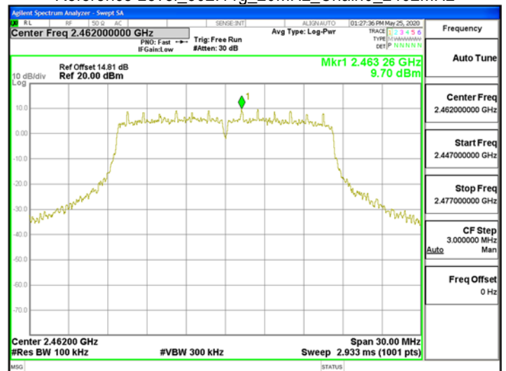
Reference Level_802.11g_20MHz_Chain0_2462MHz
