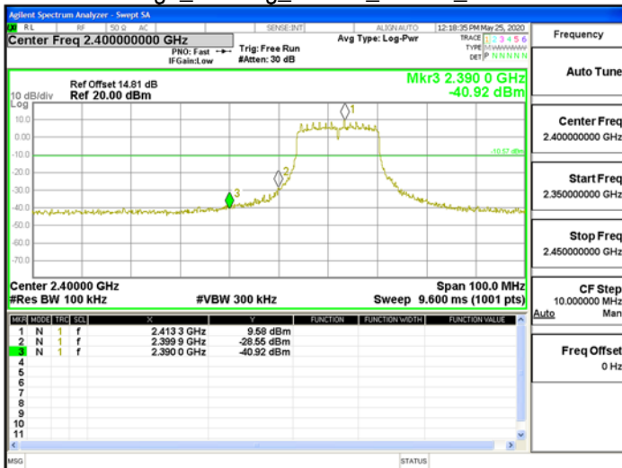
Band Edge_802.11g_20MHz_Chain0_2412MHz
