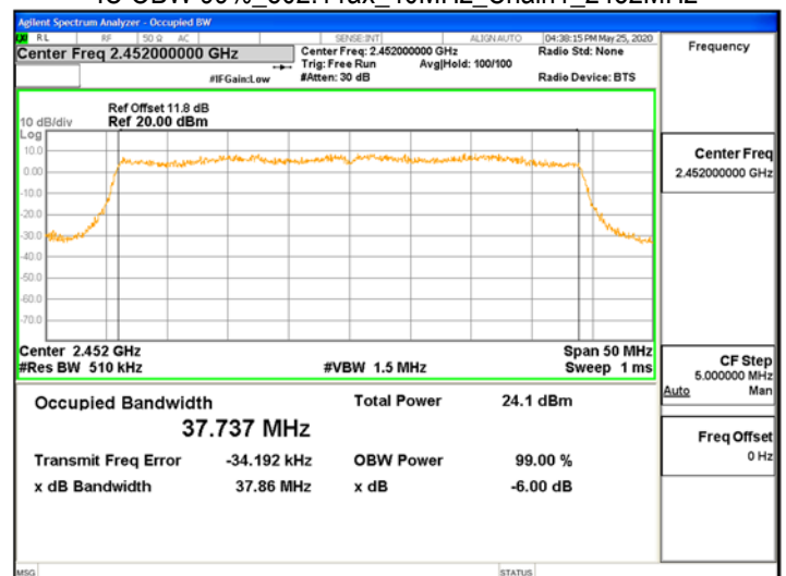
IC OBW 99% 802.11ax 40MHz Chain1 2452MHz
