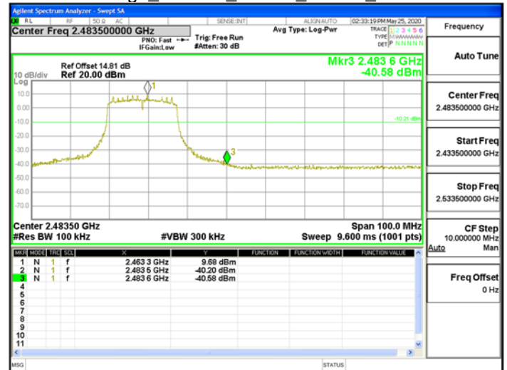
Band Edge_802.11n_20MHz_Chain0_2462MHz
