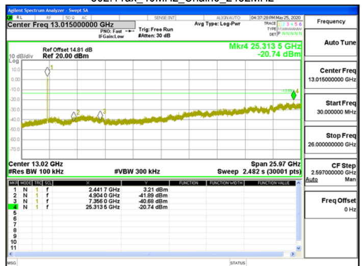
802.11ax_40MHz_Chain0_2452MHz
