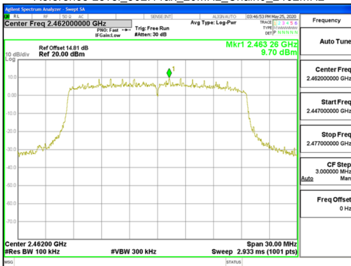
Reference Level 802.11ax 20MHz Chain0 2462MHz
