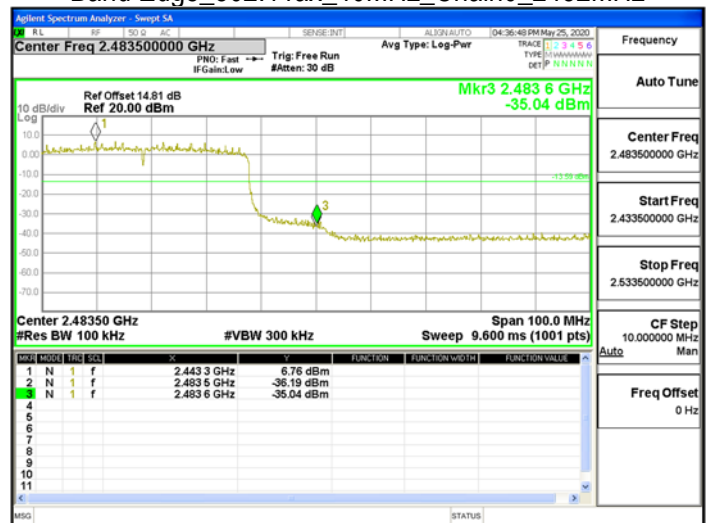
Band Edge 802.11ax 40MHz Chain0 2452MHz
