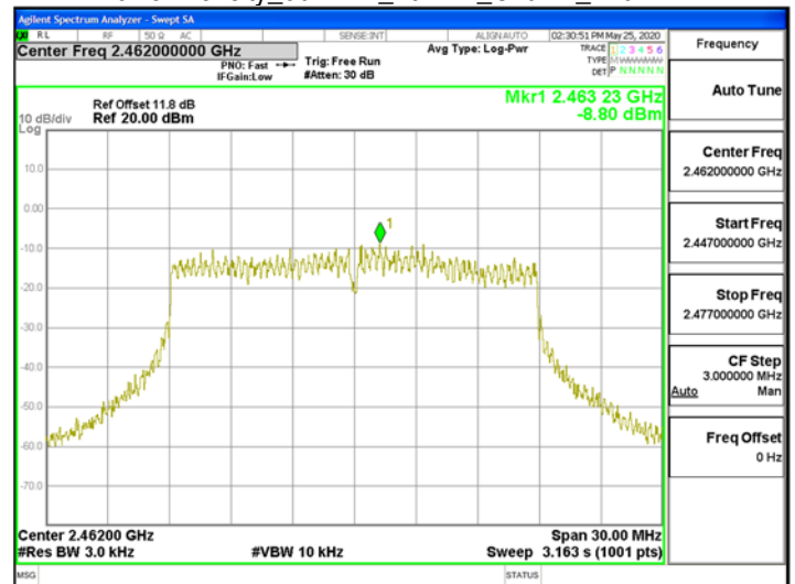
Power Density_802.11n_20MHz_Chain1_2462MHz
