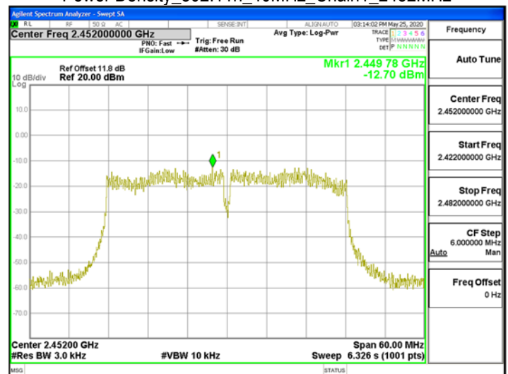
Power Density_802.11n_40MHz_Chain1_2452MHz
