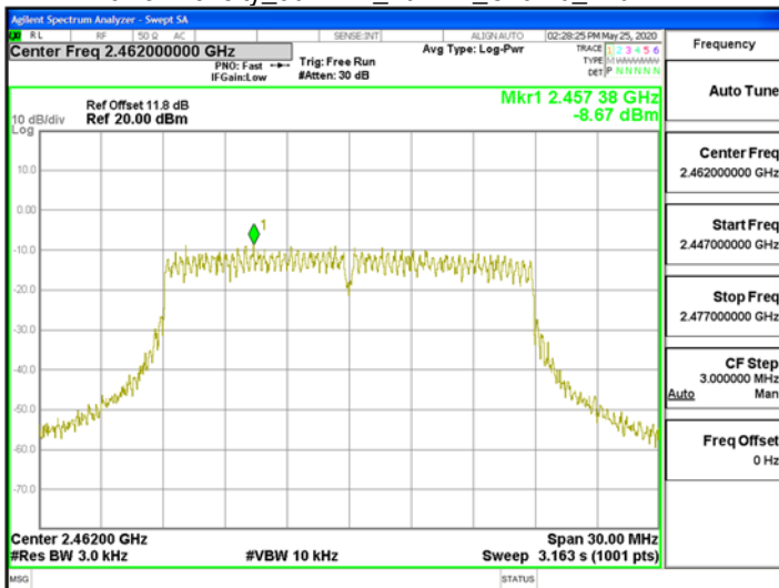
Power Density_802.11n_20MHz_Chain0_2462MHz
