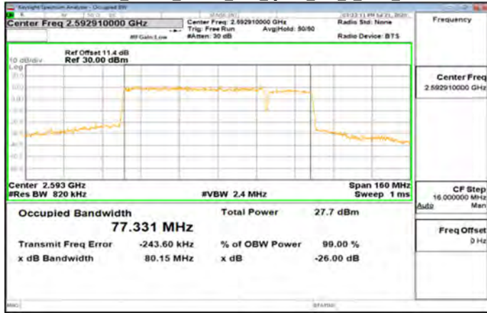
Band41_20MHz_60MHz_DFT_QPSK_162_0_Main_High
