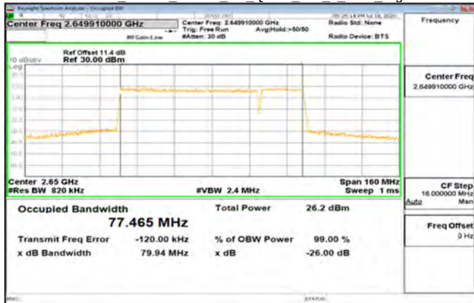
Band41_20MHz_60MHz_CP_QPSK_162_0_Main_High
