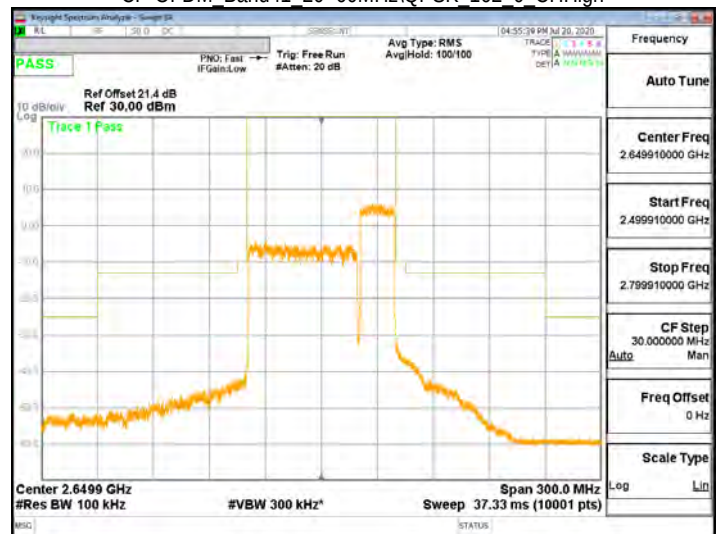
CP-OFDM Band41 20+60MHz/QPSK 162 0 CHHigh
