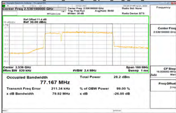
Band41_20MHz_60MHz_DFT_QPSK_162_0_Main_Low
