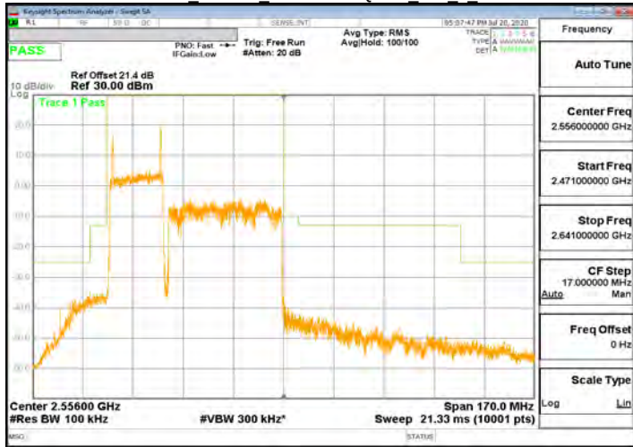
CP-OFDM Band41 20+40MHz/QPSK 106 0 CHHigh
