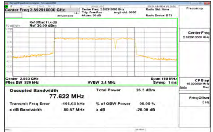
Band41_20MHz_60MHz_CP_16QAM_162_0_Main_Mid
