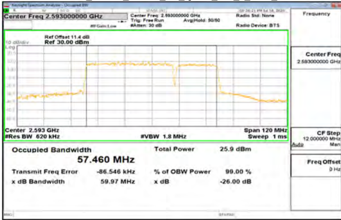
Band41_20MHz_40MHz_CP_QPSK_106_0_Main_High
