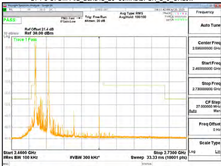
DFT-s-OFDM Pi/2 Band41 20+80MHz\BPSK 1 0 CHLow
