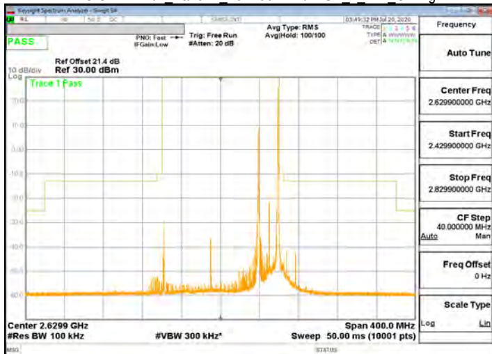
DFT-s-OFDM Pi/2 Band41 20+100MHz\BPSK 1 272 CHHigh
