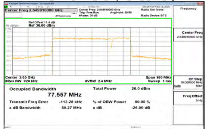
Band41_20MHz_60MHz_CP_16QAM_162_0_Main_High
