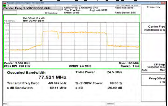
Band41_20MHz_60MHz_CP_256QAM_162_0_Main_Mid
