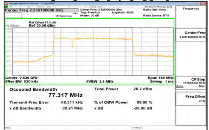
Band41_20MHz_60MHz_CP_16QAM_162_0_Main_Low
