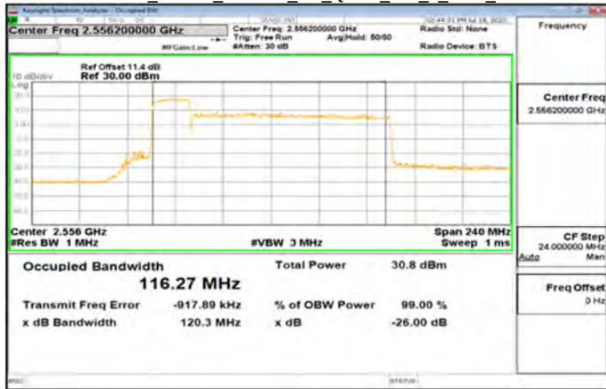
Band41_20MHz_100MHz_CP_QPSK_273_0_Main_Mid
