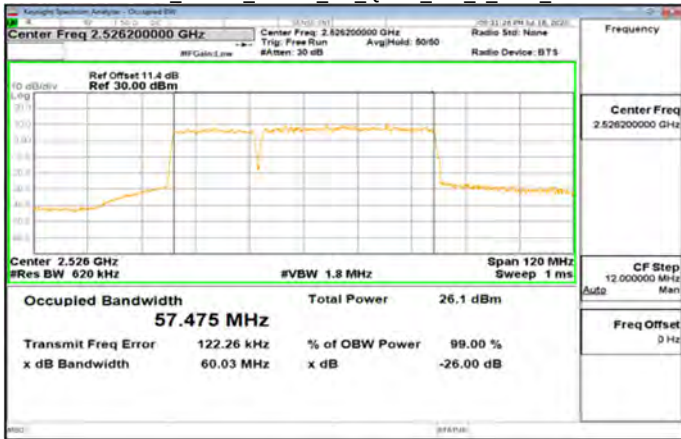
Band41_20MHz_40MHz_CP_QPSK_106_0_Main_Low
