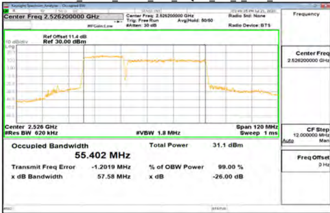
Band41_20MHz_40MHz_DFT_16QAM_100_0_Main_Mid
