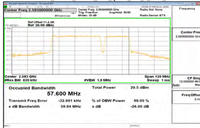
Band41 20MHz 40MHz DFT QPSK 100 0 Main Mid
