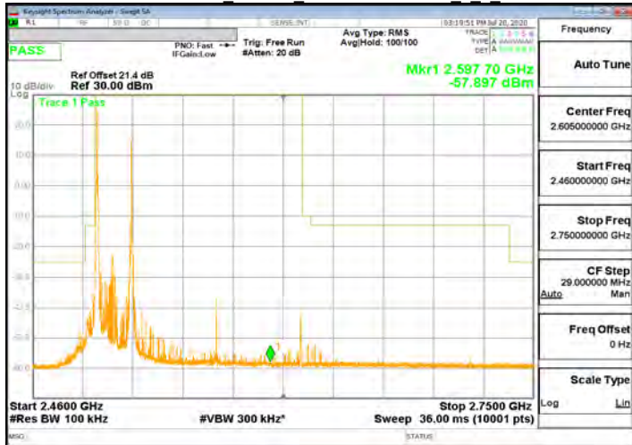
DFT-s-OFDM Pi/2 Band41 20+100MHz\BPSK 1 0 CHLow
