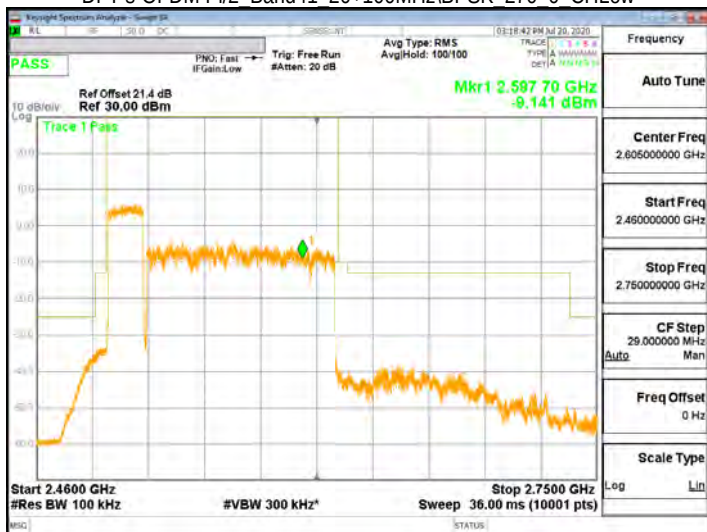
DFT-s-OFDM Pi/2 Band41 20+100MHz\BPSK 270 0 CHLow
