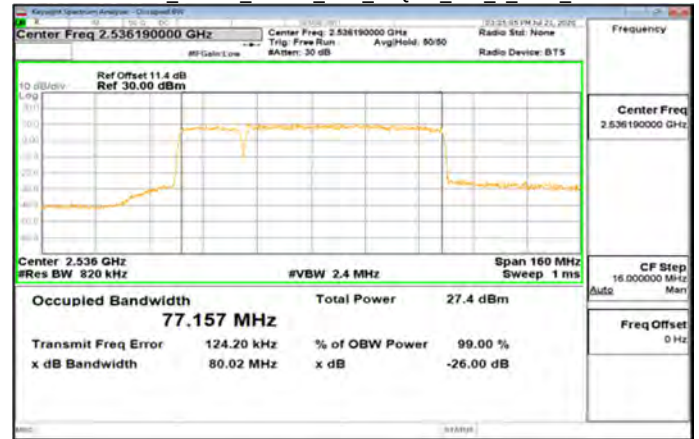
Band41_20MHz_60MHz_DFT_16QAM_162_0_Main_Low
