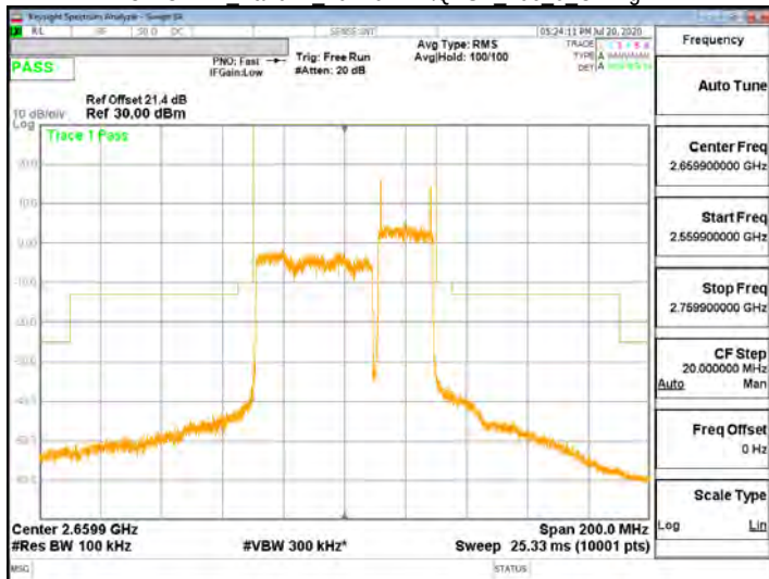
CP-OFDM Band41 20+60MHz/QPSK 1 0 CHLow
