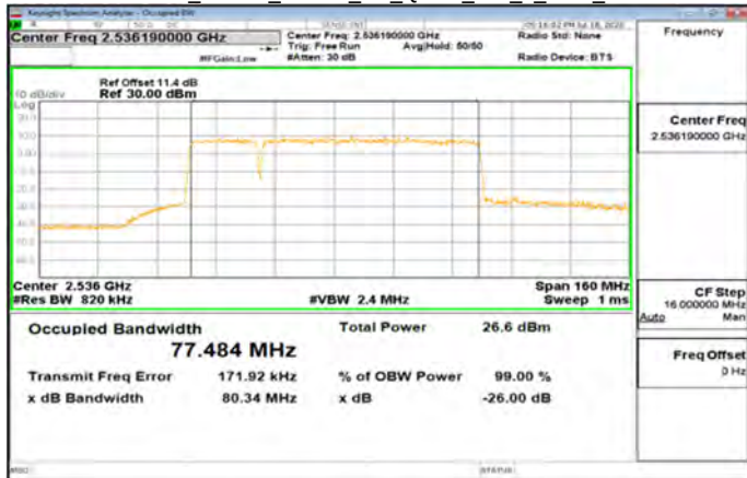
Band41_20MHz_60MHz_CP_QPSK_162_0_Main_Low
