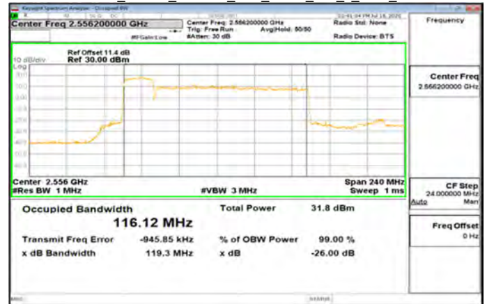
Band41_20MHz_100MHz_DFT_BPSK_270_0_Main_Low
