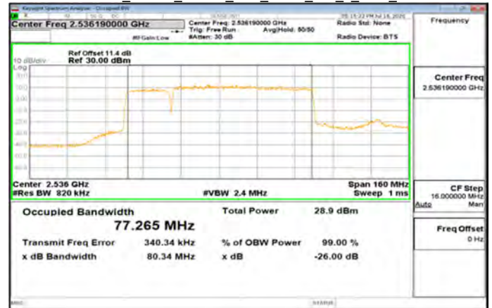
Band41_20MHz_60MHz_DFT_BPSK_162_0_Main_Mid
