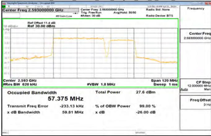
Band41_20MHz_40MHz_DFT_16QAM_100_0_Main_High
