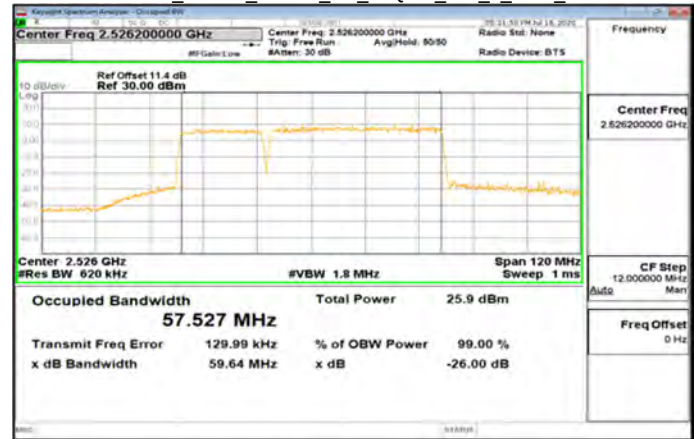
Band41_20MHz_40MHz_CP_16QAM_106_0_Main_Low
