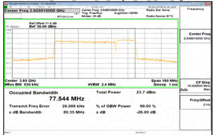
Band41_20MHz_60MHz_CP_256QAM_162_0_Main_High
