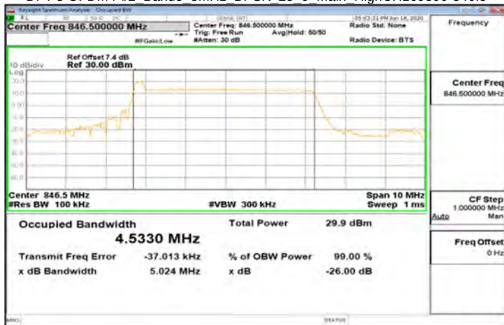
DFT-s-OFDM Pi/2_Band5_5MHz_BPSK_25_0_Main_HighCH169300-846.5
