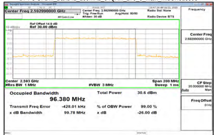
DFT-s-OFDM_Band41_100MHz_64QAM_270_0_Main_MidCH518598
