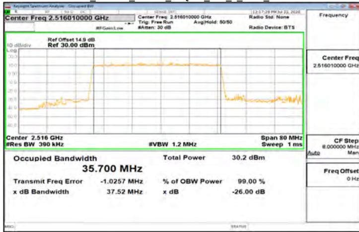
DFT-s-OFDM_Band41_40MHz_64QAM_100_0_Main_LowCH503202
