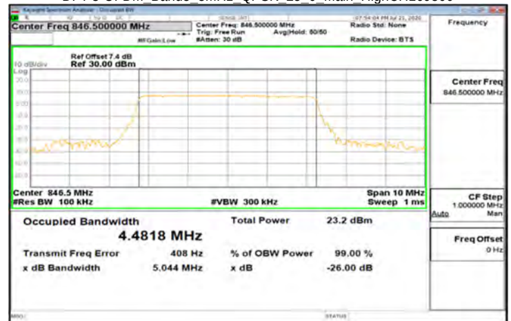
DFT-s-OFDM_Band5_5MHz_QPSK_25_0_Main_HighCH169300
