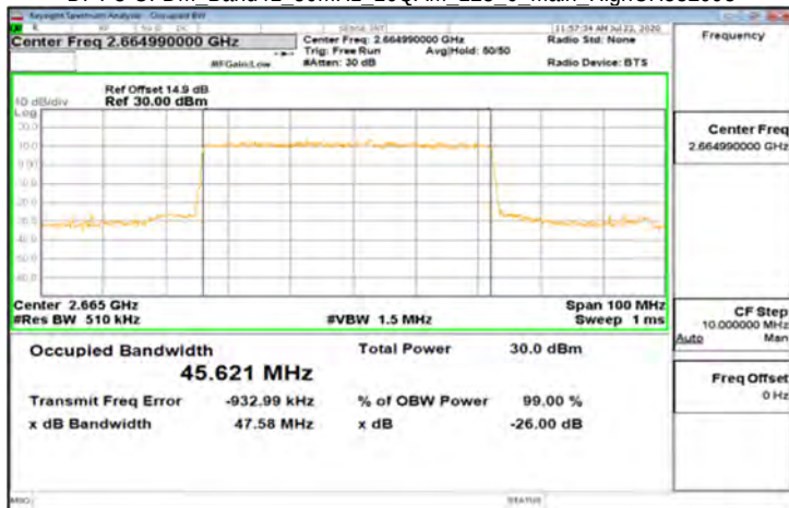
DFT-s-OFDM_Band41_50MHz_16QAM_128_0_Main_HighCH532998
