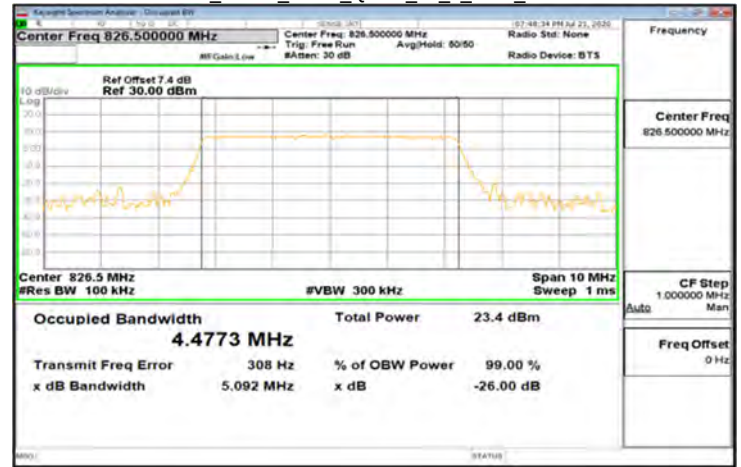
DFT-s-OFDM_Band5_5MHz_QPSK_25_0_Main_LowCH165300
