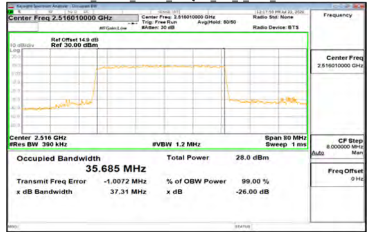
DFT-s-OFDM_Band41_40MHz_256QAM_100_0_Main_LowCH503202
