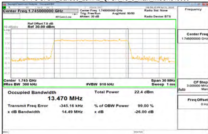
DFT-s-OFDM_Band66_15MHz_QPSK_75_0_Main_MidCH349000
