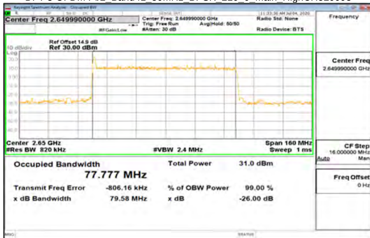
DFT-s-OFDM Pi/2_Band41_80MHz_BPSK_216_0_Main_HighCH529998
