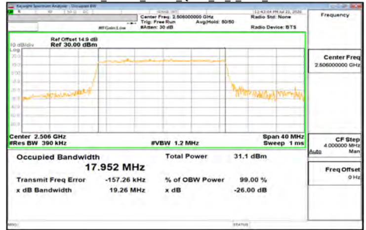
DFT-s-OFDM_Band41_20MHz_QPSK_50_0_Main_LowCH39750
