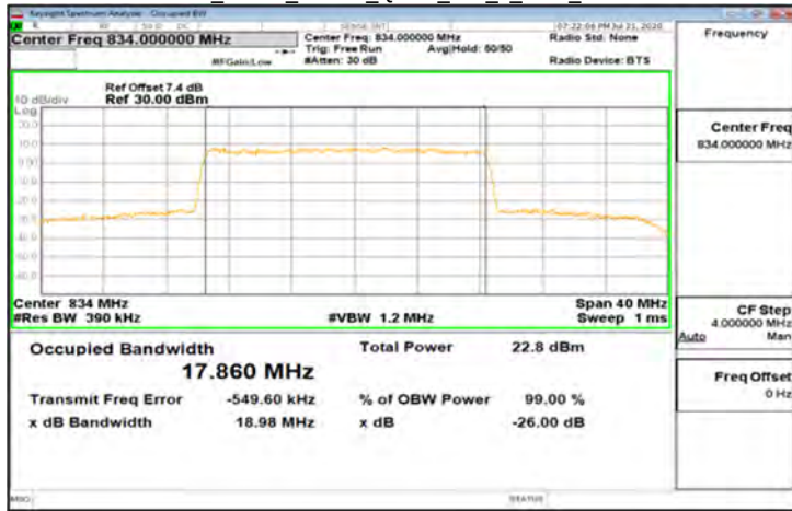
DFT-s-OFDM_Band5_20MHz_QPSK_100_0_Main_MidCH167300
