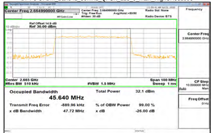
DFT-s-OFDM_Band41_50MHz_QPSK_128_0_Main_HighCH532998
