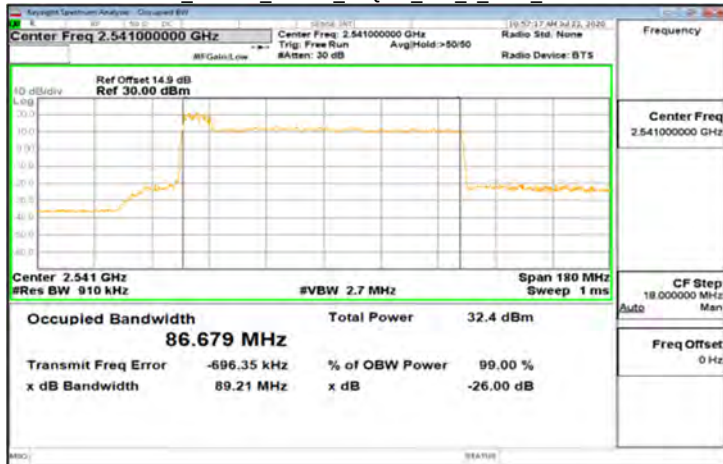
DFT-s-OFDM_Band41_90MHz_64QAM_243_0_Main_LowCH508200
