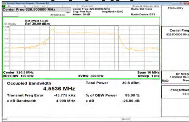
DFT-s-OFDM Pi/2_Band5_5MHz_BPSK_25_0_Main_LowCH165300-826.5
