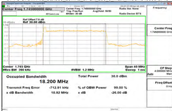
DFT-s-OFDM Pi/2_Band66_20MHz_BPSK_100_0_Main_MidCH349000-1745
