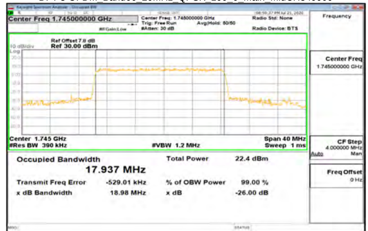
DFT-s-OFDM_Band66_20MHz_QPSK_100_0_Main_MidCH349000
