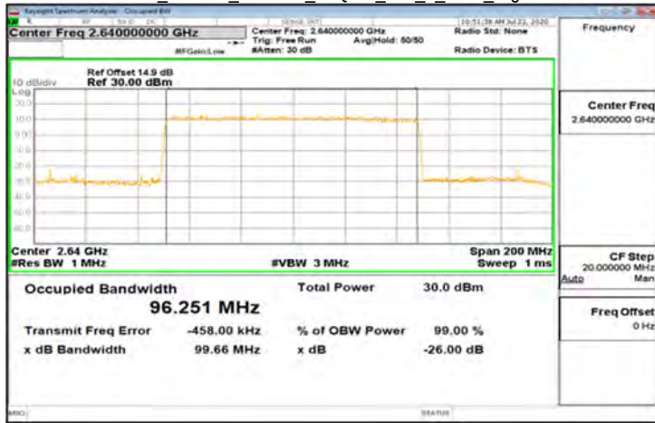
DFT-s-OFDM_Band41_100MHz_64QAM_270_0_Main_HighCH528000
