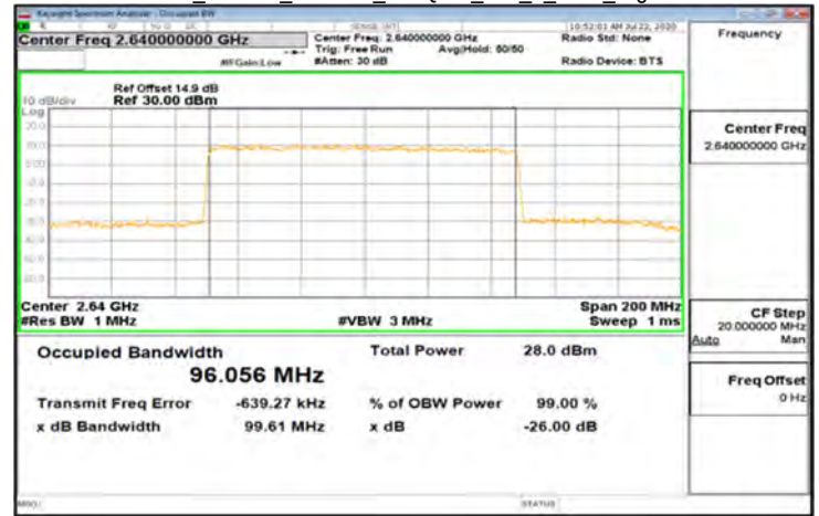
DFT-s-OFDM_Band41_100MHz_256QAM_270_0_Main_HighCH528000
