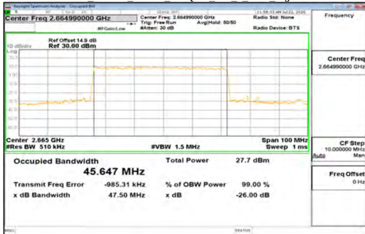
DFT-s-OFDM_Band41_50MHz_256QAM_128_0_Main_HighCH532998
