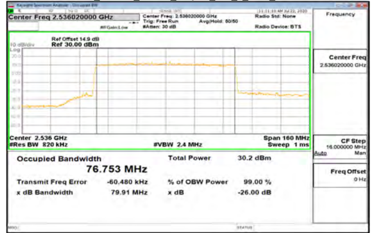
DFT-s-OFDM_Band41_80MHz_64QAM_216_0_Main_LowCH507204
