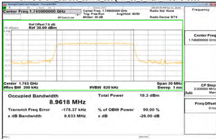
DFT-s-OFDM_Band66_10MHz_256QAM_50_0_Main_MidCH349000
