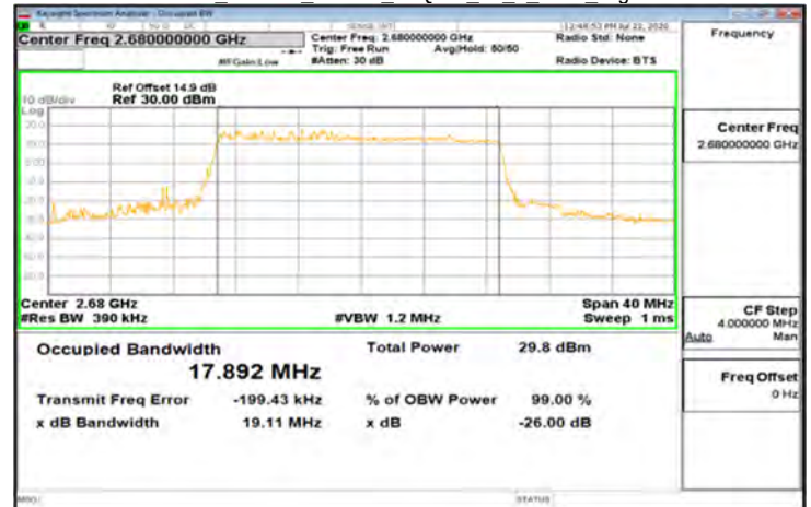
DFT-s-OFDM_Band41_20MHz_64QAM_50_0_Main_HighCH41490
