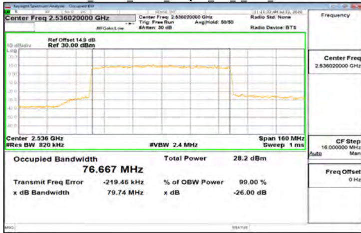
DFT-s-OFDM_Band41_80MHz_256QAM_216_0_Main_LowCH507204
