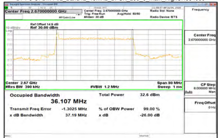
DFT-s-OFDM Pi/2_Band41_40MHz_BPSK_100_0_Main_HighCH534000
