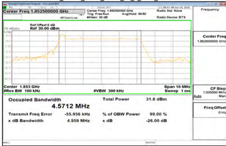
DFT-s-OFDM Pi/2_Band2_5MHz_BPSK_25_0_Main_LowCH370500-1852.5
