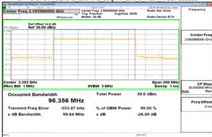
DFT-s-OFDM_Band41_100MHz_16QAM_270_0_Main_MidCH518598
