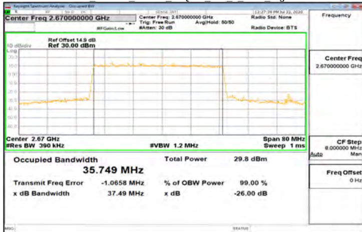
DFT-s-OFDM_Band41_40MHz_64QAM_100_0_Main_HighCH534000
