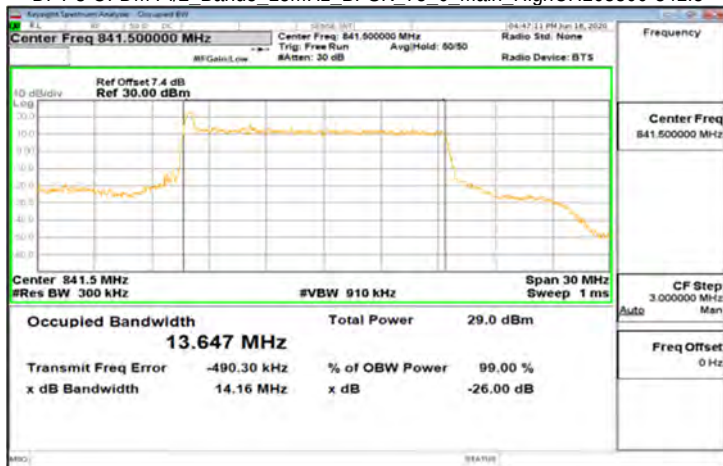
DFT-s-OFDM Pi/2_Band5_15MHz_BPSK_75_0_Main_HighCH168300-841.5
