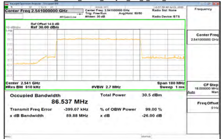
DFT-s-OFDM_Band41_90MHz_256QAM_243_0_Main_LowCH508200
