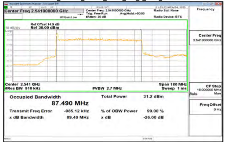
DFT-s-OFDM Pi/2_Band41_90MHz_BPSK_243_0_Main_LowCH508200-2541
