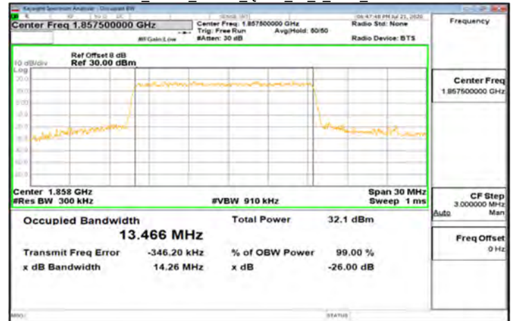
DFT-s-OFDM_Band2_15MHz_QPSK_75_0_Main_LowCH371500
