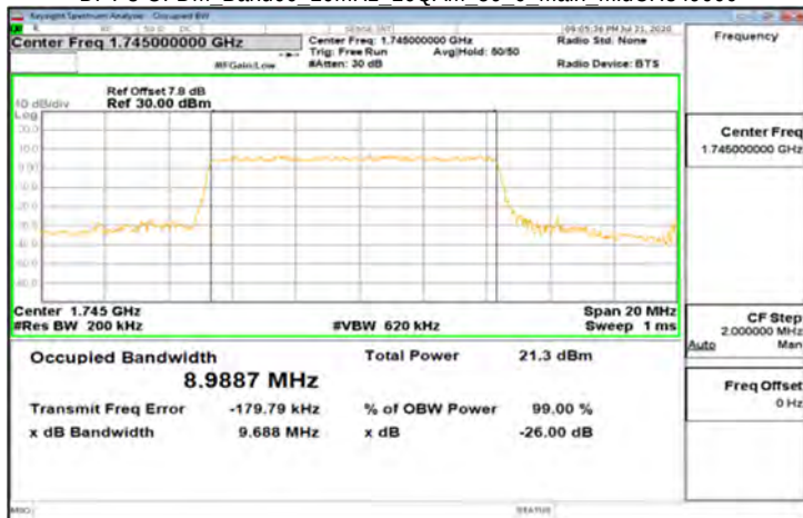
DFT-s-OFDM_Band66_10MHz_16QAM_50_0_Main_MidCH349000
