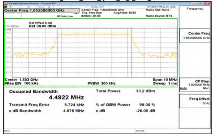
DFT-s-OFDM_Band2_5MHz_QPSK_25_0_Main_LowCH370500
