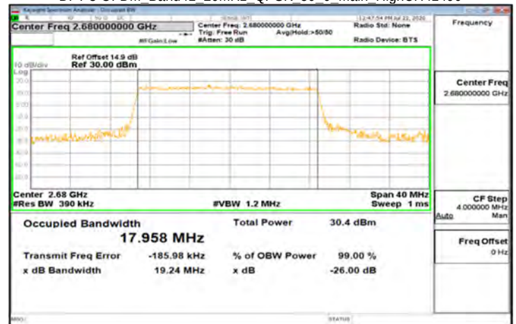
DFT-s-OFDM_Band41_20MHz_QPSK_50_0_Main_HighCH41490
