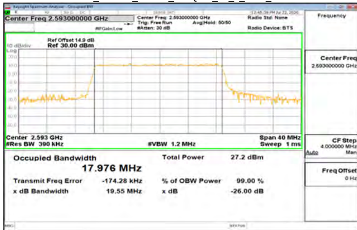
DFT-s-OFDM_Band41_20MHz_256QAM_50_0_Main_HighCH41490
