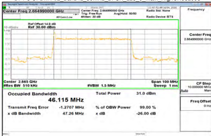
DFT-s-OFDM Pi/2_Band41_50MHz_BPSK_128_0_Main_HighCH532998
