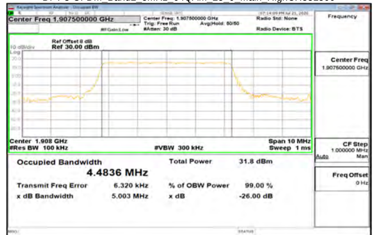
DFT-s-OFDM_Band2_5MHz_64QAM_25_0_Main_HighCH381500
