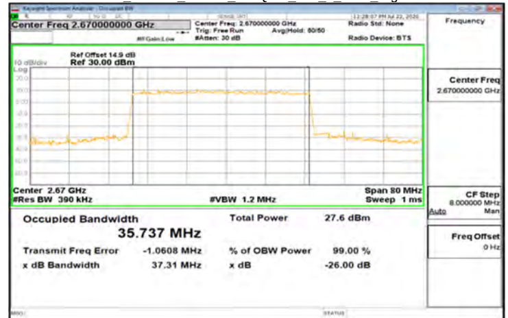
DFT-s-OFDM_Band41_40MHz_256QAM_100_0_Main_HighCH534000
