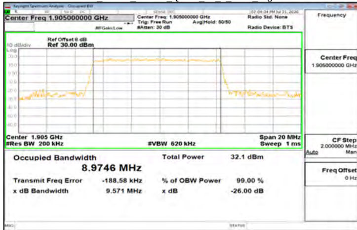
DFT-s-OFDM_Band2_10MHz_QPSK_50_0_Main_HighCH381000
