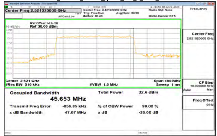
DFT-s-OFDM_Band41_50MHz_QPSK_128_0_Main_LowCH504204
