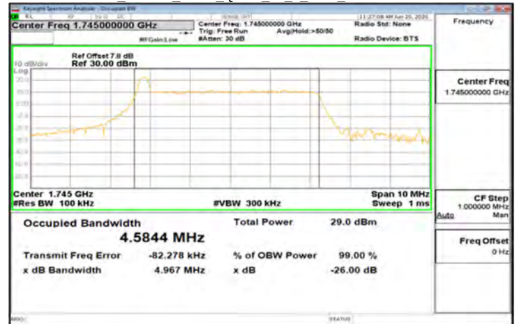
CP-OFDM_Band66_5MHz_QPSK_25_0_Main_MidCH349000-1745
