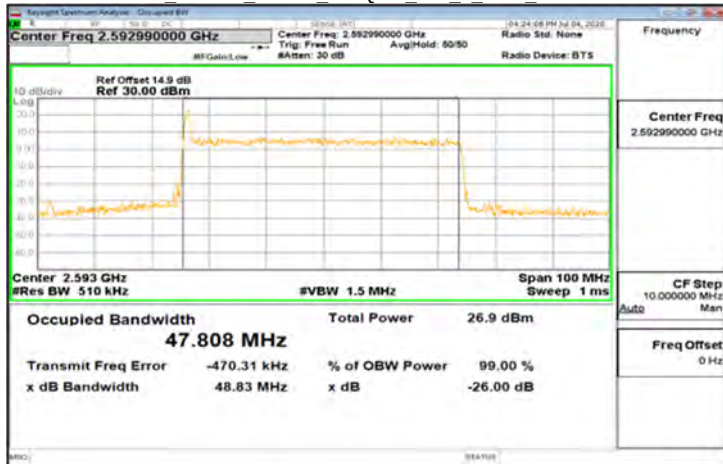
CP-OFDM_Band41_50MHz_256QAM_133_0_Main_MidCH518598
