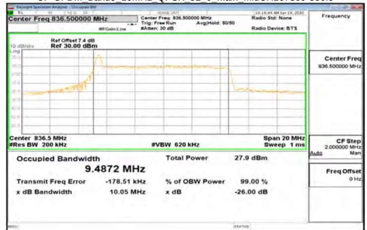
CP-OFDM Band5_10MHz_QPSK_52_0_Main_MidCH167300-836.5
