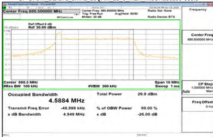
CP-OFDM_Band71_5MHz_16QAM_25_0_Main_MidCH136100-680.5
