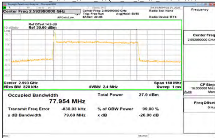
CP-OFDM_Band41_80MHz_256QAM_217_0_Main_MidCH518598
