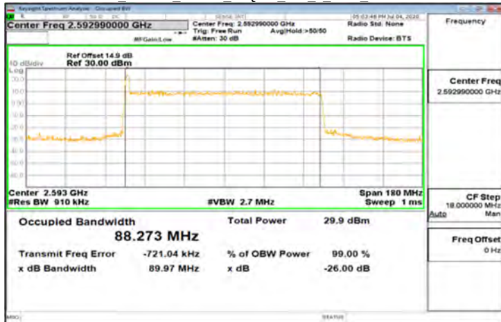
CP-OFDM_Band41_90MHz_16QAM_245_0_Main_MidCH518598
