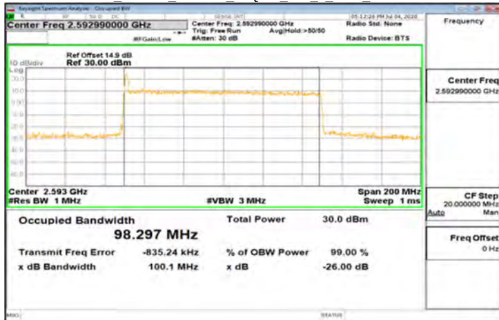
CP-OFDM_Band41_100MHz_16QAM_273_0_Main_MidCH518598
