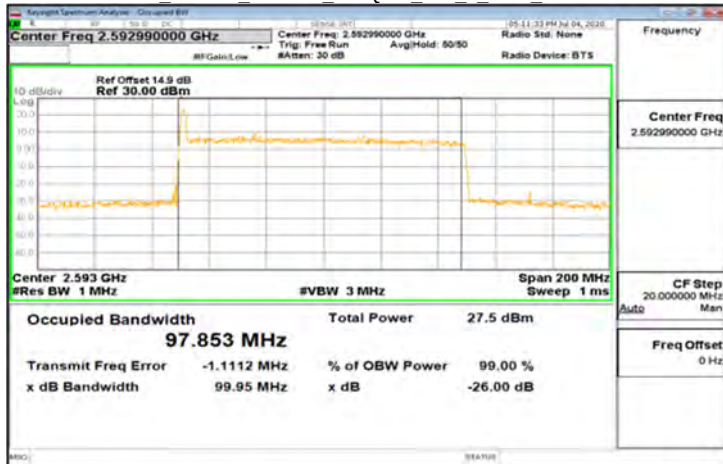
CP-OFDM_Band41_100MHz_256QAM_273_0_Main_MidCH518598
