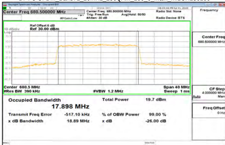
DFT-s-OFDM_Band71_20MHz_256QAM_100_0_Main_MidCH136100
