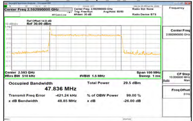
CP-OFDM_Band41_50MHz_64QAM_133_0_Main_MidCH518598
