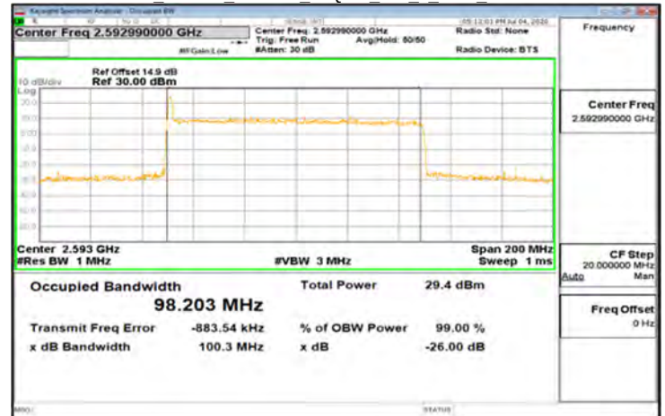
CP-OFDM_Band41_100MHz_64QAM_273_0_Main_MidCH518598
