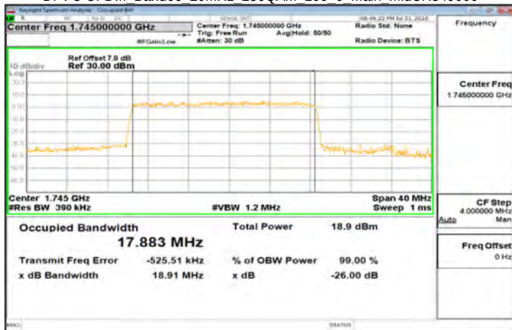
DFT-s-OFDM_Band66_20MHz_256QAM_100_0_Main_MidCH349000
