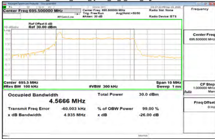
CP-OFDM_Band71_5MHz_QPSK_25_0_Main_HighCH139100-695.5
