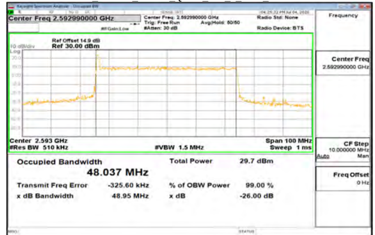
CP-OFDM_Band41_50MHz_QPSK_133_0_Main_MidCH518598
