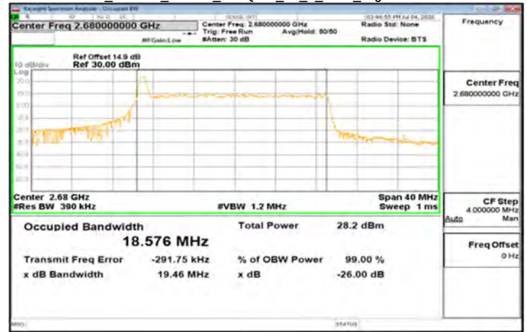
CP-OFDM Band41_20MHz_256QAM_51_0_Main_HighCH535998-2680
