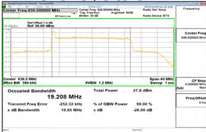
CP-OFDM_Band5_20MHz_16QAM_106_0_Main_MidCH167300-836.5
