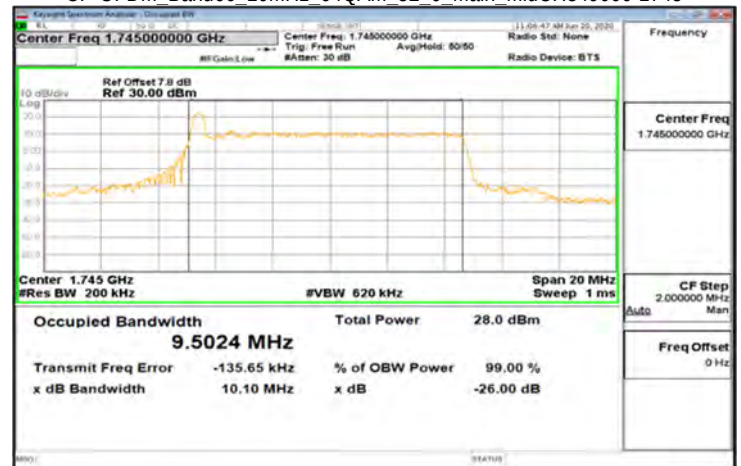
CP-OFDM_Band66_10MHz_64QAM_52_0_Main_MidCH349000-1745
