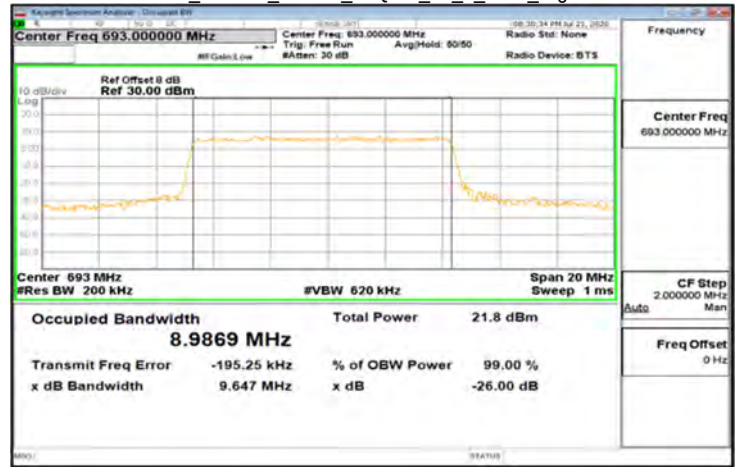
DFT-s-OFDM_Band71_10MHz_16QAM_50_0_Main_HighCH138600
