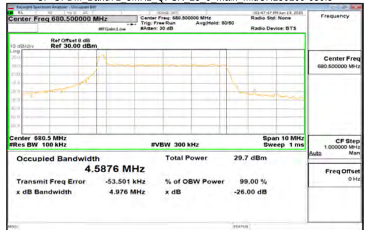
CP-OFDM_Band71_5MHz_QPSK_25_0_Main_MidCH136100-680.5
