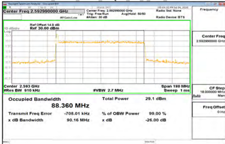
CP-OFDM_Band41_90MHz_256QAM_245_0_Main_MidCH518598
