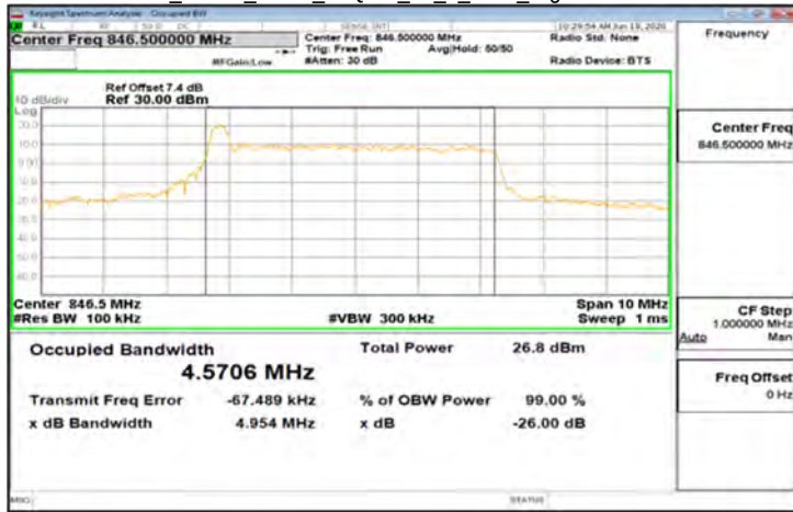
CP-OFDM Band5_5MHz_64QAM_25_0_Main_HighCH169300-846.5
