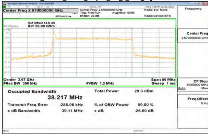
CP-OFDM_Band41_40MHz_64QAM_106_0_Main_HighCH534000-2670
