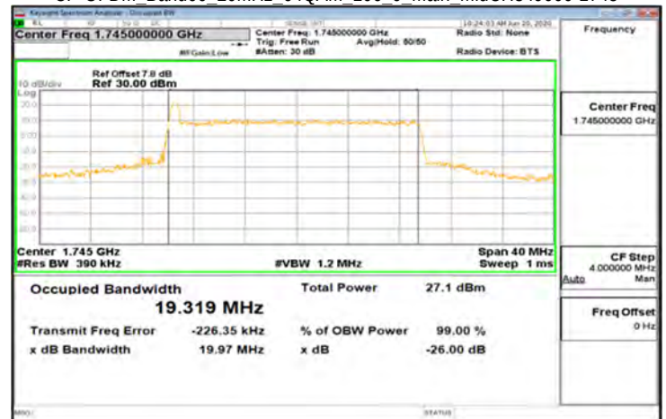
CP-OFDM Band66_20MHz_64QAM_106_0_Main_MidCH349000-1745
