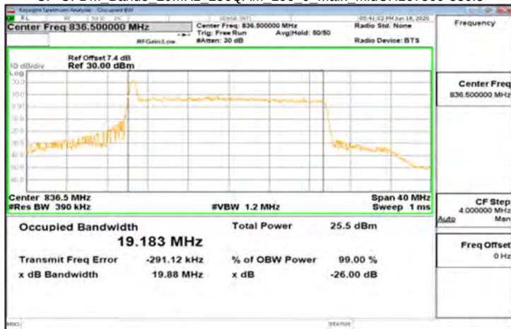
CP-OFDM Band5 20MHz 256QAM 106 0 Main_MidCH167300-836.5
