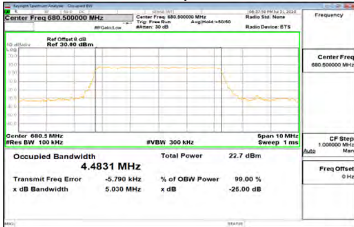
DFT-s-OFDM_Band71_5MHz_64QAM_25_0_Main_MidCH136100
