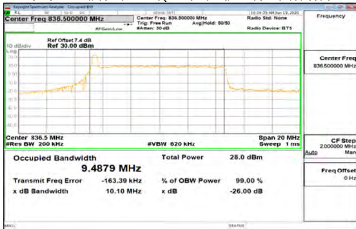
CP-OFDM_Band5_10MHz_16QAM_52_0_Main_MidCH167300-836.5
