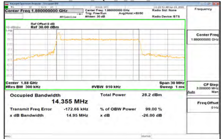
CP-OFDM_Band2_15MHz_64QAM_79_0_Main_MidCH376000-1880
