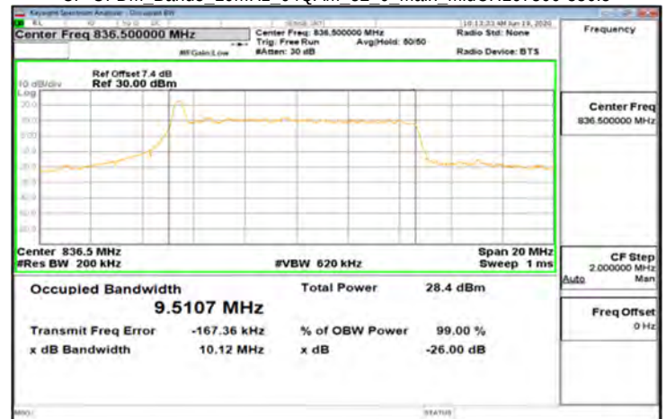
CP-OFDM_Band5_10MHz_64QAM_52_0_Main_MidCH167300-836.5
