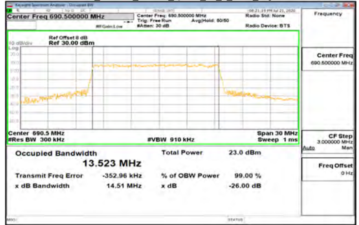
DFT-s-OFDM_Band71_15MHz_QPSK_75_0_Main_HighCH138100
