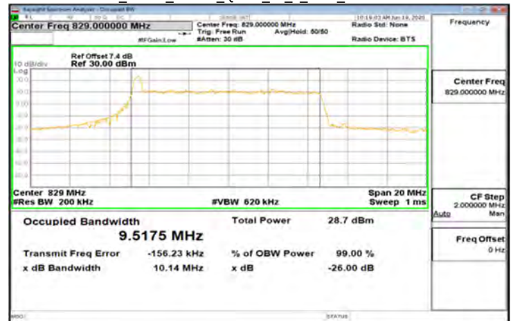
CP-OFDM Band5_10MHz_QPSK_52_0_Main_LowCH165800-829
