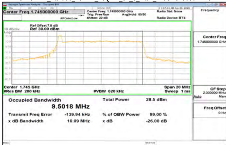
CP-OFDM_Band66_10MHz_16QAM_52_0_Main_MidCH349000-1745
