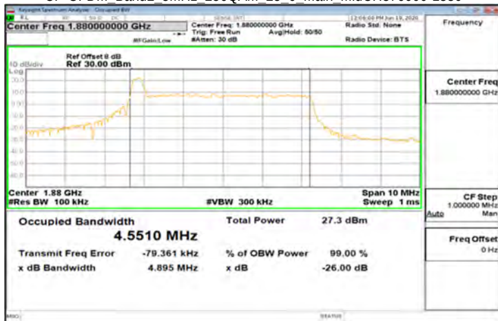
CP-OFDM_Band2_5MHz_256QAM_25_0_Main_MidCH376000-1880
