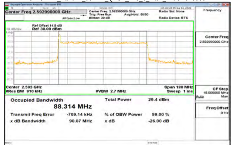
CP-OFDM_Band41_90MHz_QPSK_245_0_Main_MidCH518598
