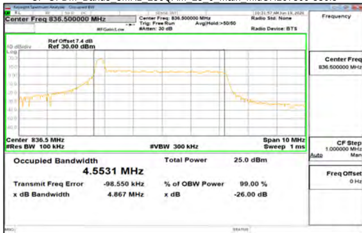
CP-OFDM Band5_5MHz_256QAM_25_0_Main_MidCH167300-836.5
