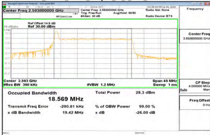
CP-OFDM Band41_20MHz_256QAM_51_0_Main_MidCH518598-2593
