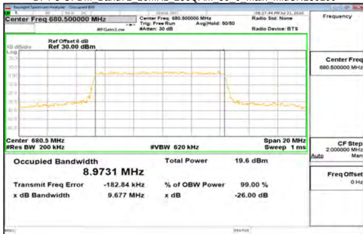
DFT-s-OFDM_Band71_10MHz_256QAM_50_0_Main_MidCH136100
