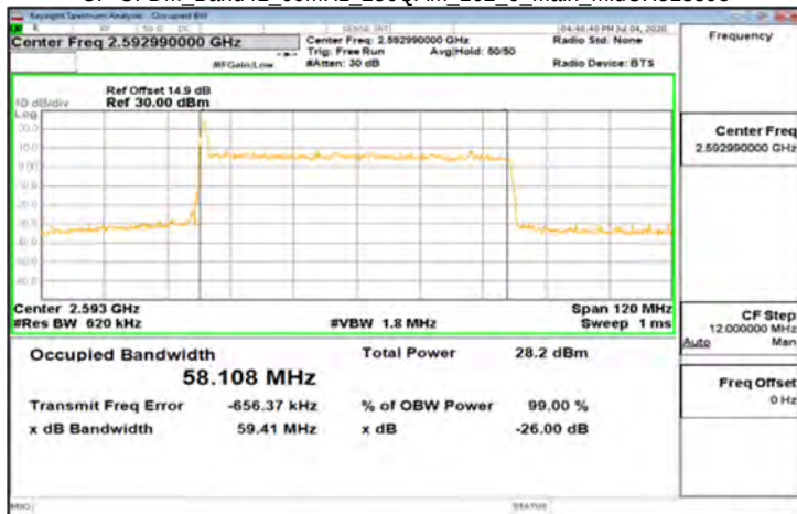
CP-OFDM_Band41_60MHz_256QAM_162_0_Main_MidCH518598
