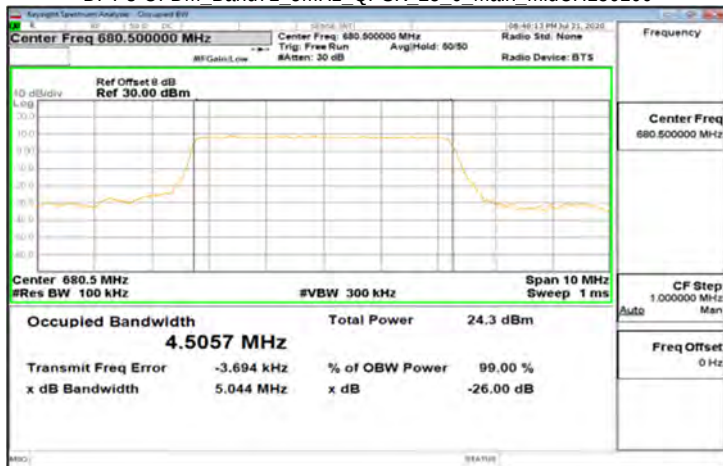
DFT-s-OFDM_Band71_5MHz_QPSK_25_0_Main_MidCH136100
