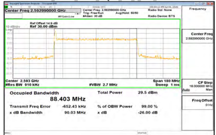
CP-OFDM_Band41_90MHz_64QAM_245_0_Main_MidCH518598
