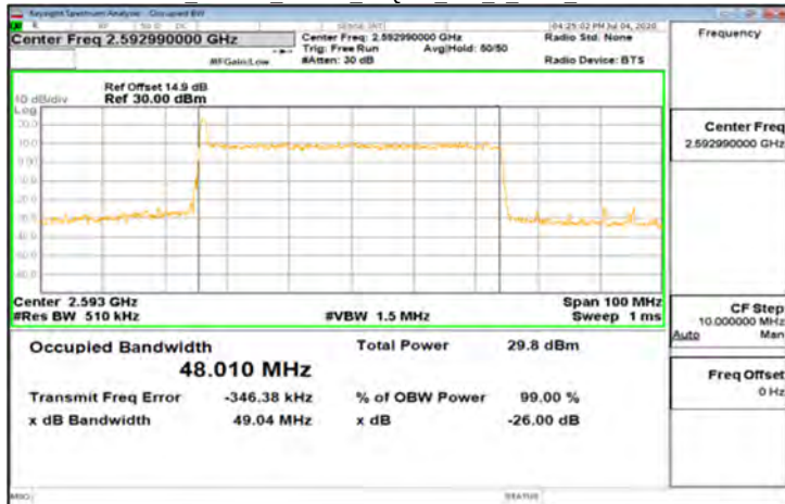
CP-OFDM_Band41_50MHz_16QAM_133_0_Main_MidCH518598
