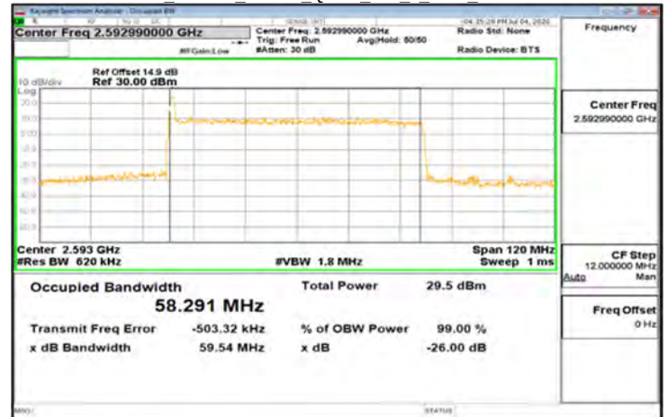
CP-OFDM_Band41_60MHz_QPSK_162_0_Main_MidCH518598
