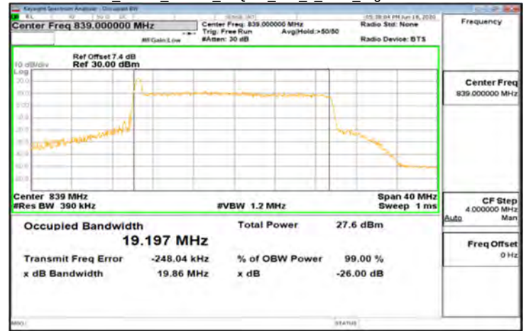
CP-OFDM_Band5_20MHz_16QAM_106_0_Main_HighCH167800-839
