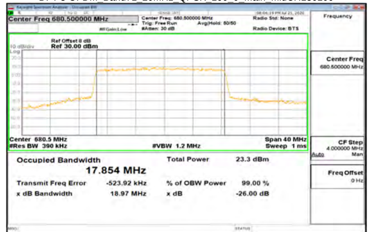
DFT-s-OFDM_Band71_20MHz_QPSK_100_0_Main_MidCH136100
