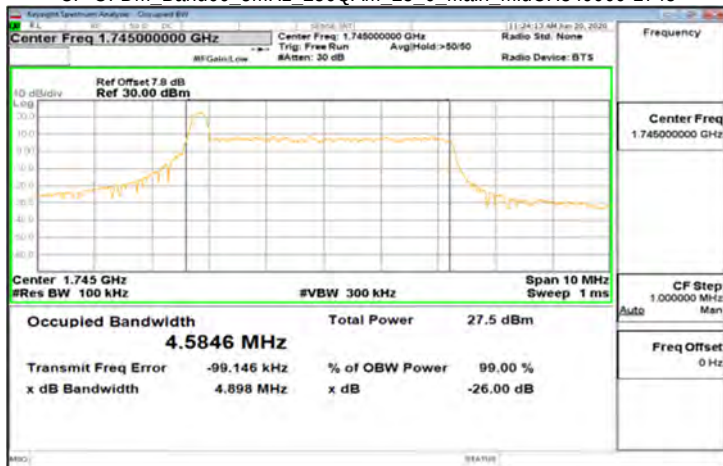
CP-OFDM_Band66_5MHz_256QAM_25_0_Main_MidCH349000-1745
