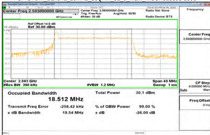
CP-OFDM_Band41_20MHz_16QAM_51_0_Main_MidCH518598-2593
