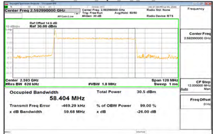
CP-OFDM_Band41_60MHz_64QAM_162_0_Main_MidCH518598
