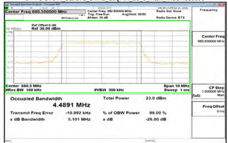
DFT-s-OFDM_Band71_5MHz_16QAM_25_0_Main_MidCH136100
