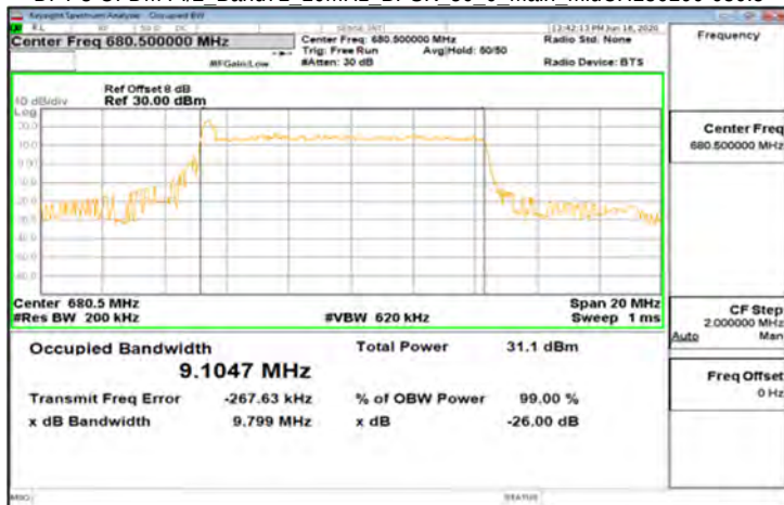
DFT-s-OFDM Pi/2_Band71_10MHz_BPSK_50_0_Main_MidCH136100-680.5
