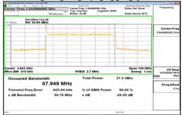
CP-OFDM_Band41_90MHz_256QAM_245_0_Main_HighCH528996
