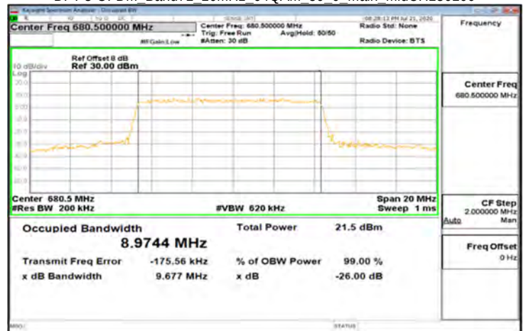
DFT-s-OFDM_Band71_10MHz_64QAM_50_0_Main_MidCH136100
