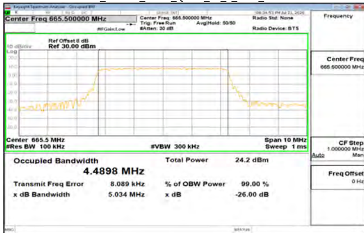
DFT-s-OFDM_Band71_5MHz_QPSK_25_0_Main_LowCH133100
