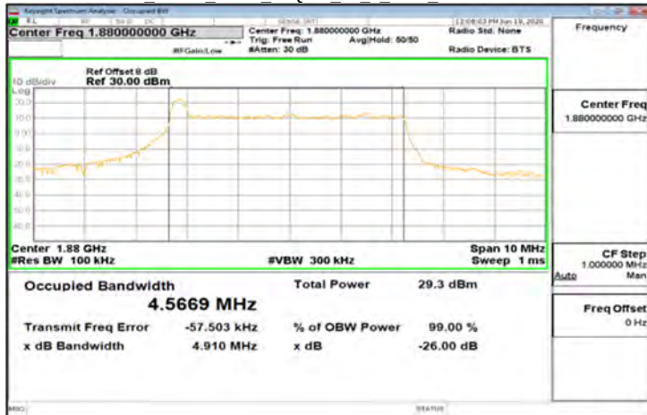
CP-OFDM_Band2_5MHz_16QAM_25_0_Main_MidCH376000-1880
