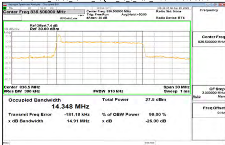
CP-OFDM_Band5_15MHz_16QAM_79_0_Main_MidCH167300-836.5
