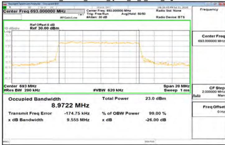
DFT-s-OFDM_Band71_10MHz_QPSK_50_0_Main_HighCH138600
