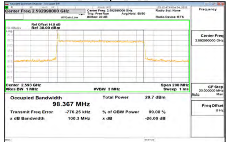
CP-OFDM_Band41_100MHz_QPSK_273_0_Main_MidCH518598
