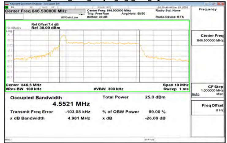
CP-OFDM Band5_5MHz_256QAM_25_0_Main_HighCH169300-846.5
