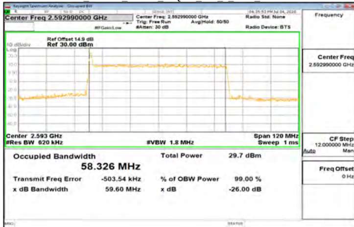
CP-OFDM_Band41_60MHz_16QAM_162_0_Main_MidCH518598
