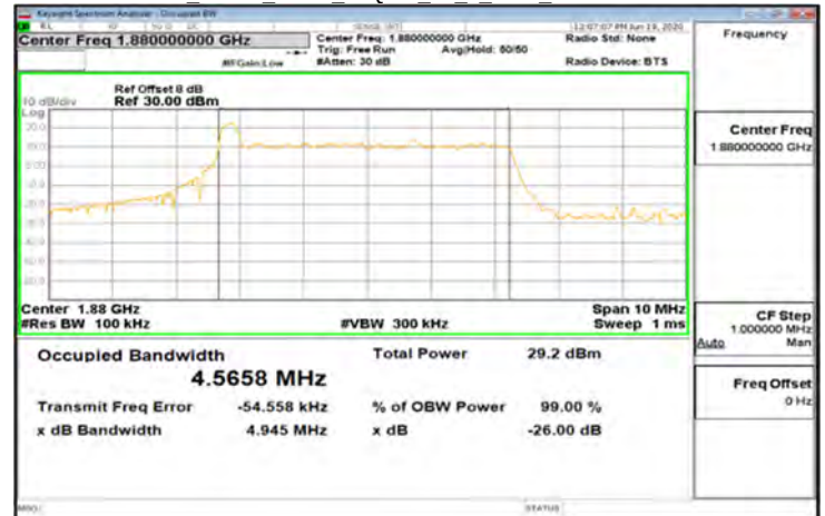
CP-OFDM_Band2_5MHz_64QAM_25_0_Main_MidCH376000-1880
