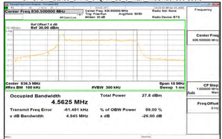
CP-OFDM_Band5_5MHz_64QAM_25_0_Main_MidCH167300-836.5
