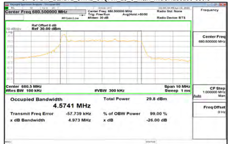
CP-OFDM_Band71_5MHz_64QAM_25_0_Main_MidCH136100-680.5
