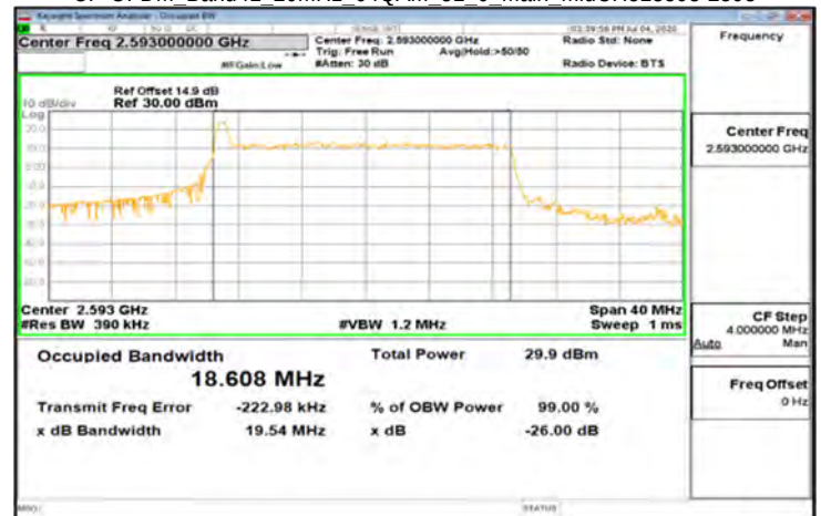
CP-OFDM_Band41_20MHz_64QAM_51_0_Main_MidCH518598-2593
