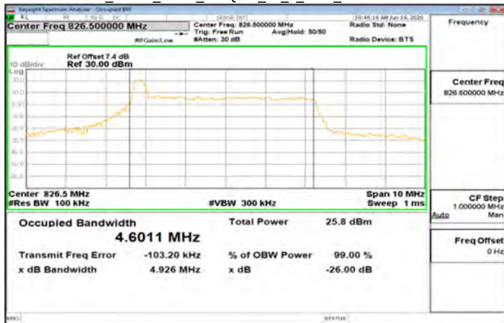
CP-OFDM Band5_5MHz_256QAM_25_0_Main_LowCH165300-826.5
