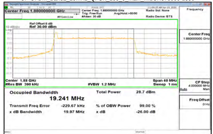
CP-OFDM_Band2_20MHz_QPSK_106_0_Main_MidCH376000-1880
