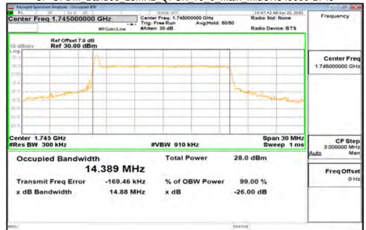
CP-OFDM Band66_15MHz_QPSK_79_0_Main_MidCH349000-1745
