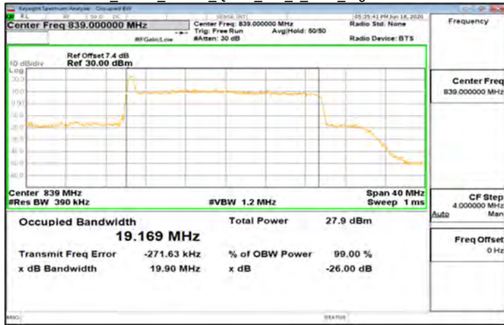
CP-OFDM_Band5_20MHz_QPSK_106_0_Main_HighCH167800-839
