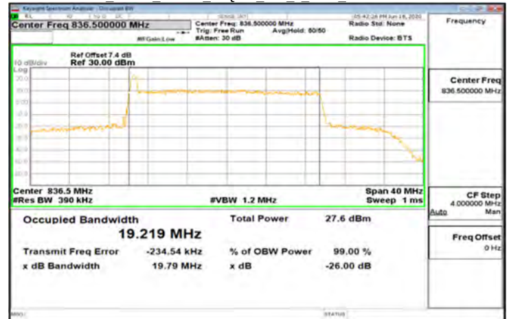
CP-OFDM_Band5_20MHz_64QAM_106_0_Main_MidCH167300-836.5
