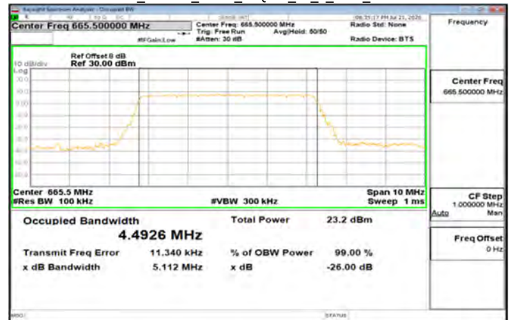
DFT-s-OFDM_Band71_5MHz_16QAM_25_0_Main_LowCH133100
