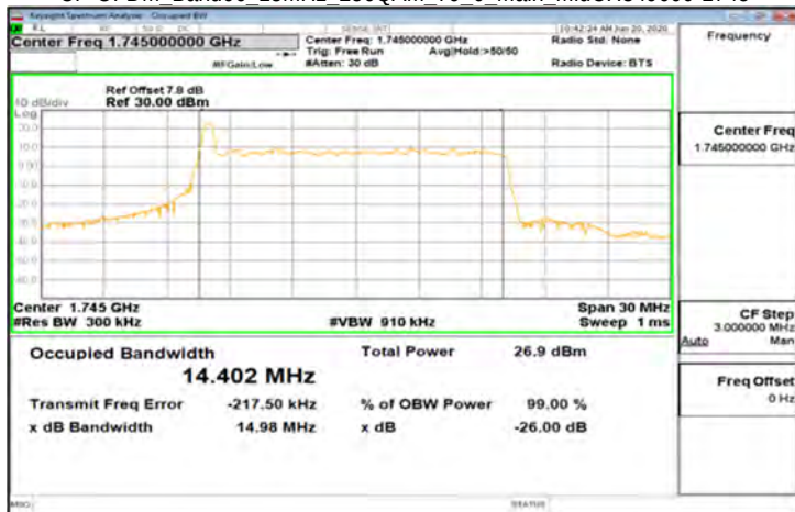
CP-OFDM_Band66_15MHz_256QAM_79_0_Main_MidCH349000-1745
