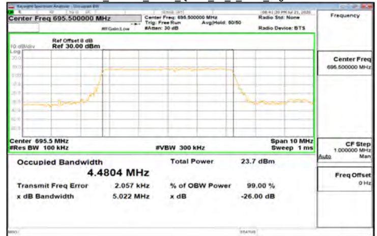
DFT-s-OFDM_Band71_5MHz_QPSK_25_0_Main_HighCH139100
