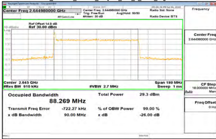
CP-OFDM_Band41_90MHz_64QAM_245_0_Main_HighCH528996
