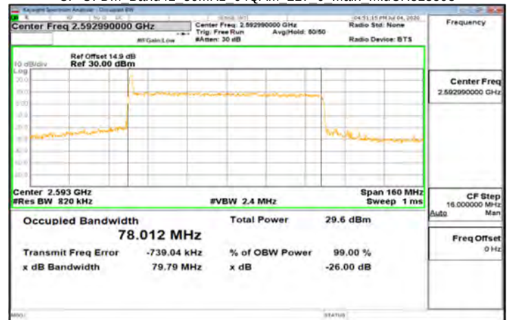
CP-OFDM_Band41_80MHz_64QAM_217_0_Main_MidCH518598
