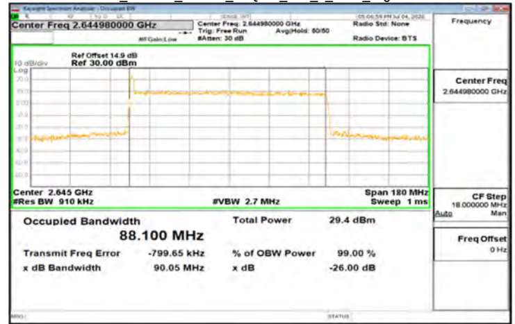
CP-OFDM_Band41_90MHz_16QAM_245_0_Main_HighCH528996
