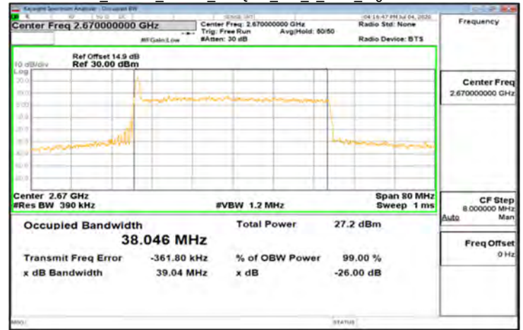
CP-OFDM_Band41_40MHz_256QAM_106_0_Main_HighCH534000-2670
