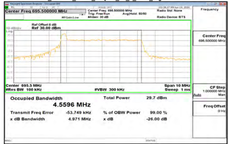
CP-OFDM_Band71_5MHz_16QAM_25_0_Main_HighCH139100-695.5
