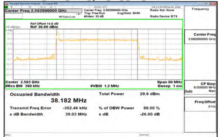
CP-OFDM Band41_40MHz_QPSK_106_0_Main_MidCH518598-2592.99
