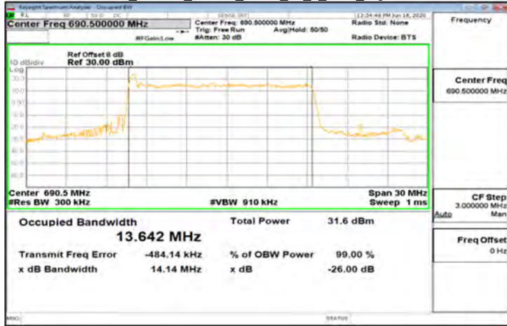
DFT-s-OFDM Pi/2_Band71_15MHz_BPSK_75_0_Main_HighCH138100-690.5
