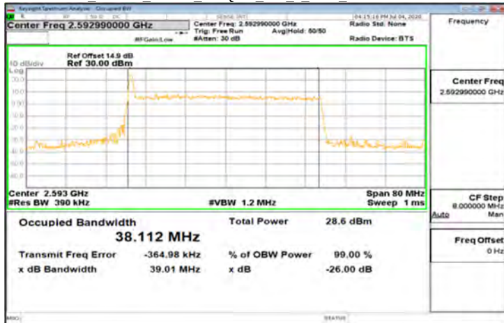
CP-OFDM_Band41_40MHz_256QAM_106_0_Main_MidCH518598-2592.99
