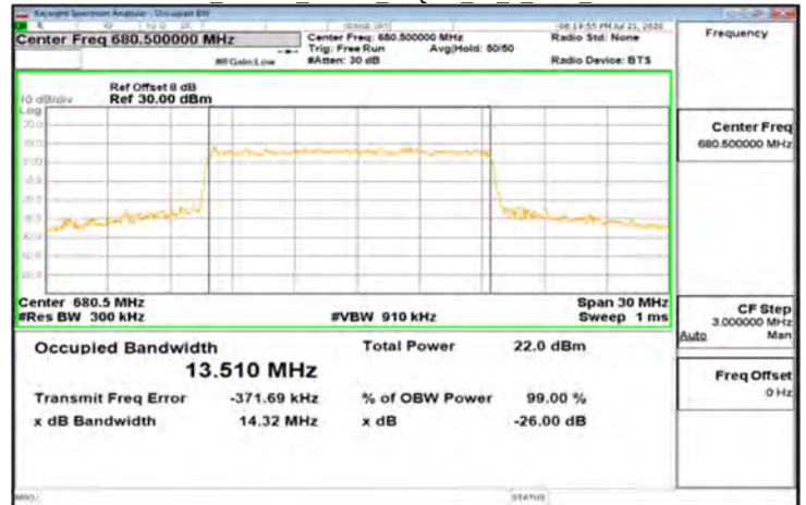
DFT-s-OFDM_Band71_15MHz_16QAM_75_0_Main_MidCH136100
