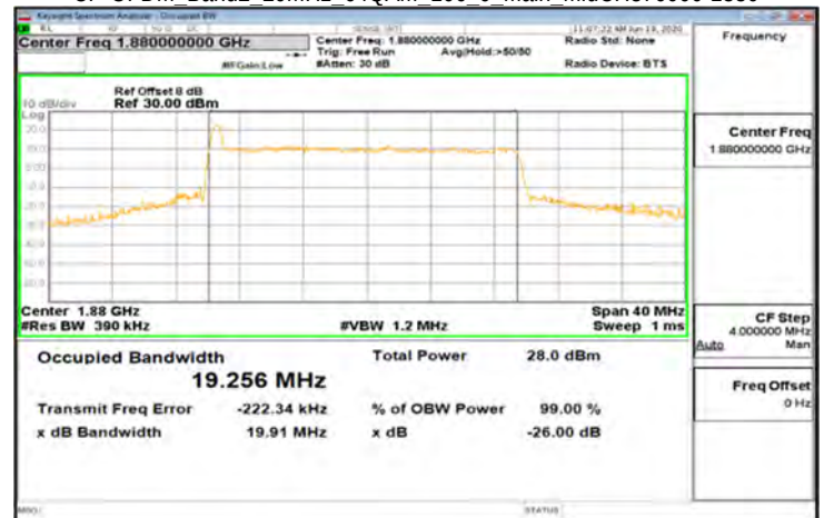
CP-OFDM_Band2_20MHz_64QAM_106_0_Main_MidCH376000-1880
