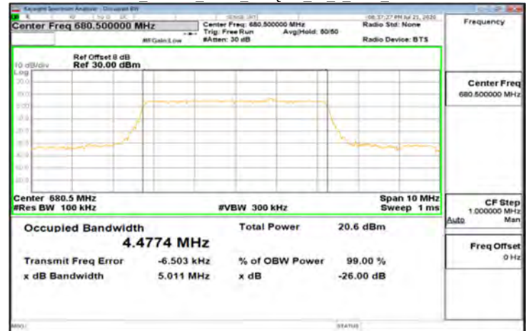
DFT-s-OFDM_Band71_5MHz_256QAM_25_0_Main_MidCH136100
