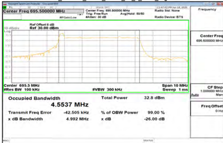
DFT-s-OFDM Pi/2_Band71_5MHz_BPSK_25_0_Main_HighCH139100-695.5
