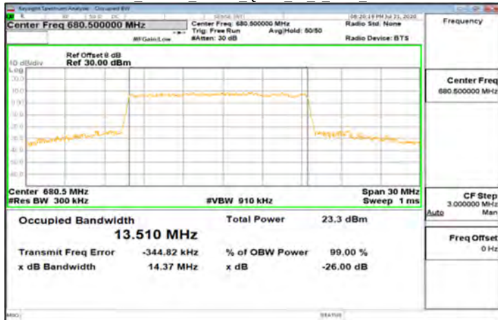
DFT-s-OFDM_Band71_15MHz_QPSK_75_0_Main_MidCH136100
