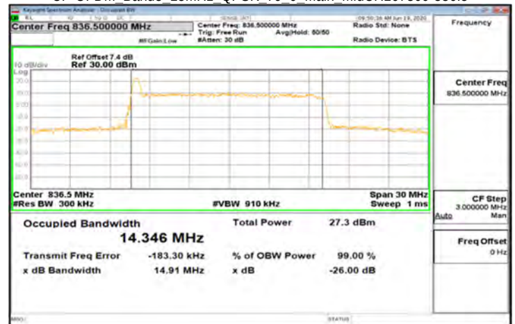
CP-OFDM_Band5_15MHz_QPSK_79_0_Main_MidCH167300-836.5
