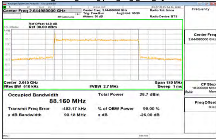
CP-OFDM_Band41_90MHz_QPSK_245_0_Main_HighCH528996
