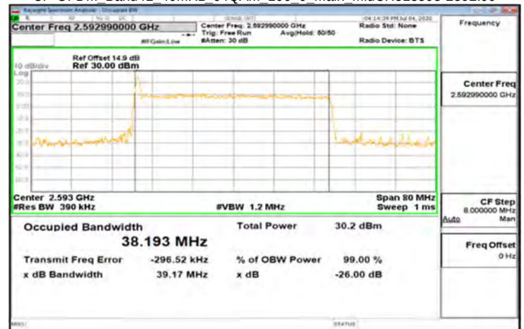
CP-OFDM Band41_40MHz_64QAM_106_0_Main_MidCH518598-2592.99
