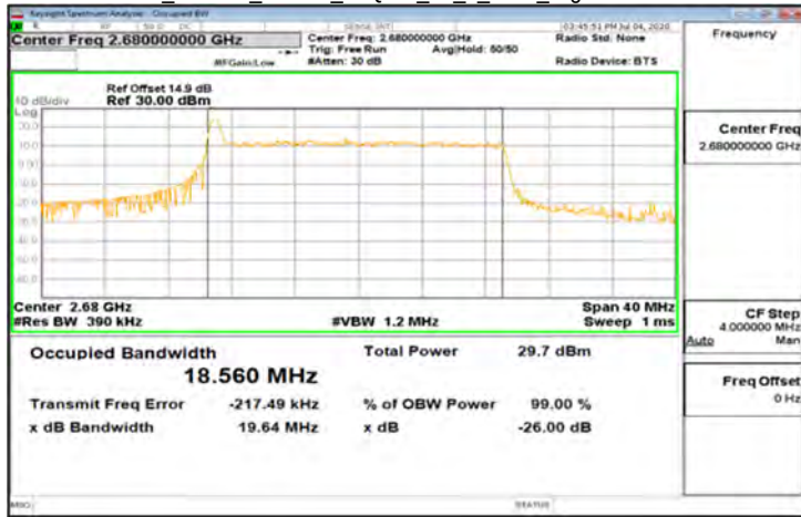
CP-OFDM Band41_20MHz_64QAM_51_0_Main_HighCH535998-2680
