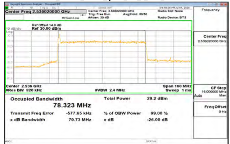
CP-OFDM_Band41_80MHz_QPSK_217_0_Main_MidCH518598
