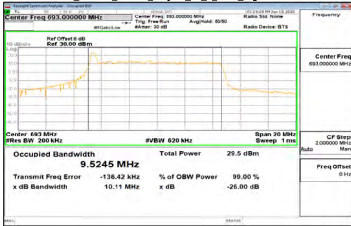
CP-OFDM_Band71_10MHz_64QAM_52_0_Main_HighCH138600-693
