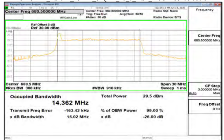
CP-OFDM Band71_15MHz_64QAM_79_0_Main_MidCH136100-680.5
