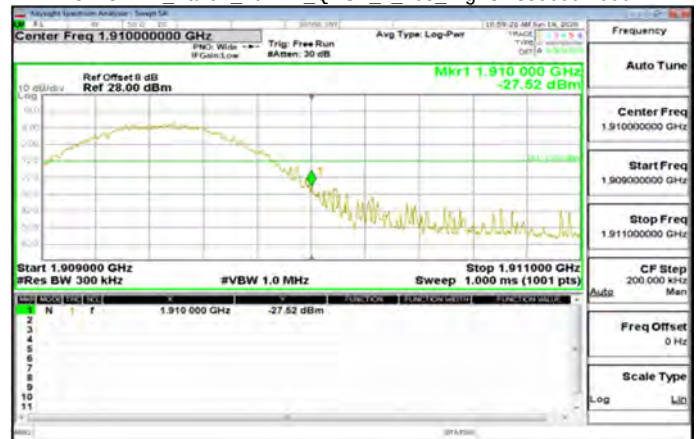
CP-OFDM Band2_20MHz_QPSK_1_105_HighCH380000-1900
