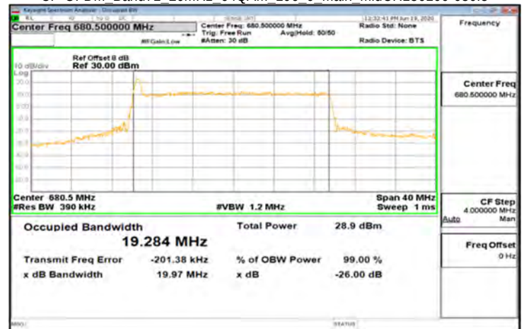
CP-OFDM_Band71_20MHz_64QAM_106_0_Main_MidCH136100-680.5
