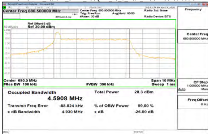
CP-OFDM Band71 5MHz 256QAM 25 0 Main_MidCH136100-680.5
