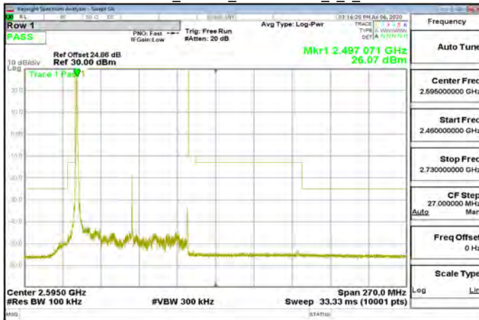
DFT-s-OFDM Pi/2_Band41_80MHz\BPSK_1_0_CH507204
