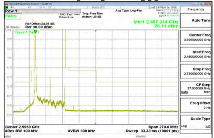
DFT-s-OFDM Pi/2_Band41_50MHz\BPSK_1_0_CH504204
