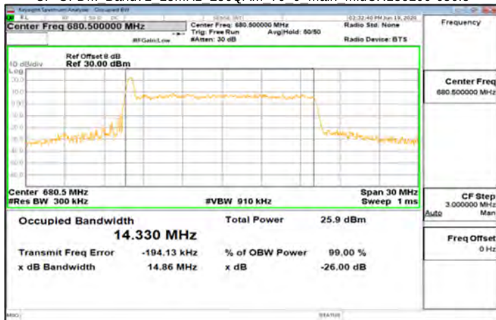
CP-OFDM_Band71_15MHz_256QAM_79_0_Main_MidCH136100-680.5
