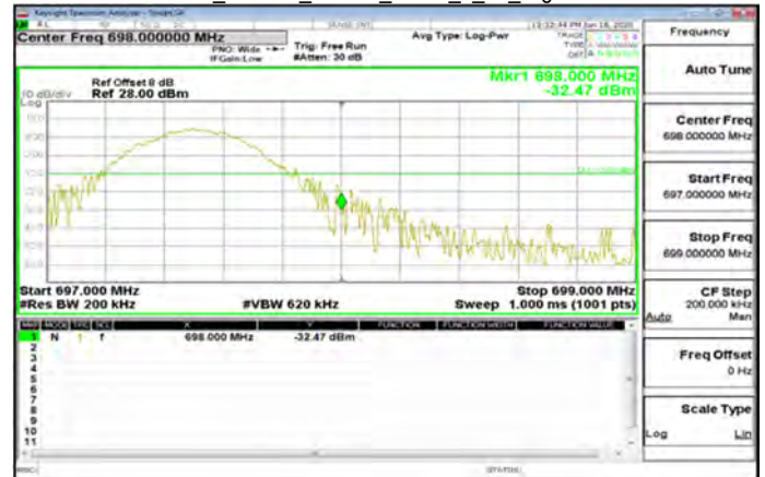
DFT-s-OFDM Pi/2_Band71_15MHz_BPSK_1_78_HighCH138100-690.5
