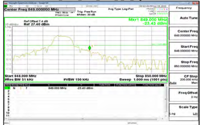
DFT-s-OFDM Pi/2_Band5_5MHz_BPSK_1_24_HighCH169300-846.5
