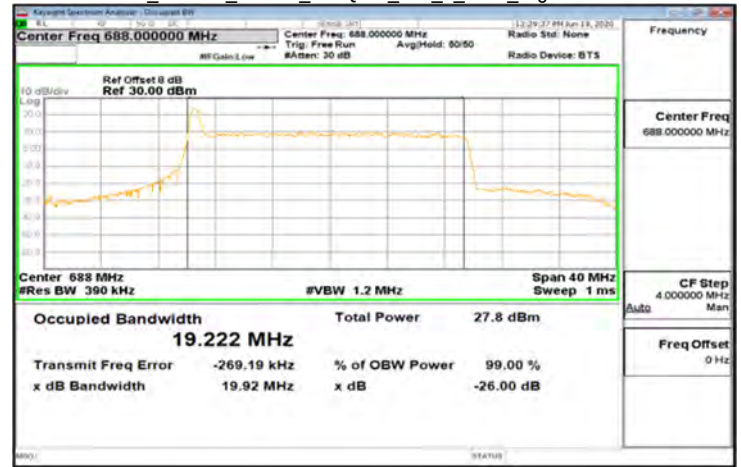
CP-OFDM_Band71_20MHz_256QAM_106_0_Main_HighCH137600-688
