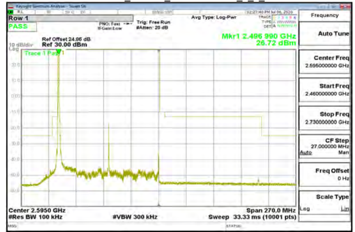
DFT-s-OFDM Pi/2_Band41_100MHz\BPSK_1_0_CH509202
