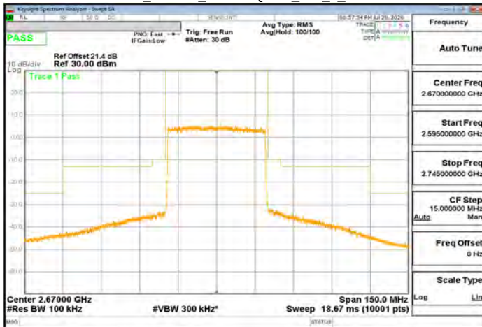
CP-OFDM_Band41_40MHz\QPSK_106_0_CH534000
