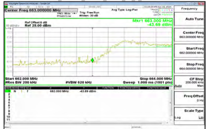
DFT-s-OFDM Pi/2_Band71_15MHz_BPSK_75_0_LowCH134100-670.5
