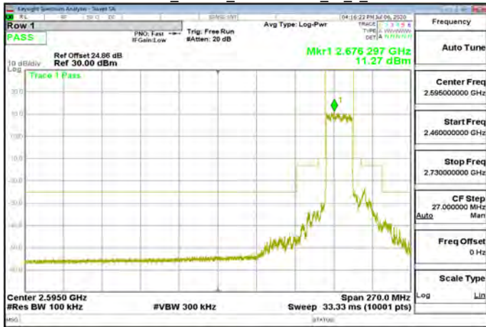
DFT-s-OFDM Pi/2_Band41_20MHz\BPSK_50_0_CH535998
