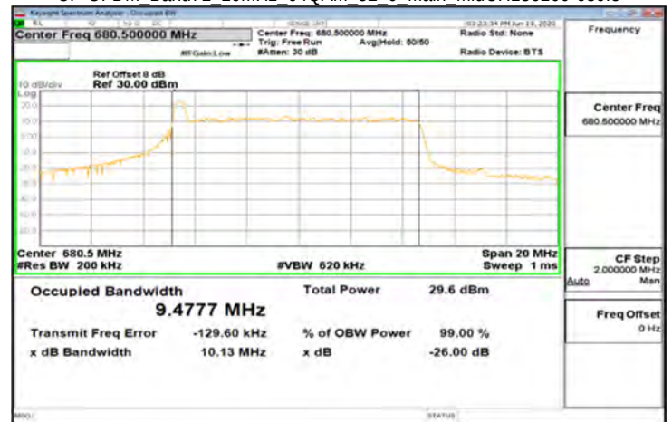
CP-OFDM_Band71_10MHz_64QAM_52_0_Main_MidCH136100-680.5
