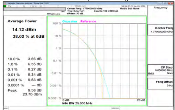
CP-OFDM Band66 20MHz 256QAM 106 0 HighCH354000-1770
