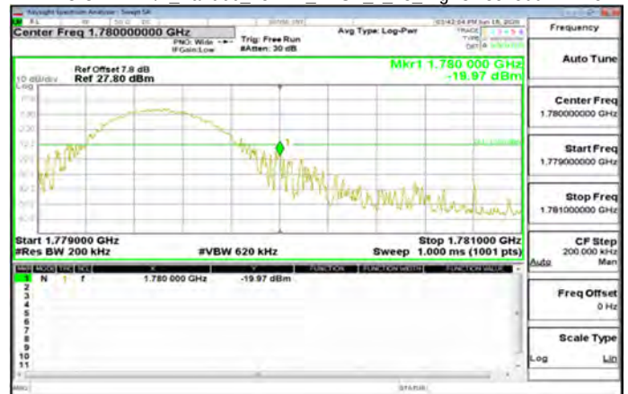
DFT-s-OFDM Pi/2_Band66_15MHz_BPSK_1_78_HighCH354500-1772.5
