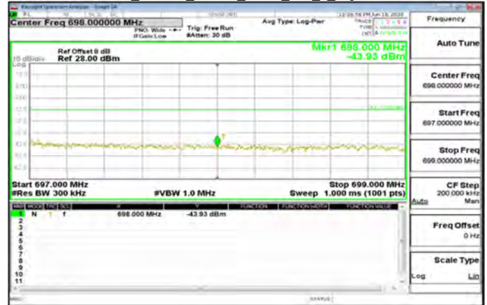
DFT-s-OFDM Pi/2_Band71_20MHz_BPSK_100_0_HighCH137600-688
