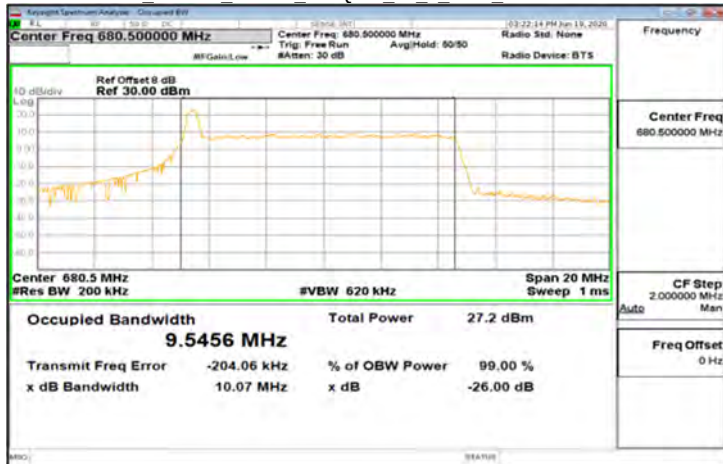
CP-OFDM_Band71_10MHz_256QAM_52_0_Main_MidCH136100-680.5
