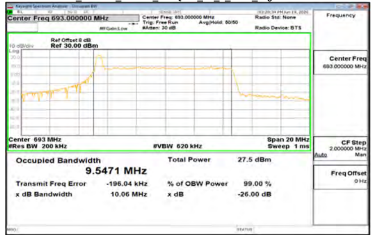
CP-OFDM_Band71_10MHz_256QAM_52_0_Main_HighCH138600-693
