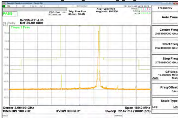
DFT-s-OFDM Pi/2_Band41_50MHz\BPSK_1_132_CH532998
