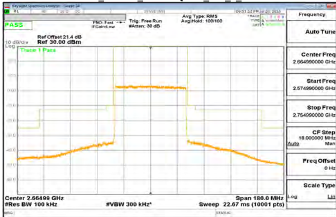
CP-OFDM_Band41_50MHz\QPSK_133_0_CH532998
