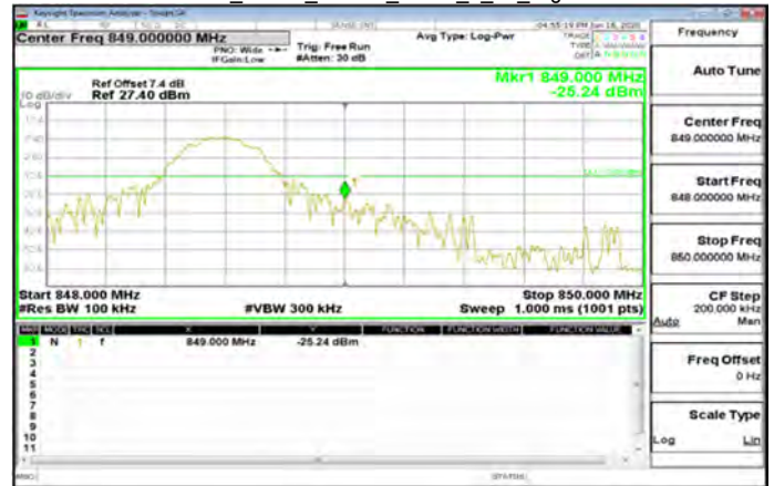
DFT-s-OFDM Pi/2_Band5_10MHz_BPSK_1_51_HighCH168800-844
