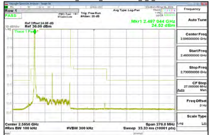
DFT-s-OFDM Pi/2_Band41_60MHz\BPSK_1_0_CH505200
