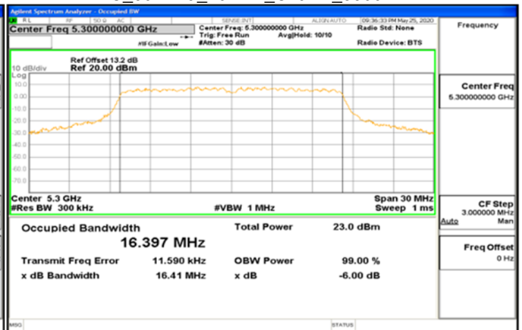
IC_802.11a_20MHz_Chain1_5300MHz
