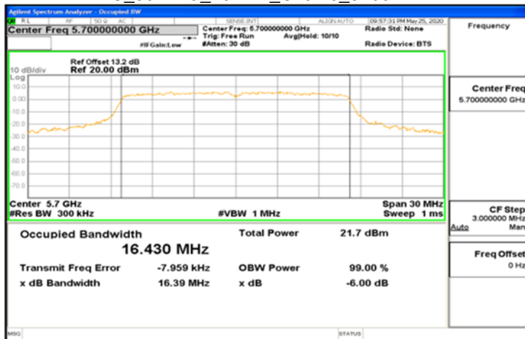
IC_802.11a_20MHz_Chain0_5700MHz
