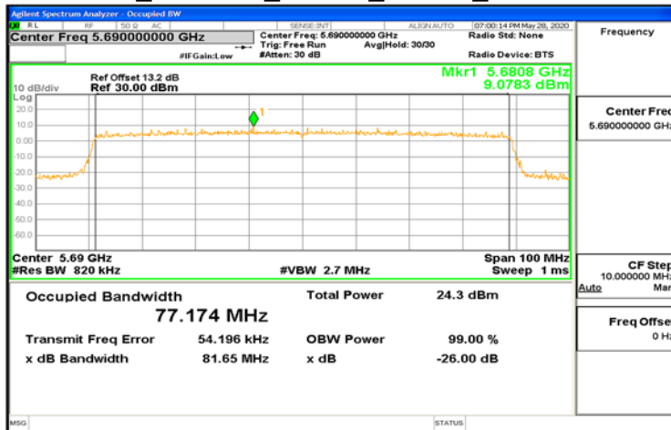
FCC_802.11ax_80MHz_Chain0_5690MHz
