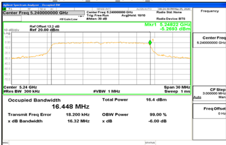
IC_802.11a_20MHz_Chain0_5240MHz
