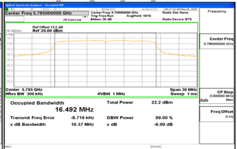
IC_802.11a_20MHz_Chain0_5785MHz
