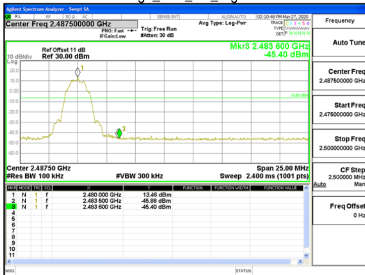
BLE\Band Edge_BLE_2M_HighCH39-2480
