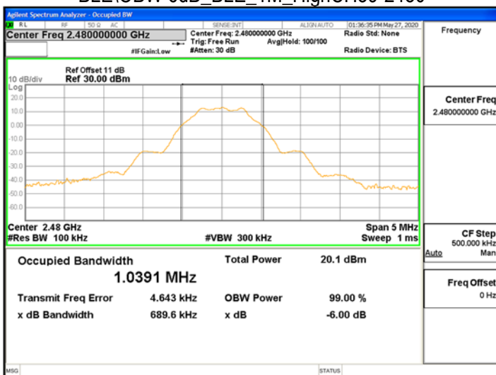
BLE\OBW 6dB_BLE_1M_HighCH39-2480
