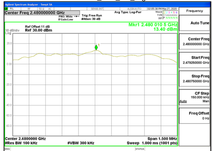
BLE\Reference Level_BLE_2M_HighCH39-2480
