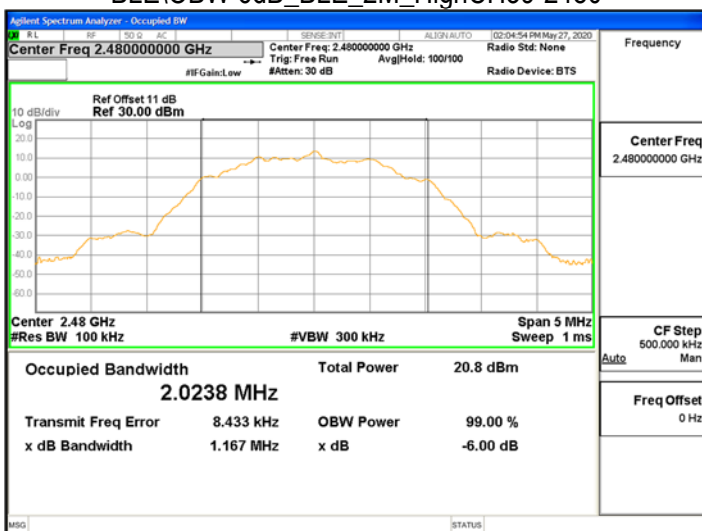
BLE\OBW 6dB_BLE_2M_HighCH39-2480
