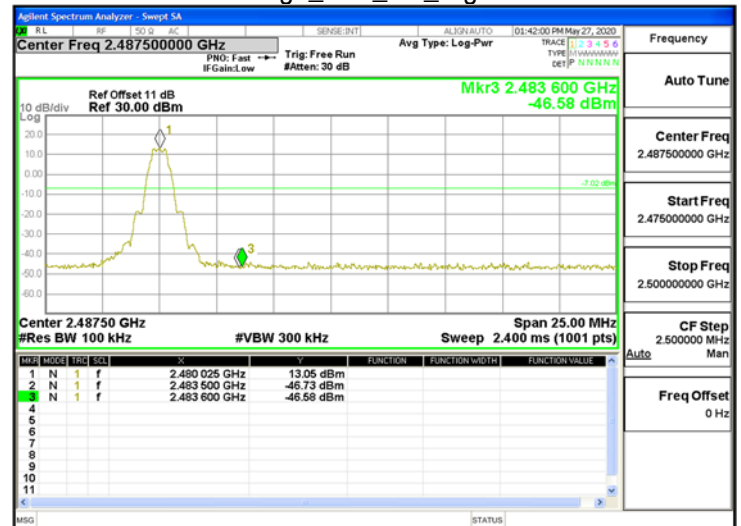
BLE\Band Edge_BLE_1M_HighCH39-2480
