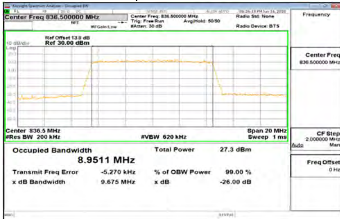
Band26 10MHz_256QAM_50_0_Main_MidCH26915-836.5
