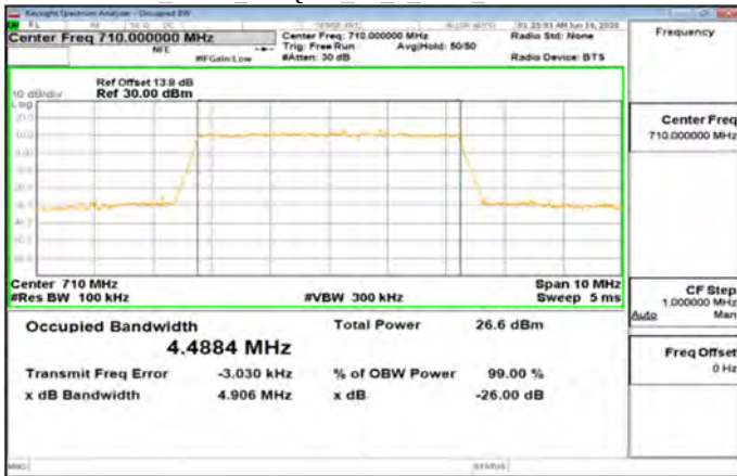
Band17 5MHz_256QAM_25_0_Main_MidCH23790-710
