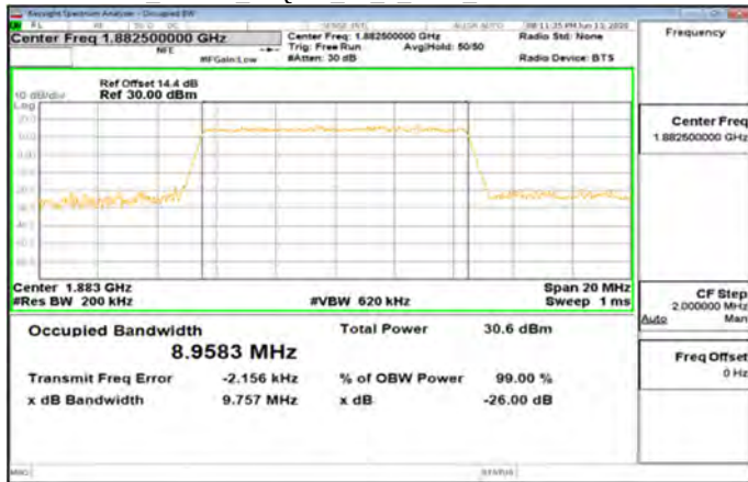
Band25_10MHz_16QAM_50_0_Main_MidCH26365-1882.5
