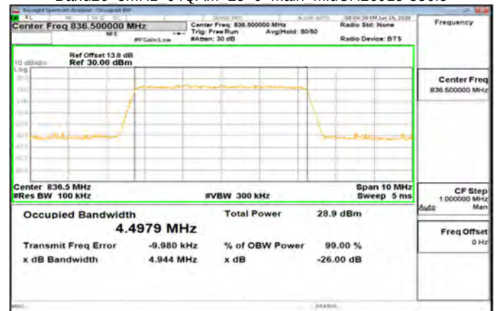
Band26_5MHz_64QAM_25_0_Main_MidCH26915-836.5
