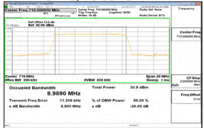
Band17 10MHz_QPSK_50_0_Main_MidCH23790-710
