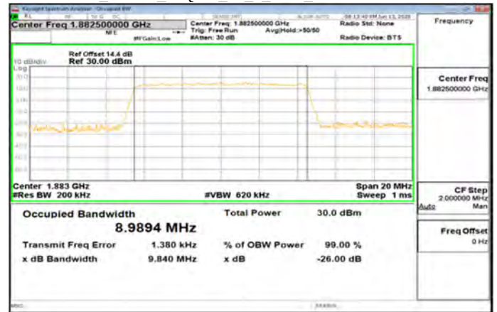
Band25_10MHz_64QAM_50_0_Main_MidCH26365-1882.5
