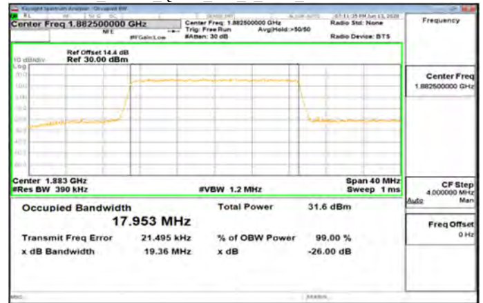
Band25 20MHz_QPSK_100_0_Main_MidCH26365-1882.5
