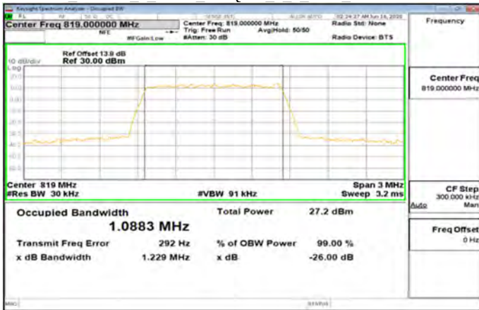
Band26_Part90s_1_4MHz_256QAM_6_0_Main_MidCH26740-819
