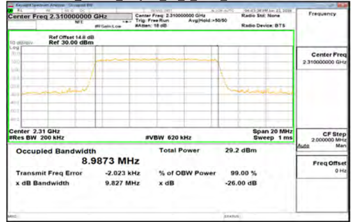
Band30 10MHz_256QAM_50_0_Main_MidCH27710-2310
