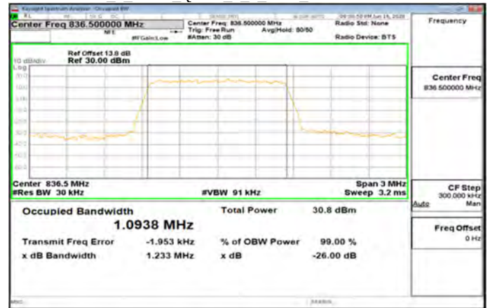
Band26 1 4MHz_QPSK_6_0_Main_MidCH26915-836.5
