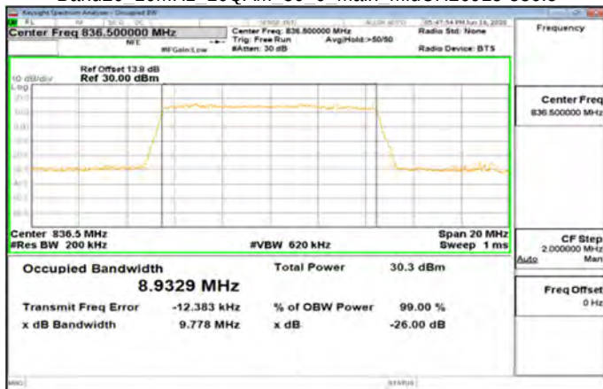
Band26 10MHz_16QAM_50_0_Main_MidCH26915-836.5
