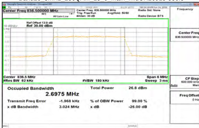
Band26 3MHz_256QAM_15_0_Main_MidCH26915-836.5
