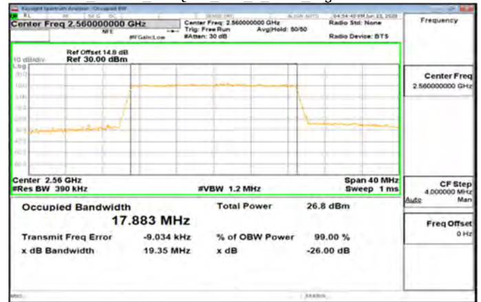
Band7 20MHz_256QAM_100_0_Main_HighCH21350-2560
