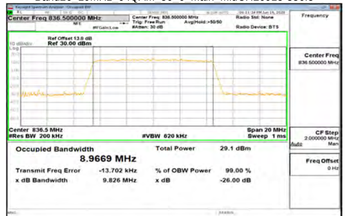
Band26 10MHz_64QAM_50_0_Main_MidCH26915-836.5
