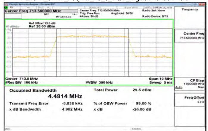
Band12_5MHz_16QAM_25_0_Main_HighCH23155-713.5
