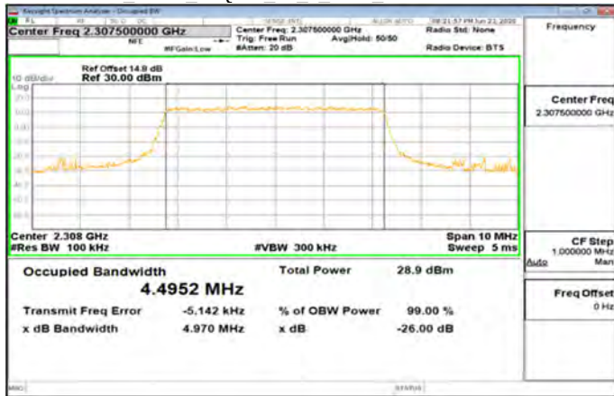
Band30_5MHz_64QAM_25_0_Main_LowCH27685-2307.5
