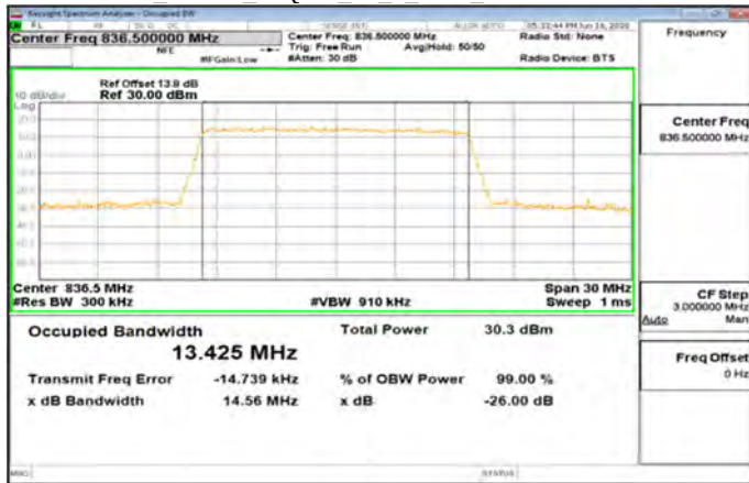
Band26 15MHz_16QAM_75_0_Main_MidCH26915-836.5
