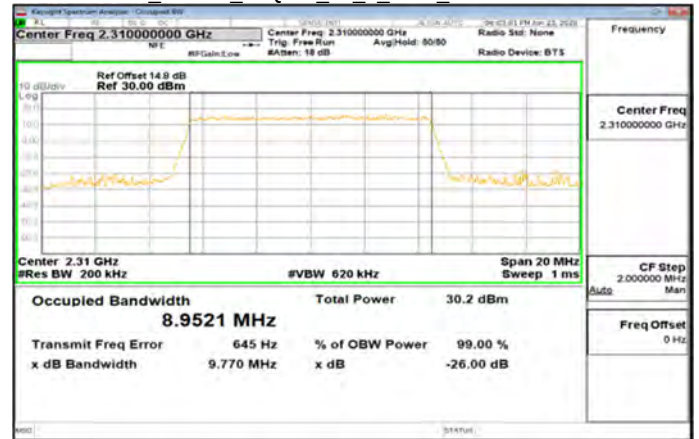
Band30 10MHz_64QAM_50_0_Main_MidCH27710-2310
