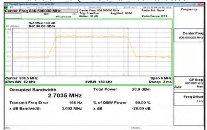
Band26_3MHz_64QAM_15_0_Main_MidCH26915-836.5
