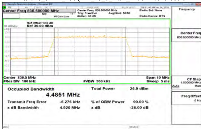
Band26 5MHz_256QAM_25_0_Main_MidCH26915-836.5
