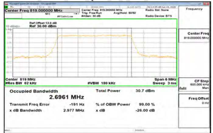
Band26_Part90s_3MHz_QPSK_15_0_Main_MidCH26740-819
