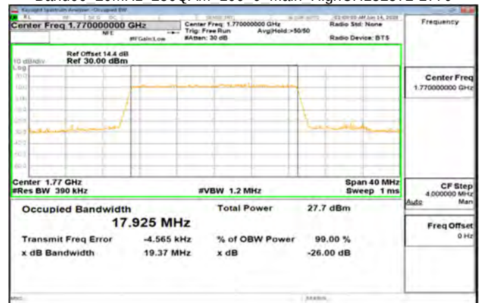
Band66 20MHz_256QAM_100_0_Main_HighCH132572-1770
