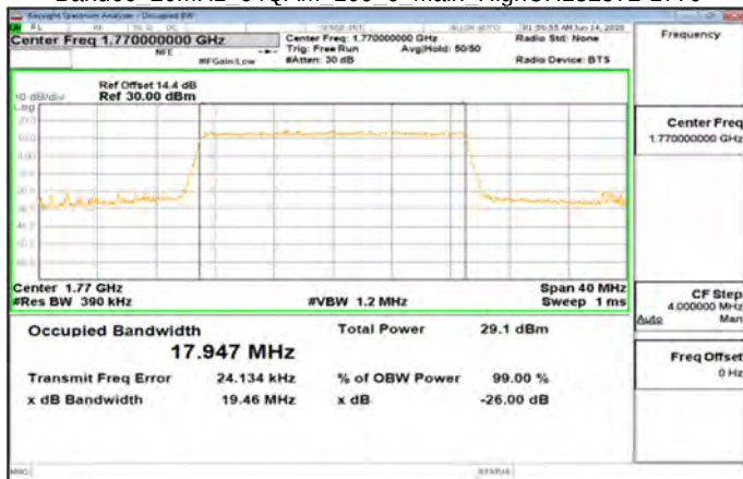
Band66 20MHz_64QAM_100_0_Main_HighCH132572-1770
